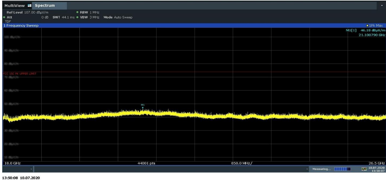
Plot 7-32. Radiated Spurious Emissions 18-26.5GHz (4Mbps, ePA – Ch.38, Ant. Pol. H)
