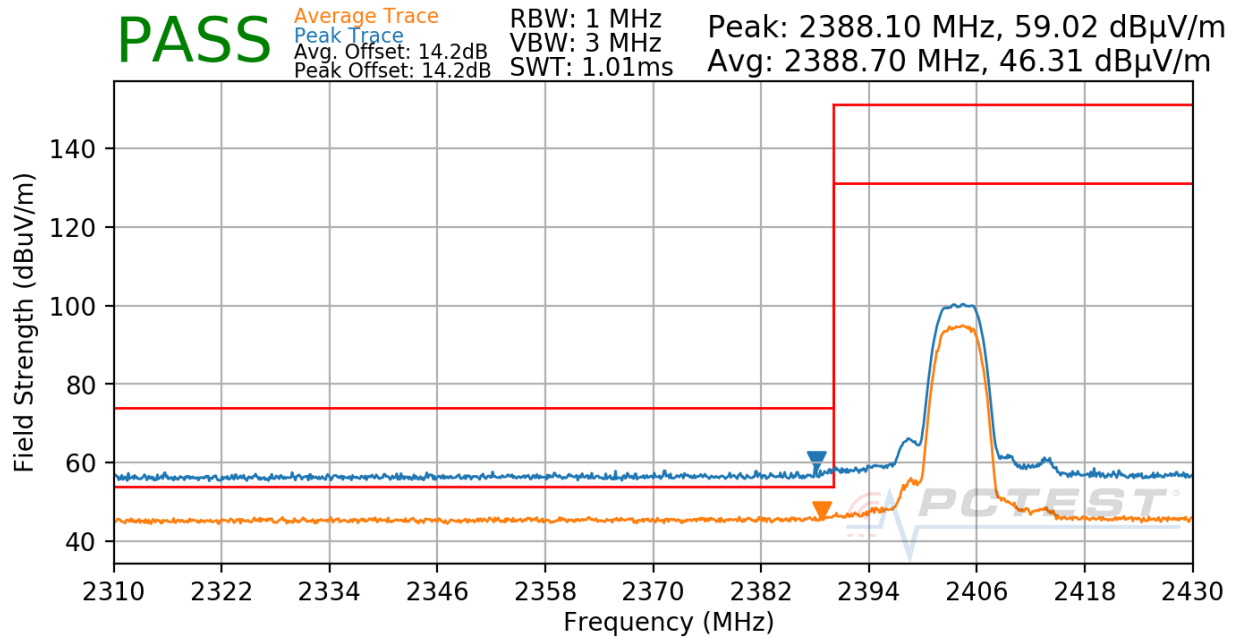
Plot 7-35. Radiated Restricted Lower Band Edge Measurement
