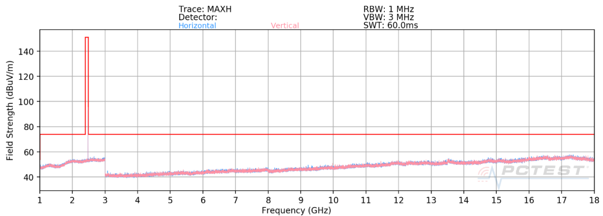
Plot 7-31. Radiated Spurious Emissions 1-18GHz (4Mbps, ePA – Ch. 75)
