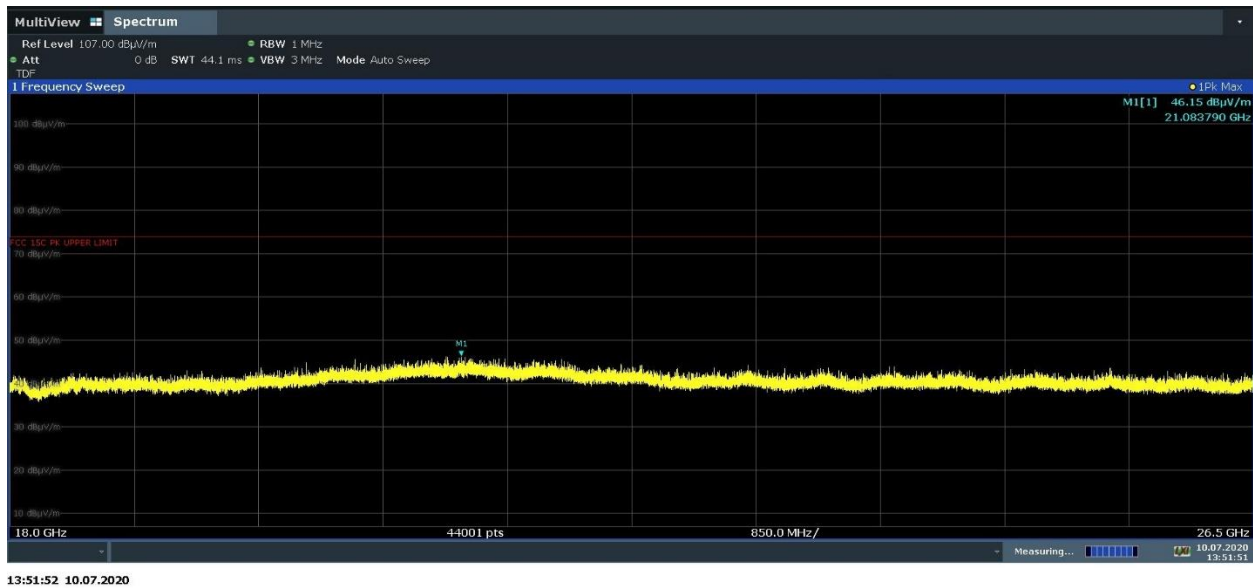
Plot 7-33. Radiated Spurious Emissions 18-26.5GHz (4Mbps, ePA – Ch.38, Ant. Pol. V)
