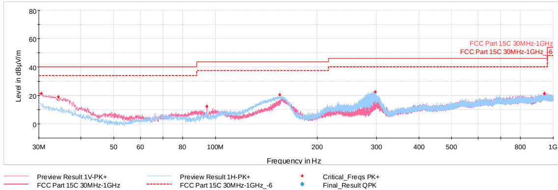
Plot 7-38. Radiated Spurious Emissions 30MHz-1GHz (1Mbps, ePA – Ch.19, with WCP + AC/DC adapter)
