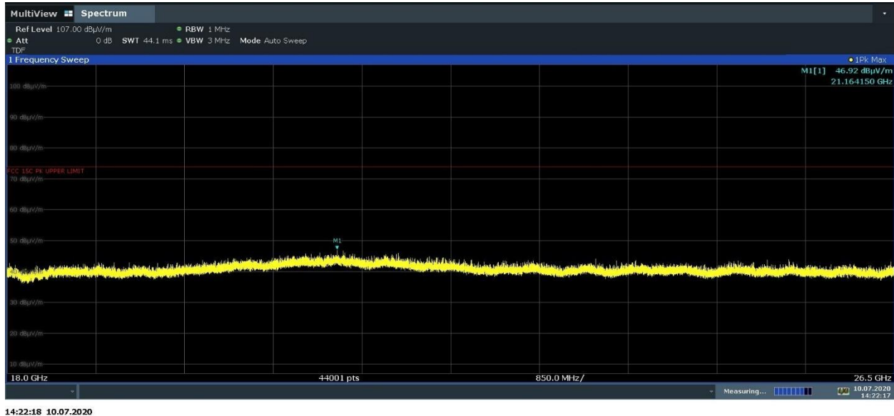
Plot 7-43. Radiated Spurious Emissions 18-26.5GHz (802.11b – Ch. 6, Ant. Pol. H)
