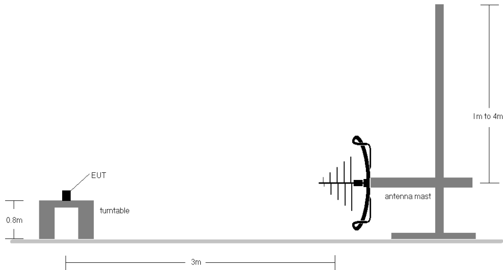
Figure 7-5. Radiated Measurement Setup < 1GHz
