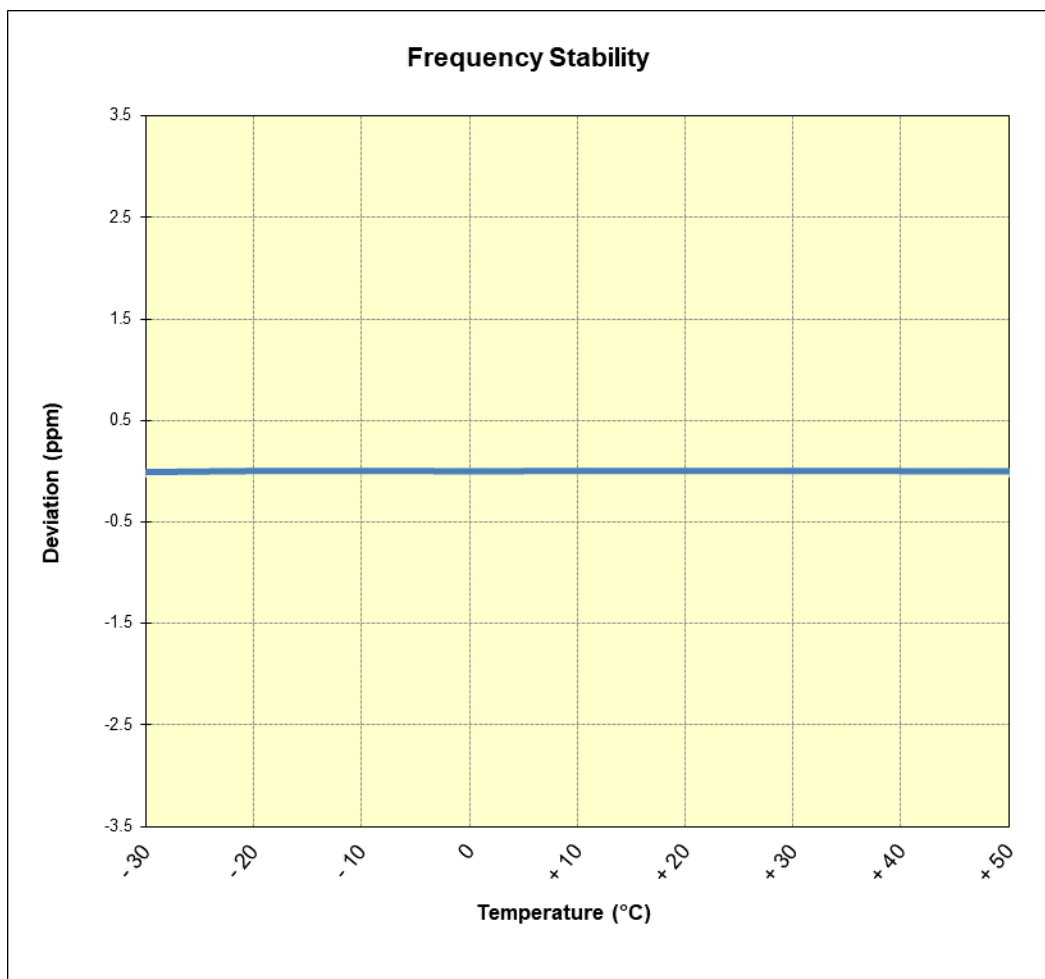
Figure 7-8. LTE Band 26 Frequency Stability Chart – 10MHz QPSK Full RB Configuration
