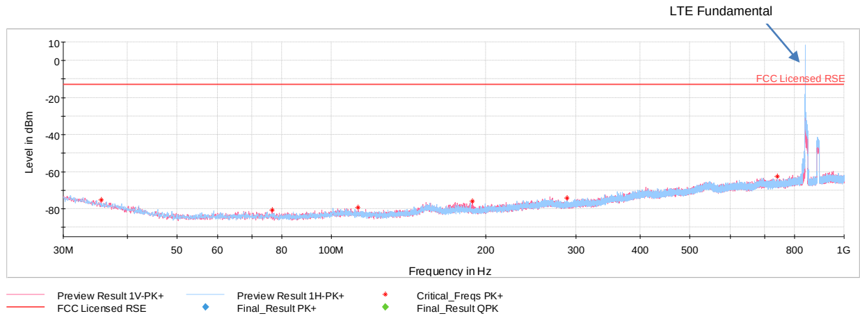
Plot 7-22. Radiated Spurious Emissions Below 1GHz (Band 26)
