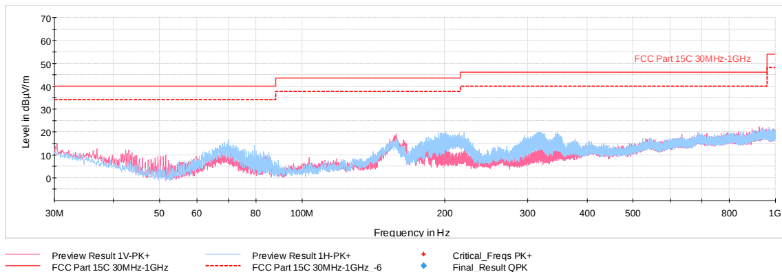
Plot 7-57. Radiated Spurious Emissions 30MHz-1GHz (802.11b – Ch.6, with WCP + laptop)
