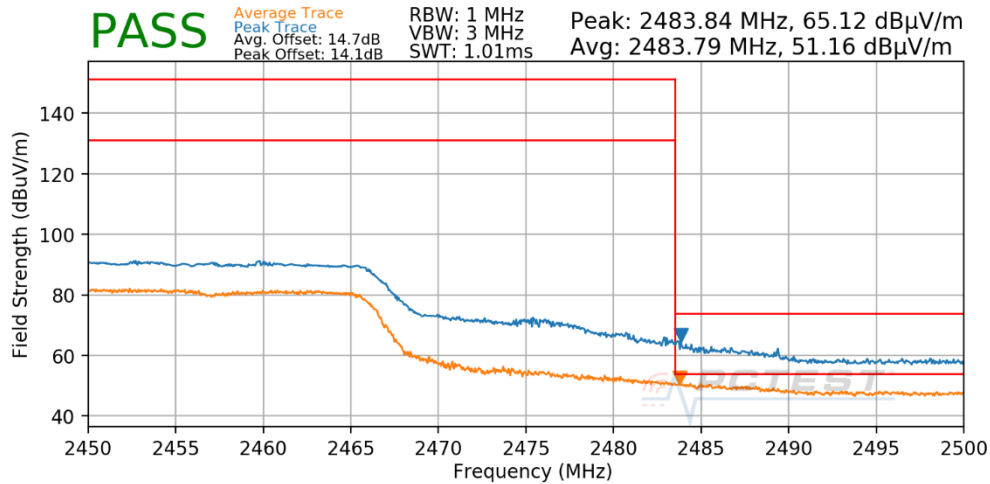
Plot 7-53. Radiated Restricted Upper Band Edge Measurement
