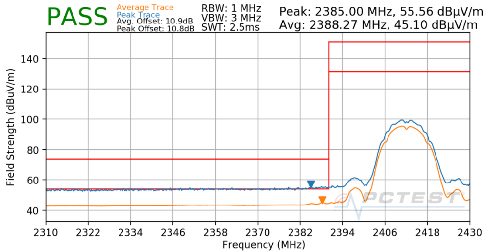
Plot 7-48. Radiated Restricted Lower Band Edge Measurement
