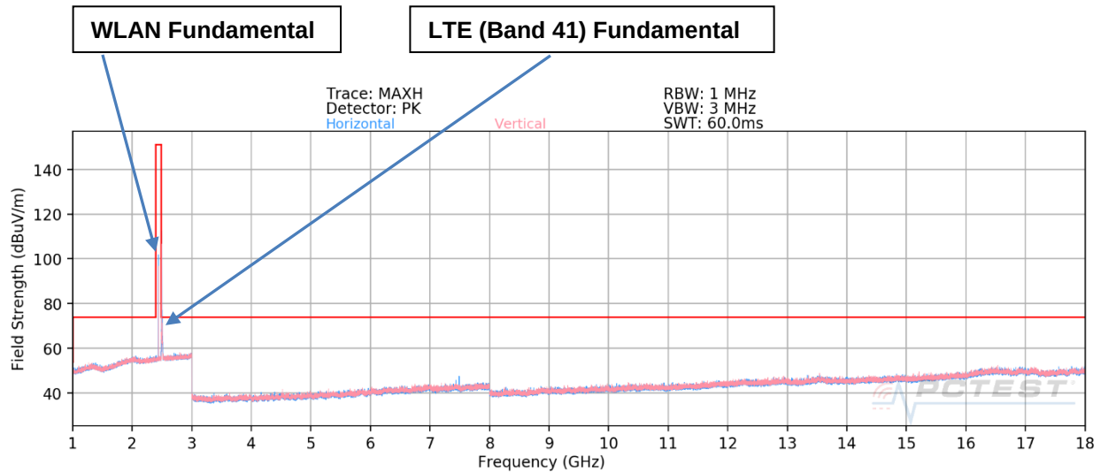
Plot 7-45. Radiated Spurious Emissions 1-18GHz (Simultaneous Transmission)
