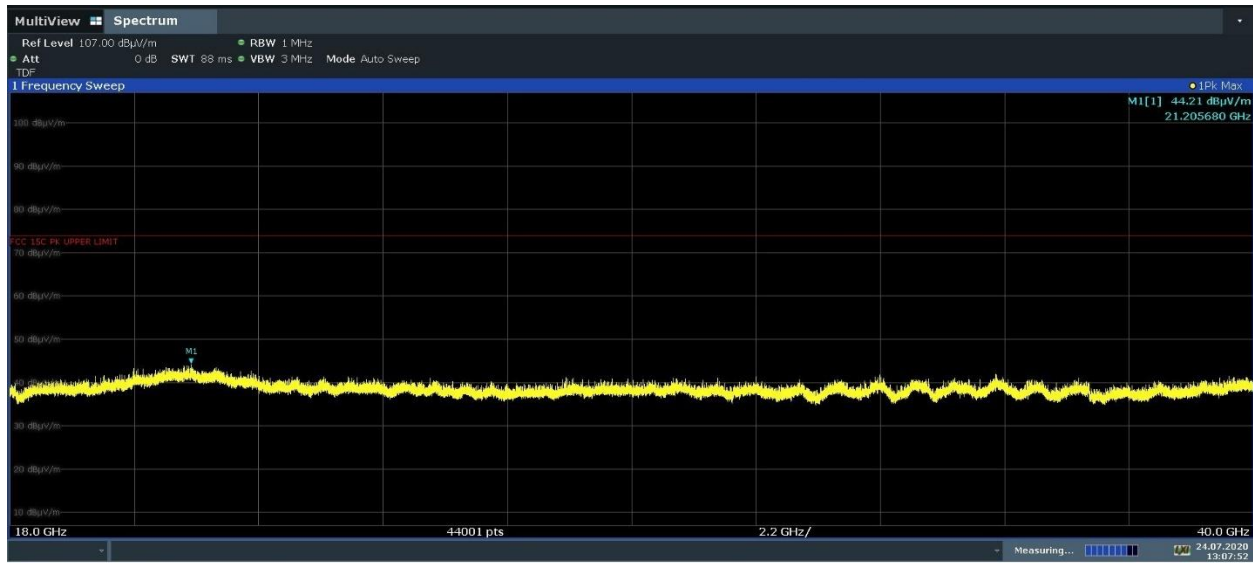
Plot 7-46. Radiated Spurious Emissions 18-40GHz (Simultaneous Transmission, Ant. Pol. H)
