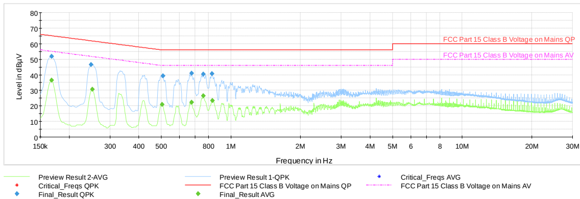
Plot 7-59. AC Line Conducted Emission with 802.11b Ch.6 (L1, with WCP + AC/DC Adapter)
