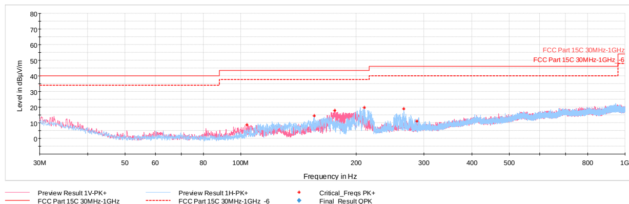
Plot 7-58. Radiated Spurious Emissions 30MHz-1GHz (Simultaneous Transmission, with WCP + AC/DC adapter)
