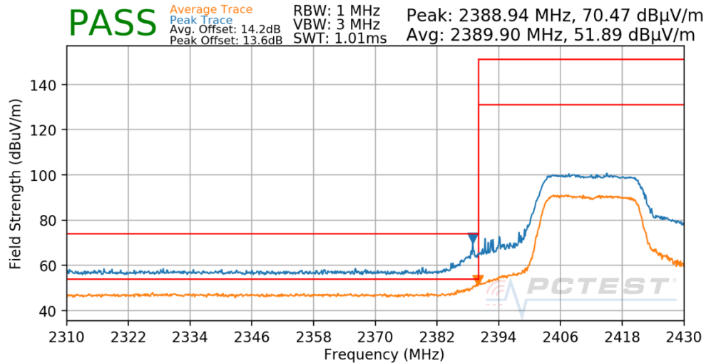
Plot 7-51. Radiated Restricted Lower Band Edge Measurement
