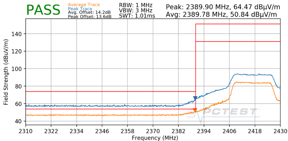
Plot 7-52. Radiated Restricted Lower Band Edge Measurement
