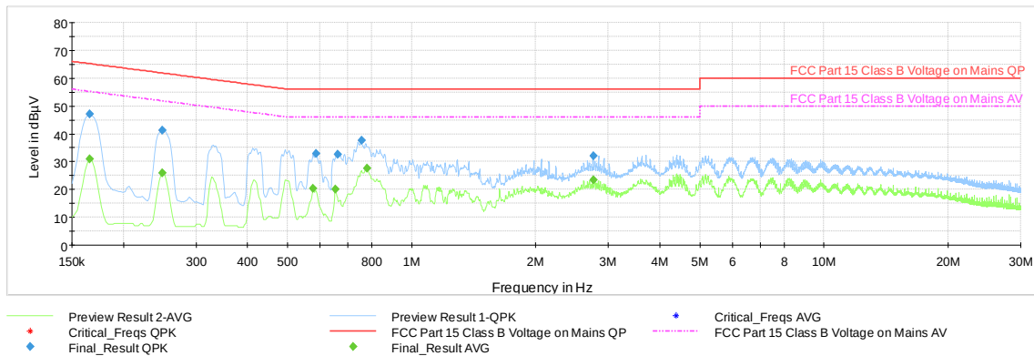
Plot 7-60. AC Line Conducted Emission with 802.11b Ch.6 (N, with WCP + AC/DC Adapter)
