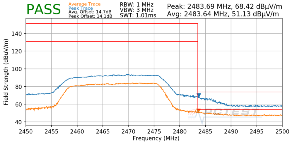
Plot 7-55. Radiated Restricted Upper Band Edge Measurement
