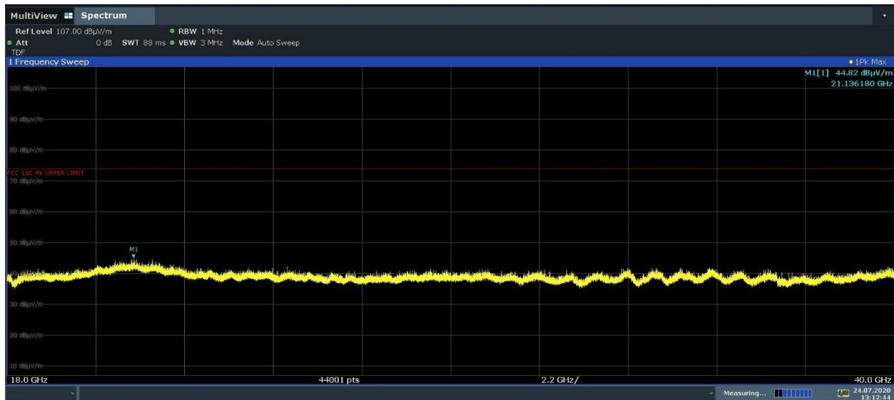
Plot 7-47. Radiated Spurious Emissions 18-40GHz (Simultaneous Transmission, Ant. Pol. V)
