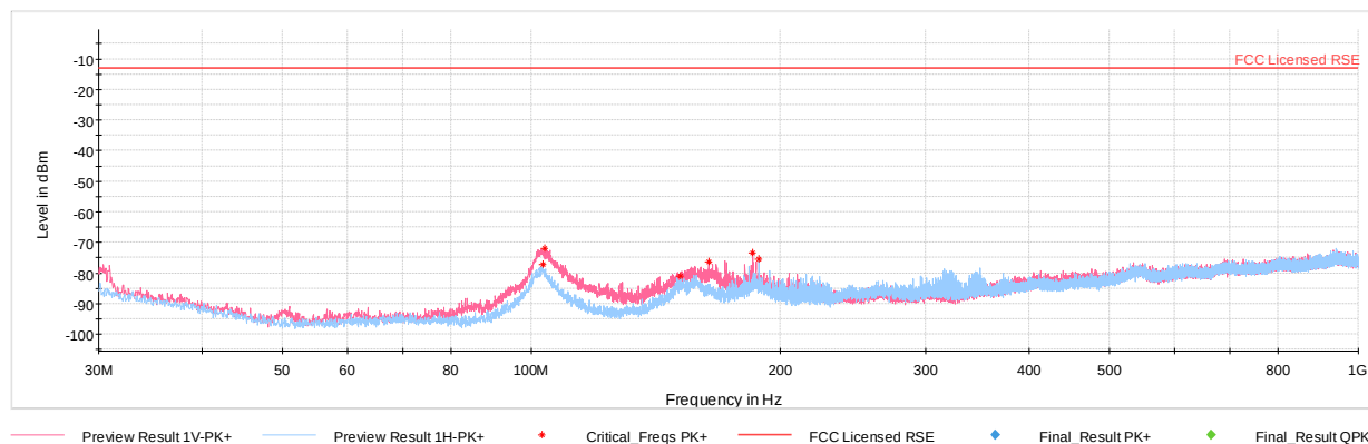
Plot 7-280. Radiated Spurious Emissions – Simultaneous Transmission 30MHz – 1GHz
