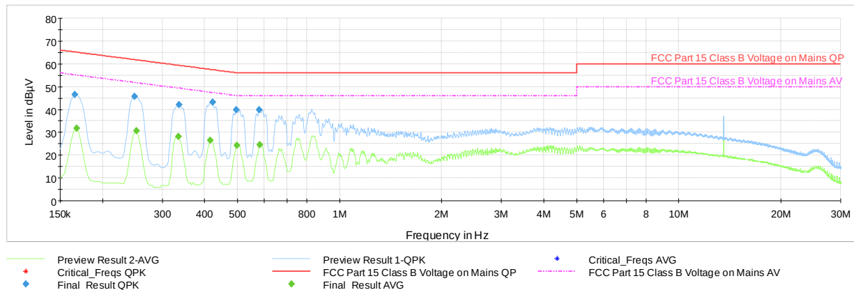
Plot 7-12. AC Line-Conducted Test Plot (L1, CE B 848kbps, with WCP + AC/DC Adapter)
