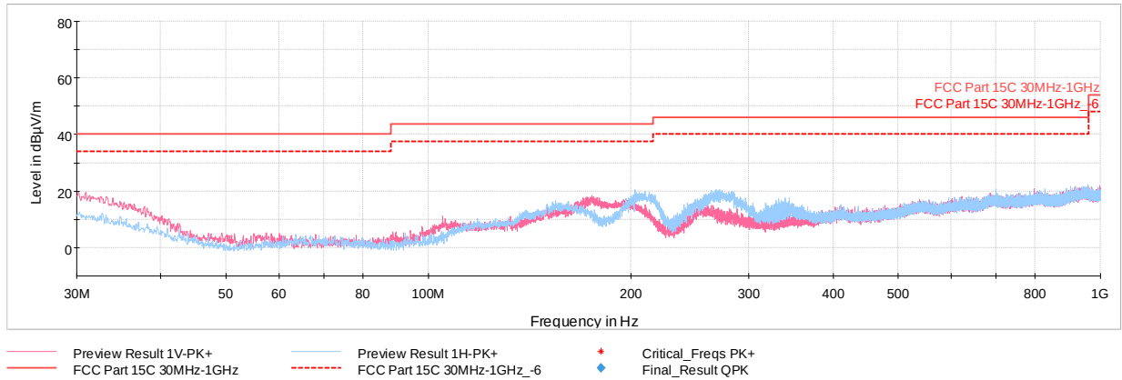
Plot 7-10. Radiated Spurious Emissions 30MHz – 1GHz (CE B 848kbps, with WCP + AC/DC Adapter)
