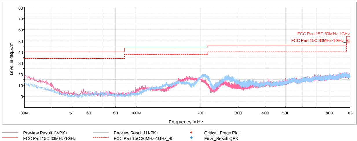
Plot 7-11. Radiated Spurious Emissions 30MHz – 1GHz (Reader 10% Ask 1 out of 4, with WCP + AC/DC Adapter)
