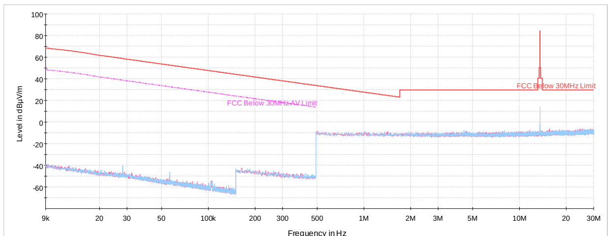
Plot 7-9. Radiated Spurious Emissions 9kHz – 30MHz (Reader 10% Ask 1 out of 4, with WCP + AC/DC Adapter)
