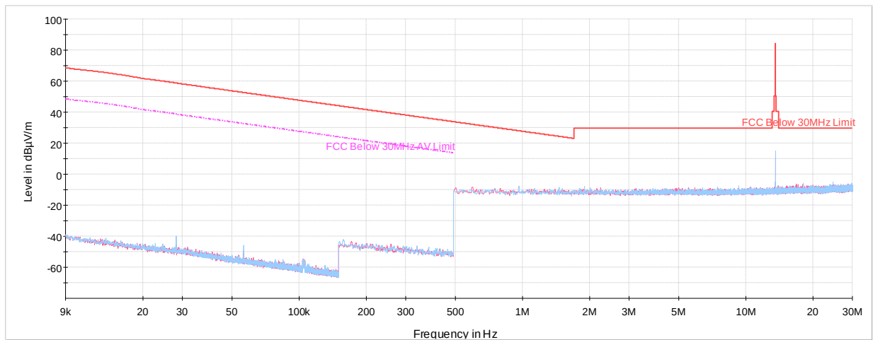
Plot 7-8. Radiated Spurious Emissions 9kHz – 30MHz (CE B 848kbps, with WCP + AC/DC Adapter)
