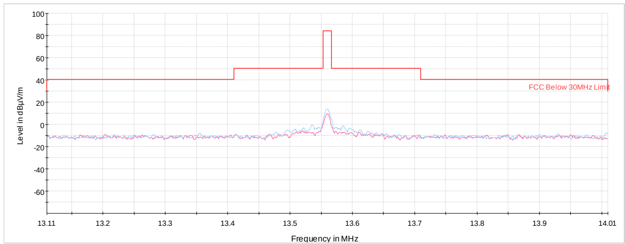
Plot 7-7. In Band Radiated Spurious Emissions (Reader 10% Ask 1 out of 4, with WCP + AC/DC Adapter)
