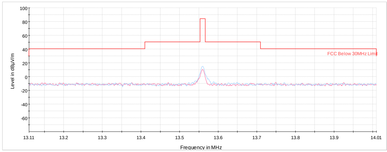
Plot 7-6. In Band Radiated Spurious Emissions (CE B 848kbps, with WCP + AC/DC Adapter)
