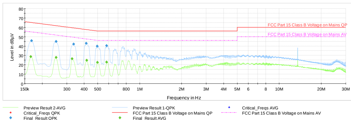
Plot 7-13. AC Line-Conducted Test Plot (N, CE B 848kbps, with WCP + AC/DC Adapter)
