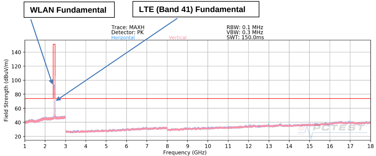
Plot 7-45. Radiated Spurious Emissions 1-18GHz (Simultaneous Transmission)
