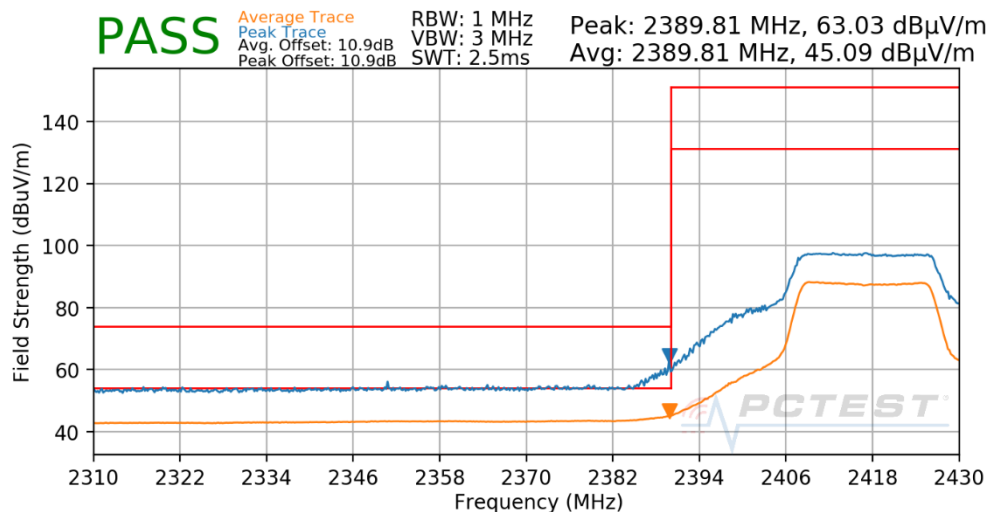
Plot 7-52. Radiated Restricted Lower Band Edge Measurement
