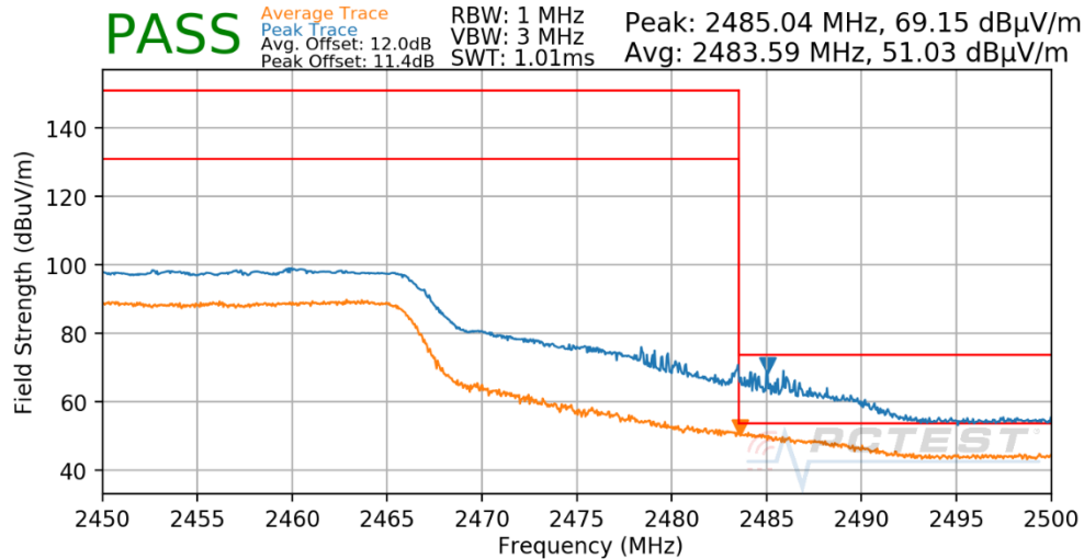
Plot 7-53. Radiated Restricted Upper Band Edge Measurement
