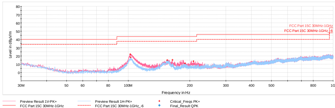
Plot 7-58. Radiated Spurious Emissions 30MHz-1GHz (Simultaneous Transmission, with WCP + laptop)
