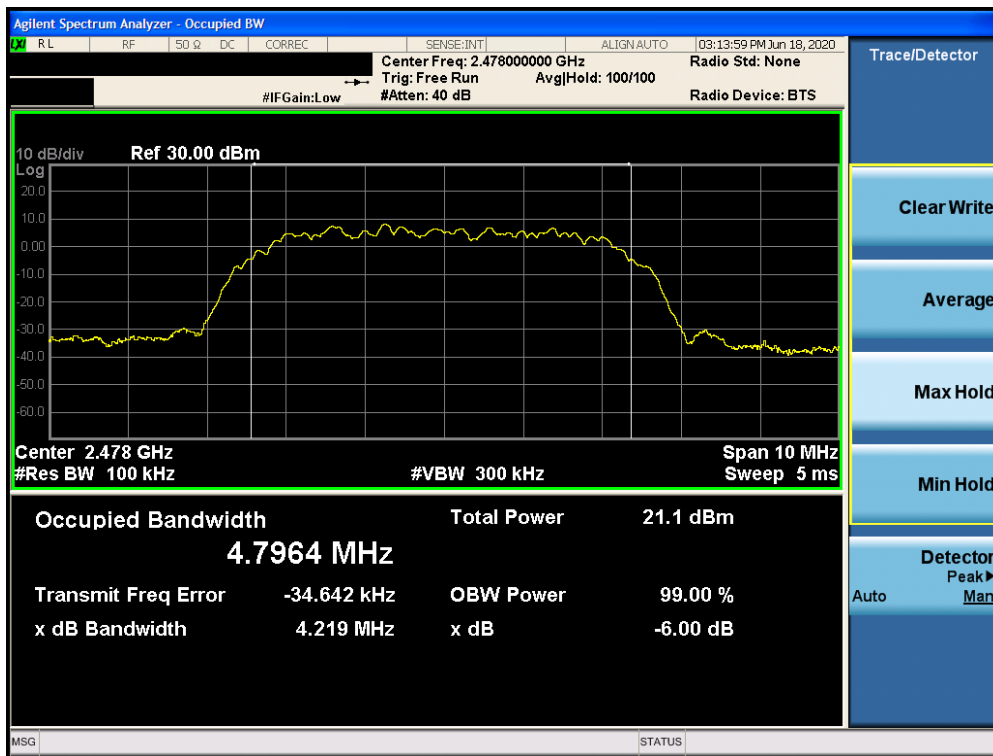
Plot 7-6. 6dB Bandwidth Plot (Bluetooth (HDR8), 8Mbps, ePA – Ch. 75)
