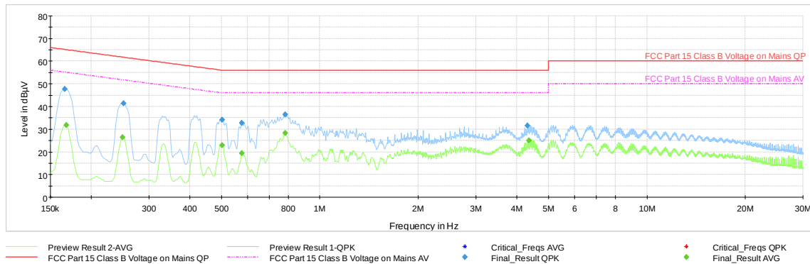
Plot 7-40. AC Line Conducted Plot with Bluetooth HDR (N – 4Mbps, ePA, Ch. 38 with WCP + AC/DC Adapter)
