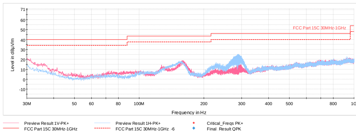
Plot 7-38. Radiated Spurious Emissions 30MHz-1GHz (4Mbps, ePA – Ch.38 with WCP + AC/DC Adapter)
