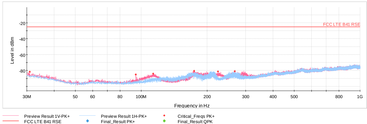
Plot 7-272. Radiated Spurious Emissions – Simultaneous Transmission 30MHz – 1GHz
