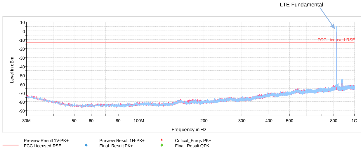
Plot 7-22. Radiated Spurious Emissions Below 1GHz (Band 26)
