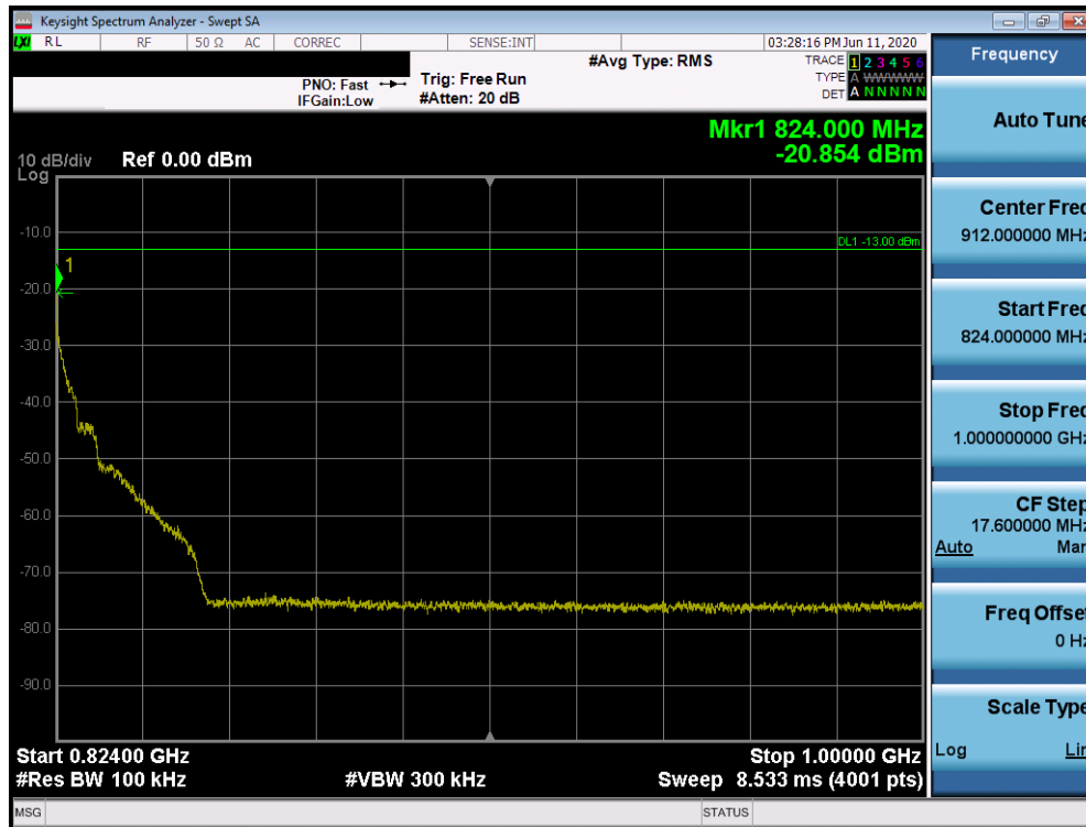
Plot 7-13. Conducted Spurious Plot (LTE Band 26 - 5MHz QPSK - RB Size 1, RB Offset 0 - High Channel)
