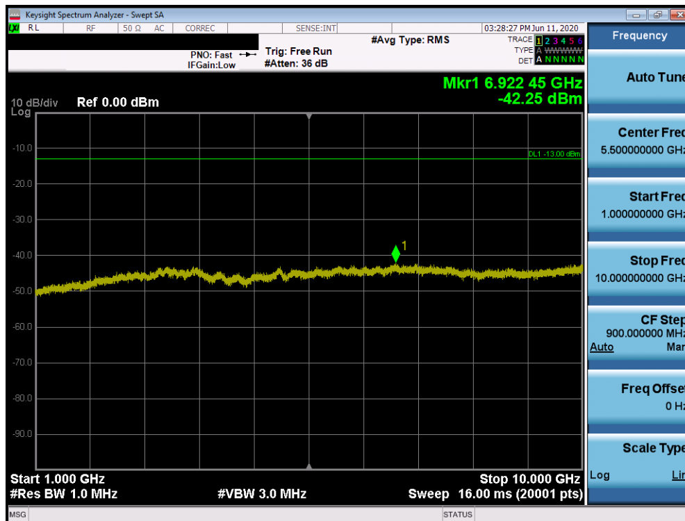
Plot 7-14. Conducted Spurious Plot (LTE Band 26 - 5MHz QPSK - RB Size 1, RB Offset 0 - High Channel)
