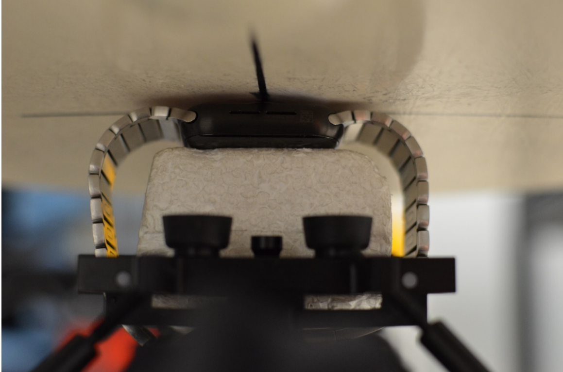
SAR Test Setup Photo 17: Titanium with Metal Links Wristband, Back side at 0.0 cm
