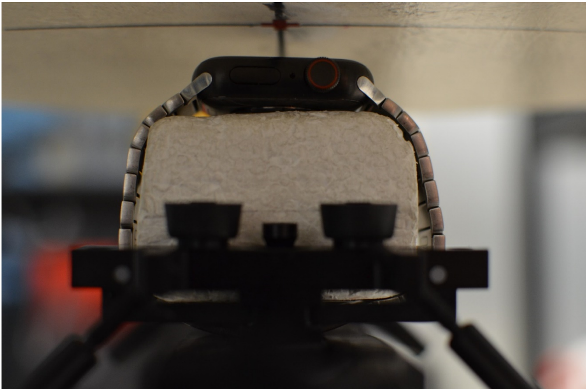
SAR Test Setup Photo 8: Titanium with Metal Links Wristband, Front side at 1.0 cm
