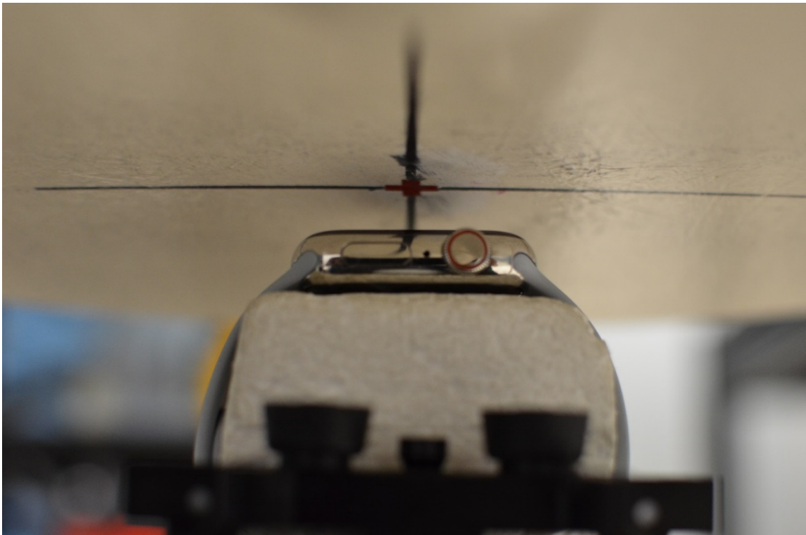
SAR Test Setup Photo 4: Stainless Steel with Sport Wristband, Front side at 1.0 cm
