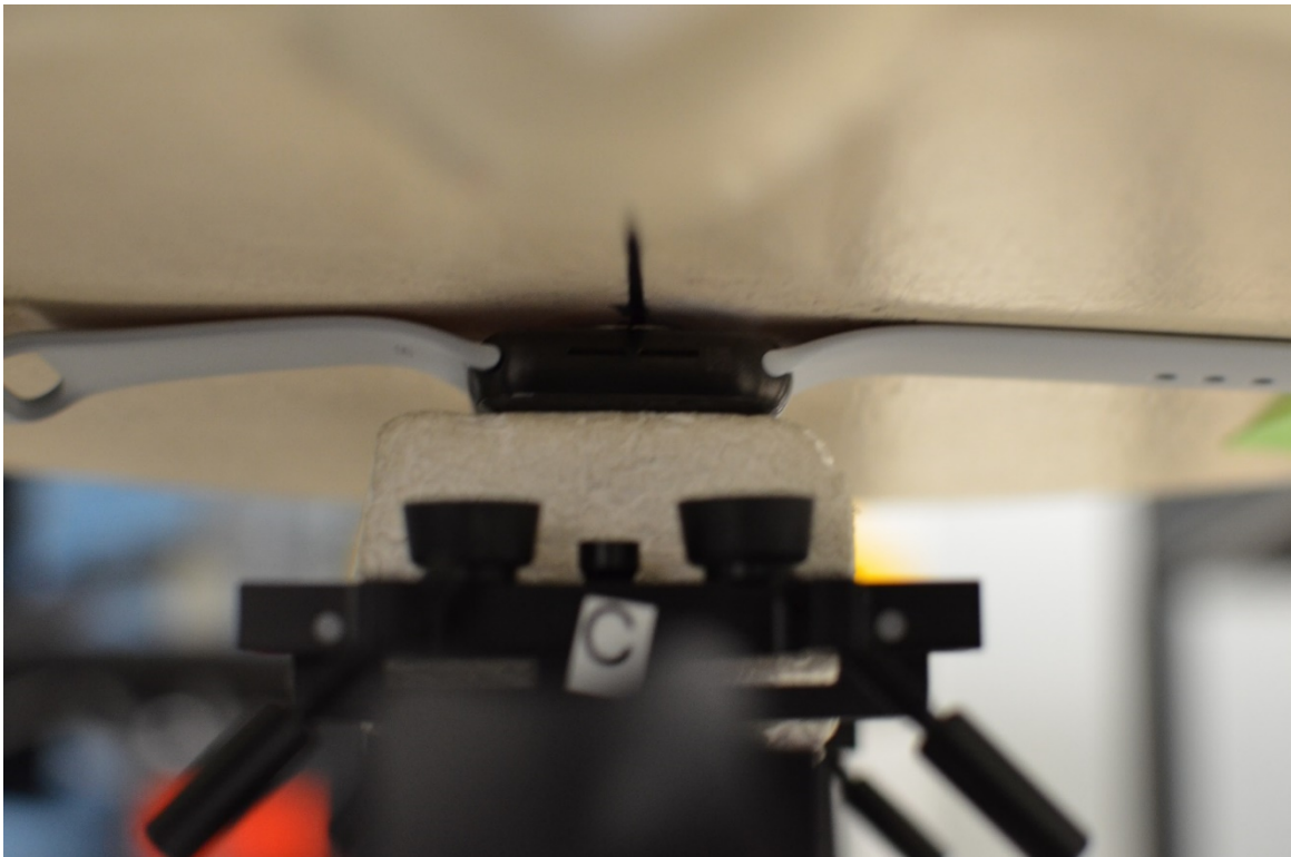
SAR Test Setup Photo 10: Aluminum with Sport Wristband, Back side at 0.0 cm
