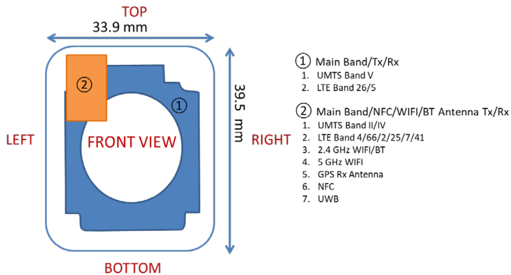
Figure E-1 DUT Antenna Locations
