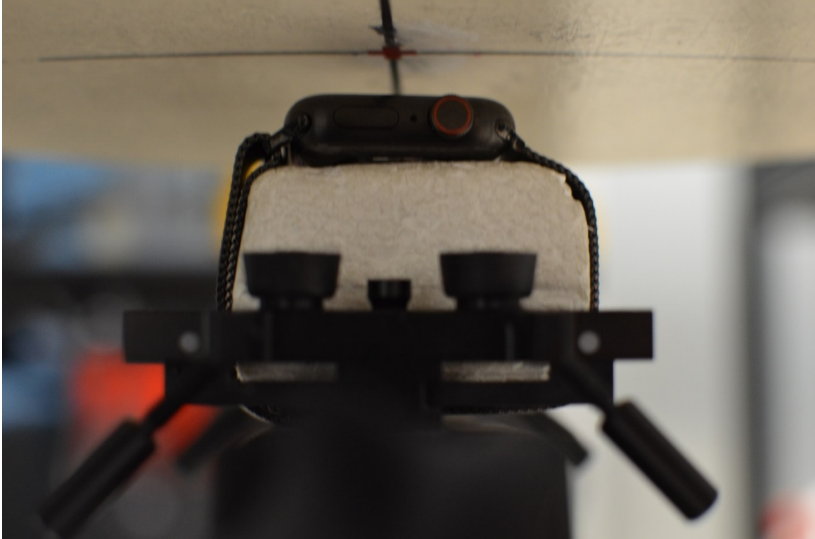
SAR Test Setup Photo 9: Titanium with Metal Loop Wristband, Front side at 1.0 cm
