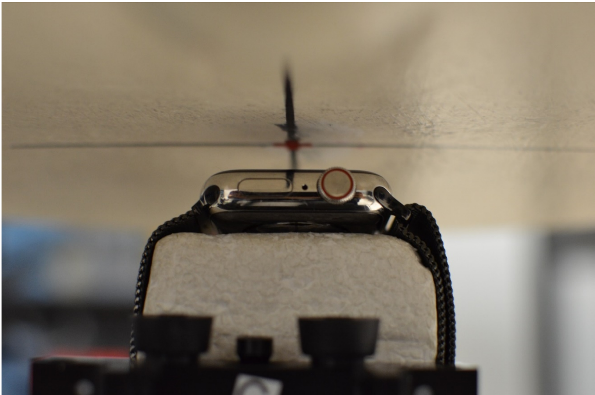
SAR Test Setup Photo 6: Stainless Steel with Metal Loop Wristband, Front side at 1.0 cm
