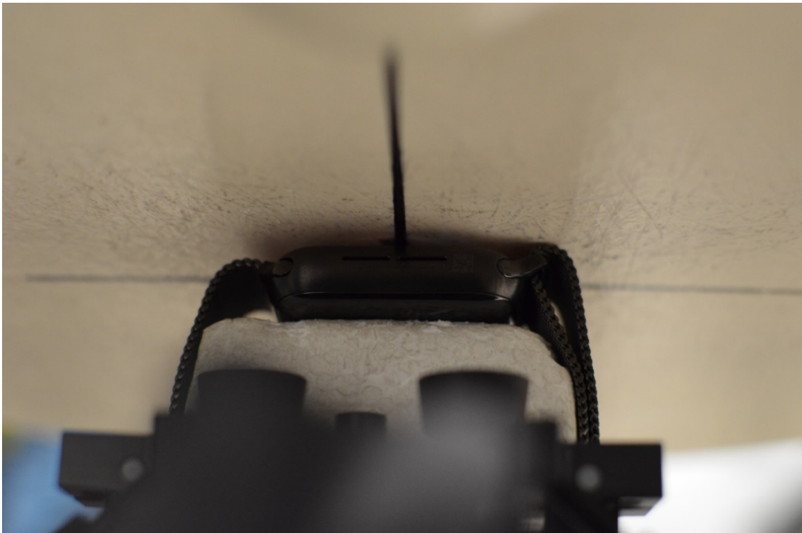
SAR Test Setup Photo 18: Titanium with Metal Loop Wristband, Back side at 0.0 cm
