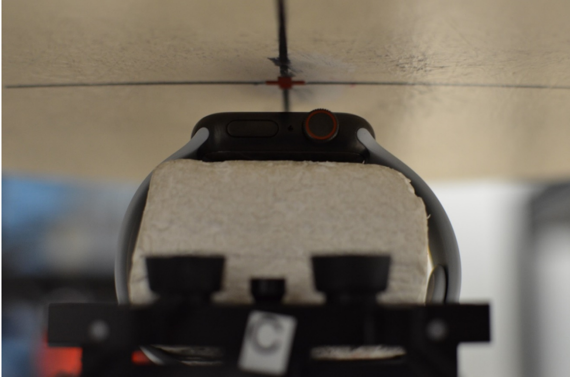
SAR Test Setup Photo 7: Titanium with Sport Wristband, Front side at 1.0 cm
