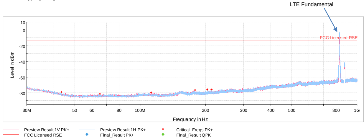
Plot 7-22. Radiated Spurious Emissions Below 1GHz (Band 26)
