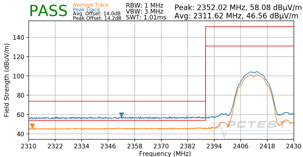
Plot 7-50. Radiated Restricted Lower Band Edge Measurement
