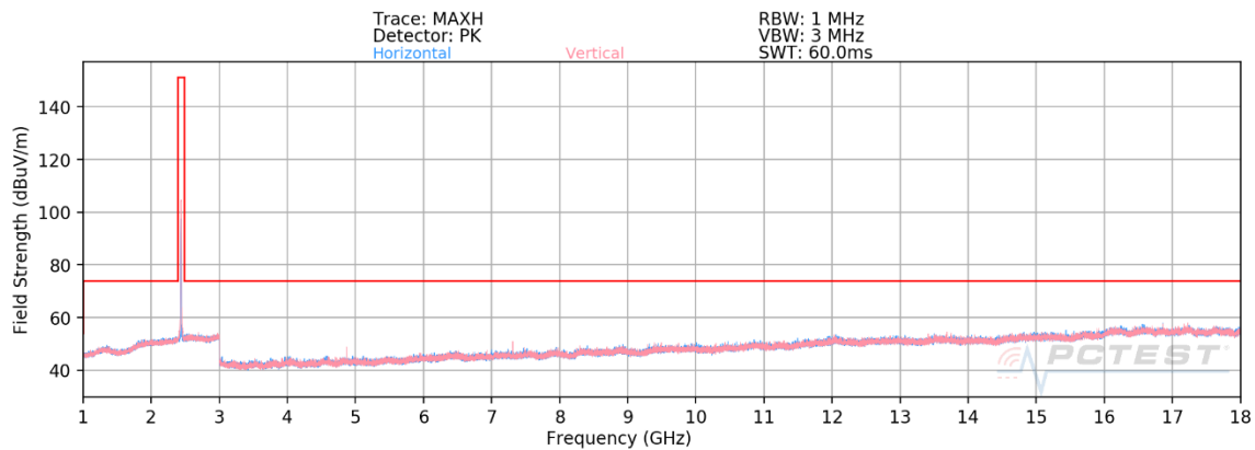
Plot 7-46. Radiated Spurious Emissions 1-18GHz (802.11b – Ch. 6)
