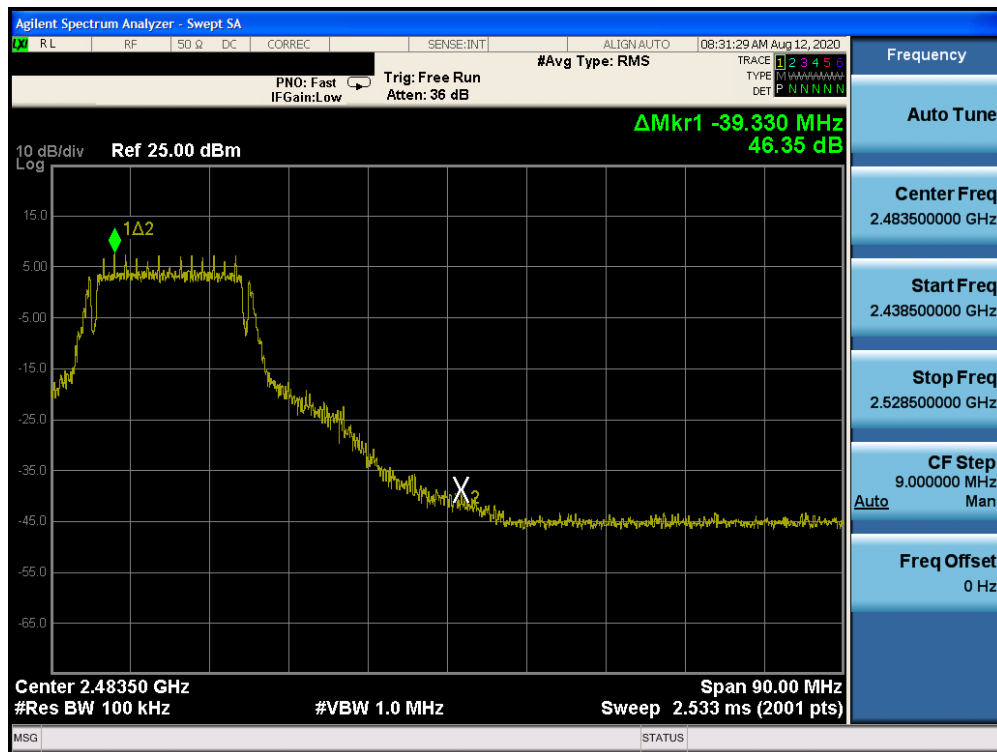
Plot 7-26. Band Edge Plot (802.11g– Ch. 9)
