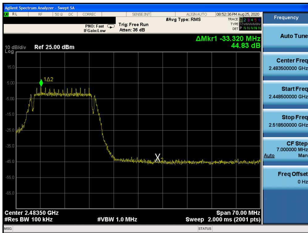
Plot 7-28. Band Edge Plot (802.11g – Ch. 11)
