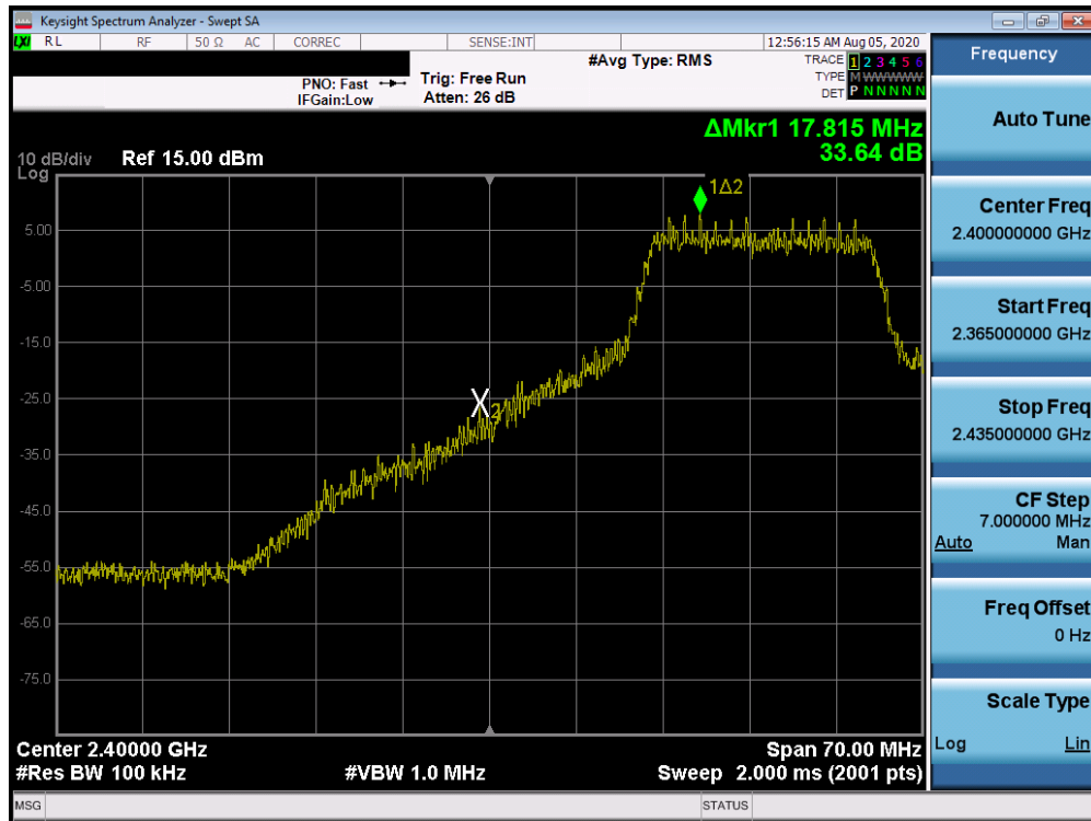
Plot 7-33. Band Edge Plot (802.11n (2.4GHz) – Ch. 3)
