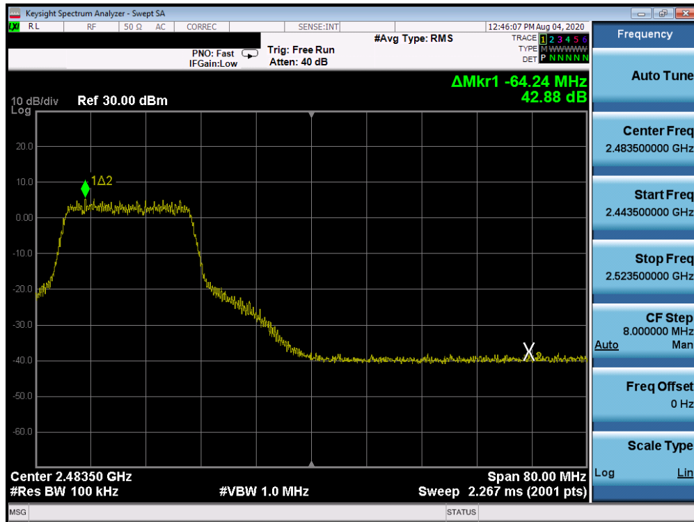
Plot 7-35. Band Edge Plot (802.11n (2.4GHz) – Ch. 10)
