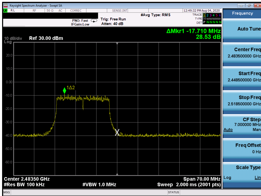
Plot 7-38. Band Edge Plot (802.11n (2.4GHz) – Ch. 13)
