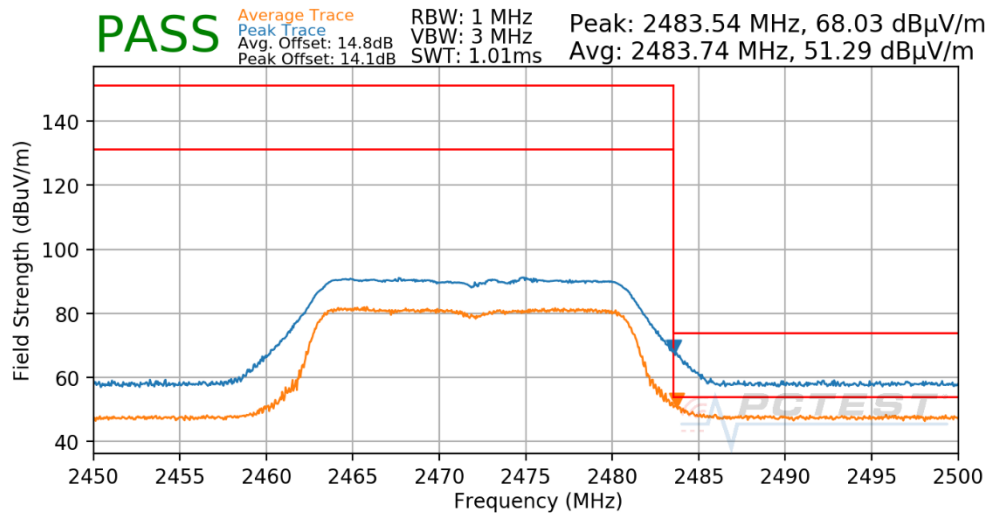
Plot 7-61. Radiated Restricted Upper Band Edge Measurement
