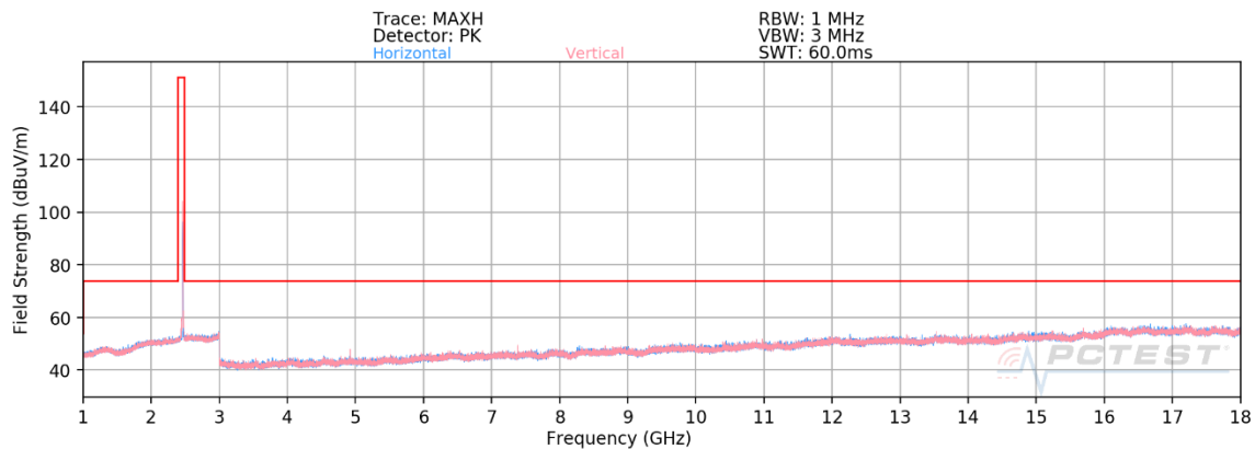
Plot 7-47. Radiated Spurious Emissions 1-18GHz (802.11b – Ch. 11)
