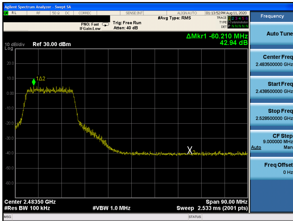
Plot 7-34. Band Edge Plot (802.11n (2.4GHz) – Ch. 9)
