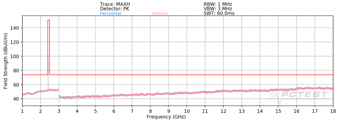
Plot 7-45. Radiated Spurious Emissions 1-18GHz (802.11b – Ch. 1)
