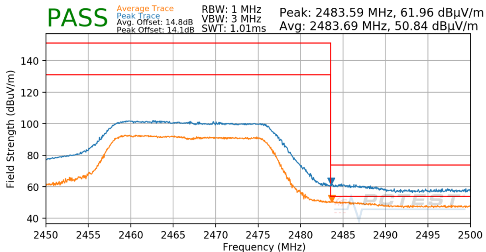
Plot 7-60. Radiated Restricted Upper Band Edge Measurement
