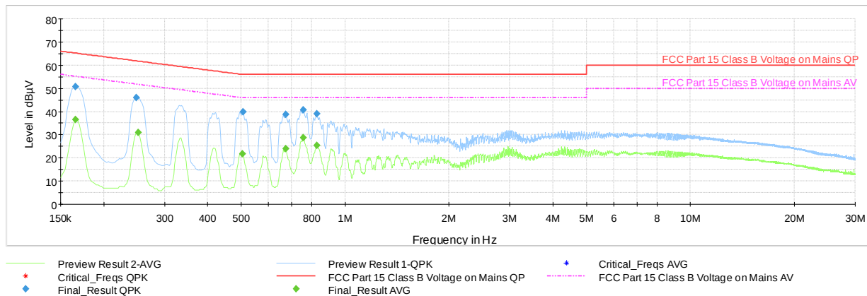
Plot 7-64. AC Line Conducted Emissions with 802.11b Ch.6 (N, with WCP + AC/DC Adapter)
