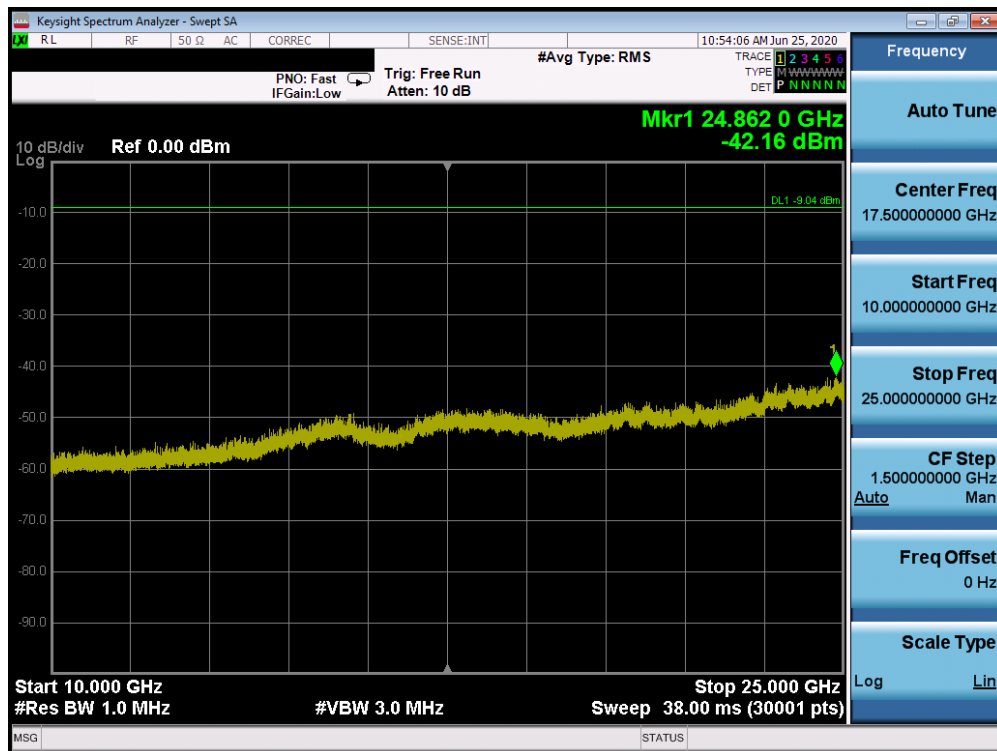
Plot 7-44. Conducted Spurious Plot (802.11b – Ch. 11)
