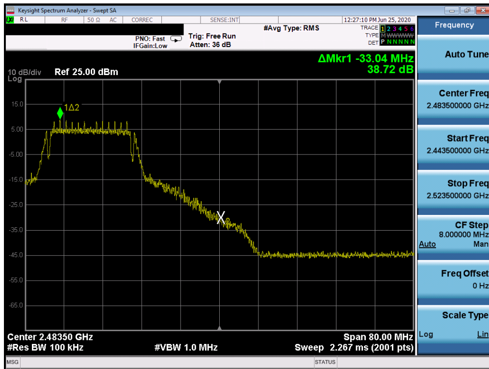
Plot 7-27. Band Edge Plot (802.11g– Ch. 10)
