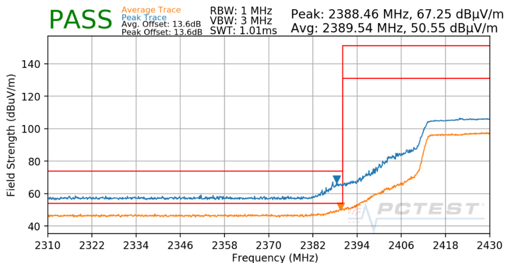
Plot 7-56. Radiated Restricted Lower Band Edge Measurement
