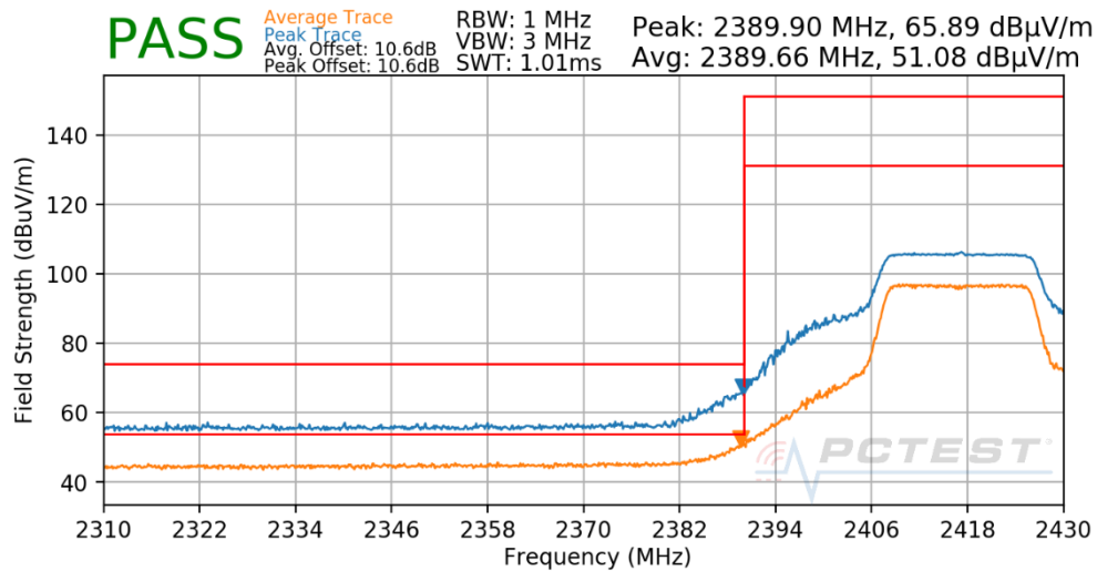
Plot 7-55. Radiated Restricted Lower Band Edge Measurement
