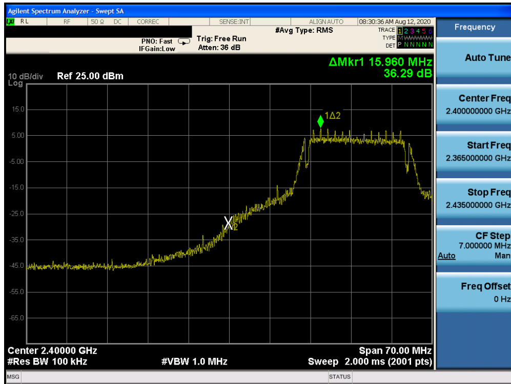
Plot 7-25. Band Edge Plot (802.11g– Ch. 3)
