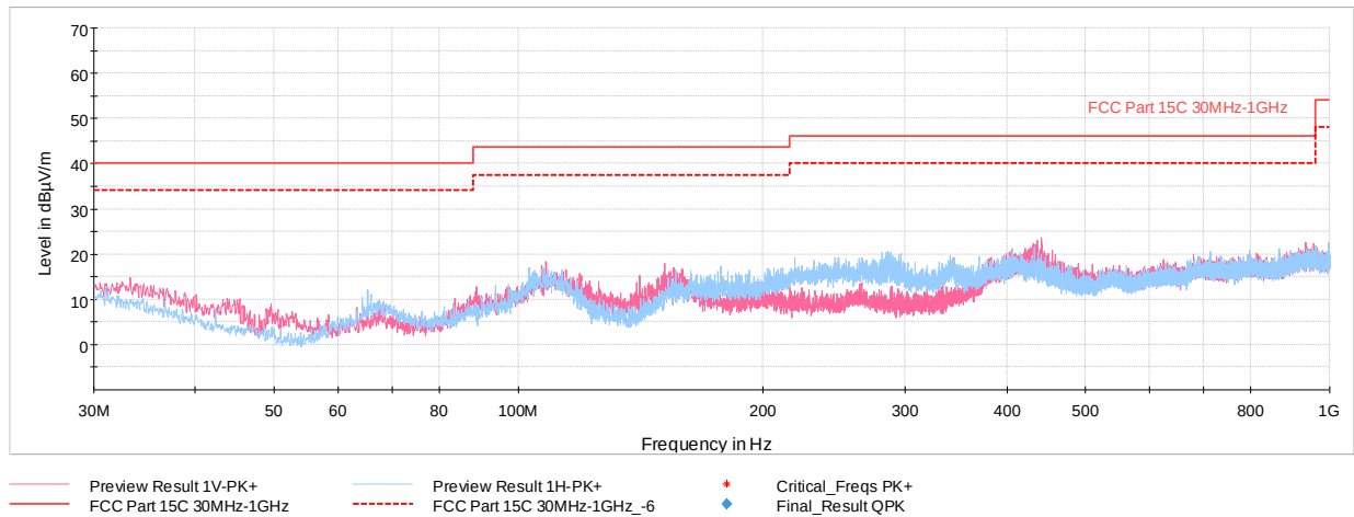
Plot 7-62. Radiated Spurious Emissions 30MHz-1GHz (802.11b – Ch.6, with WCP + laptop)
