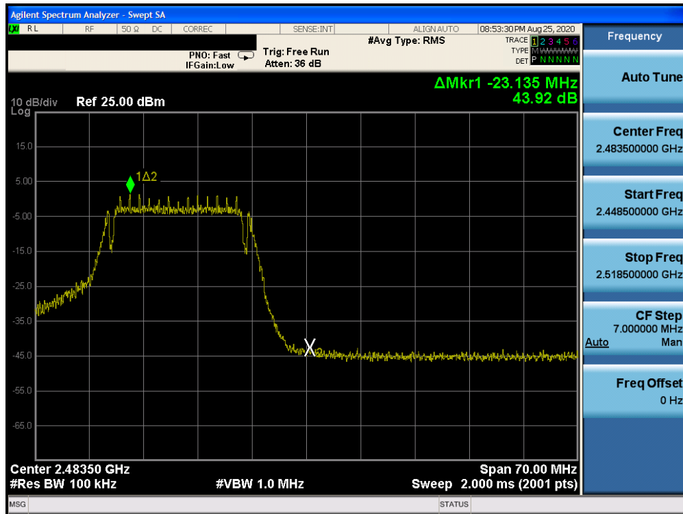
Plot 7-29. Band Edge Plot (802.11g - Ch. 12)
