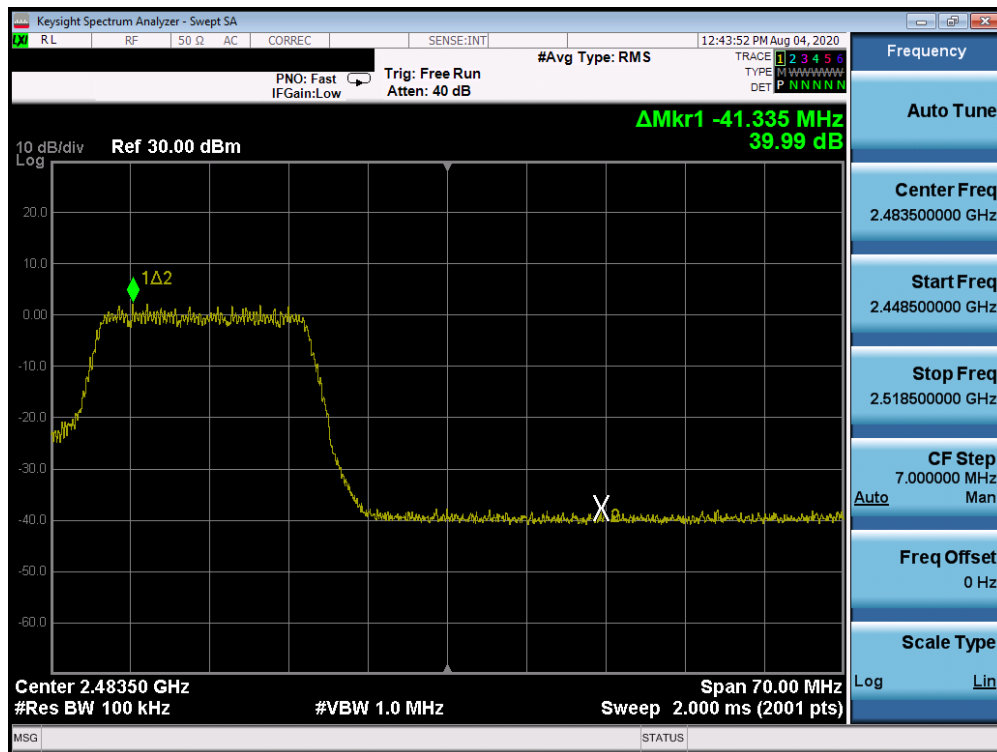
Plot 7-36. Band Edge Plot (802.11n (2.4GHz) – Ch. 11)
