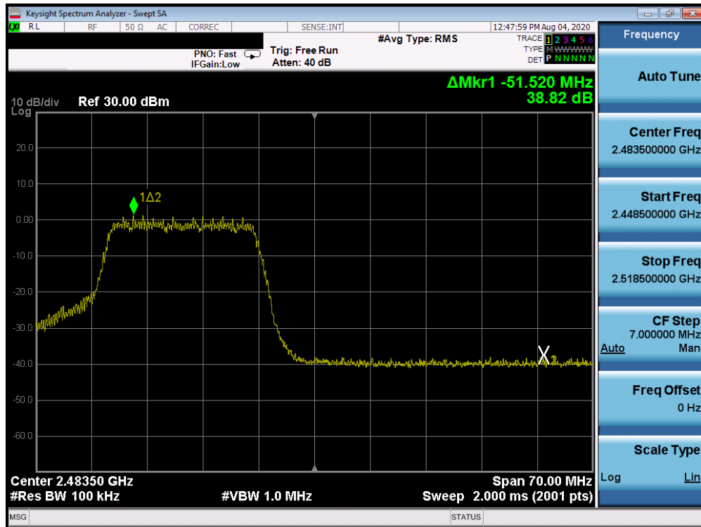
Plot 7-37. Band Edge Plot (802.11n (2.4GHz) – Ch. 12)
