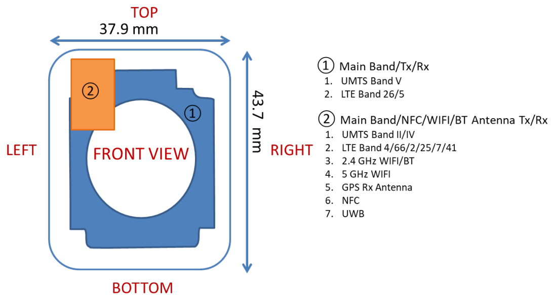
Figure E-1 DUT Antenna Locations
