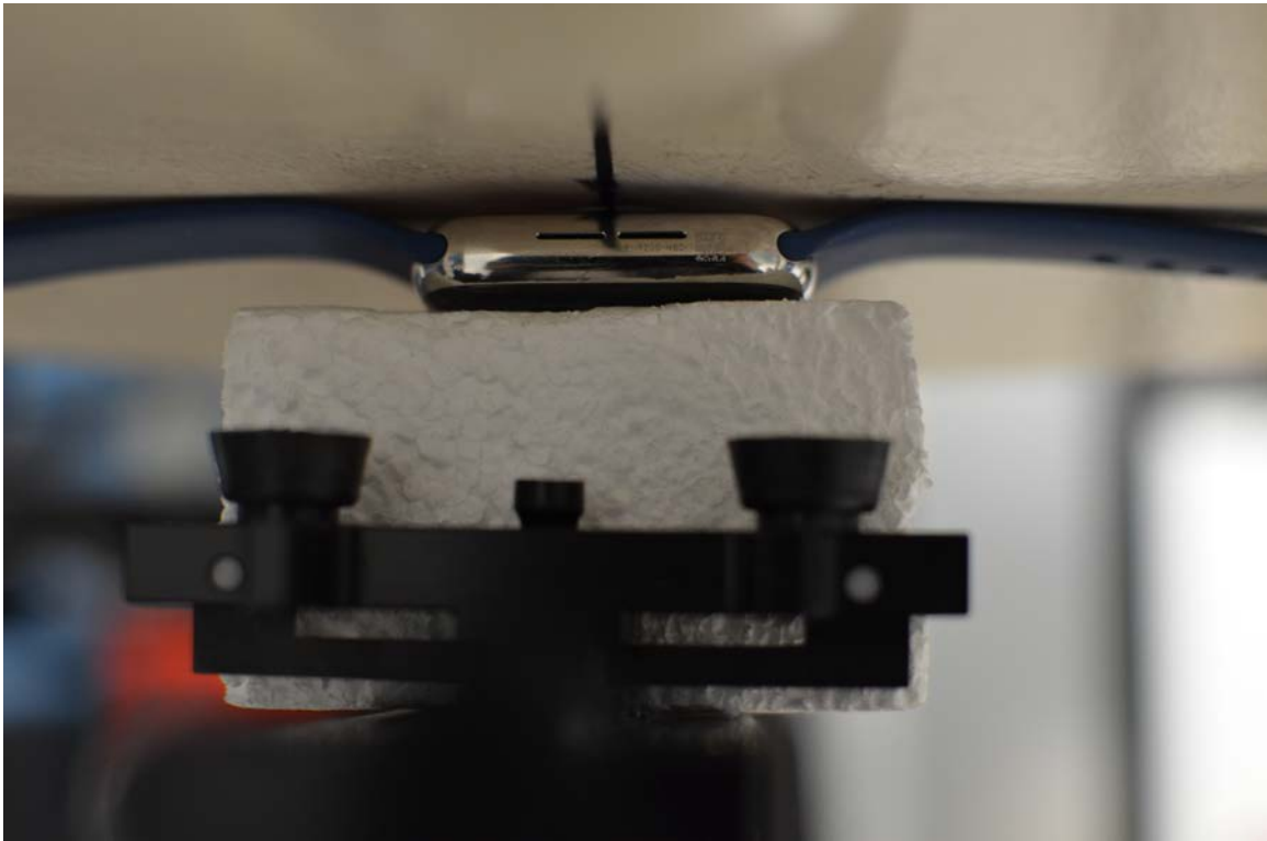
SAR Test Setup Photo 13: Stainless Steel with Sport Wristband, Back Side at 0.0 cm
