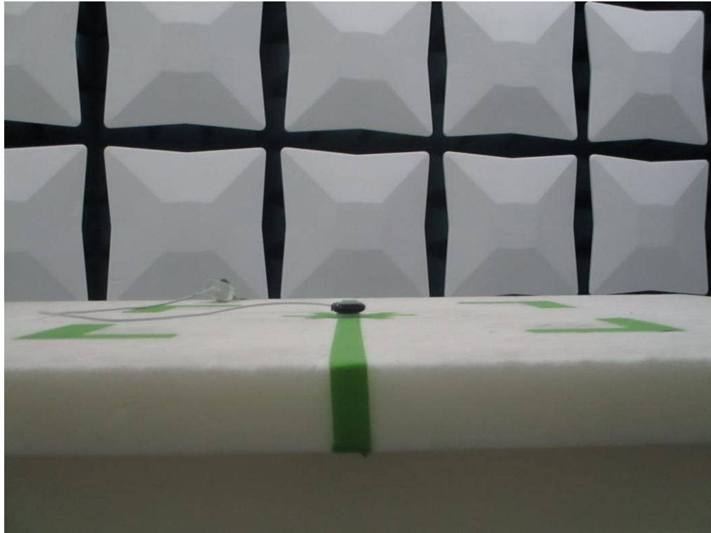
Figure 1: 1-18GHz Test Setup (Front View)
