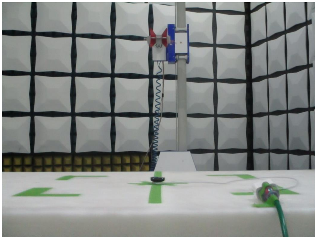
Figure 2: 1-18GHz Test Setup (Rear View)
