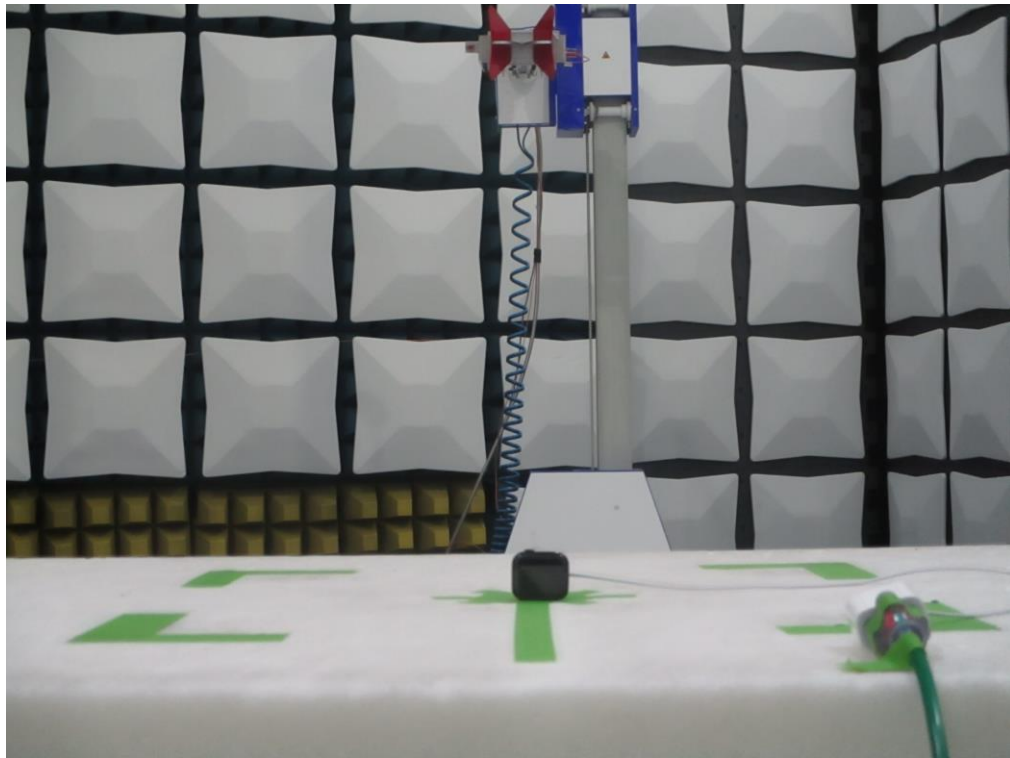
Figure 4: 1-18GHz Test Setup (Rear View)
