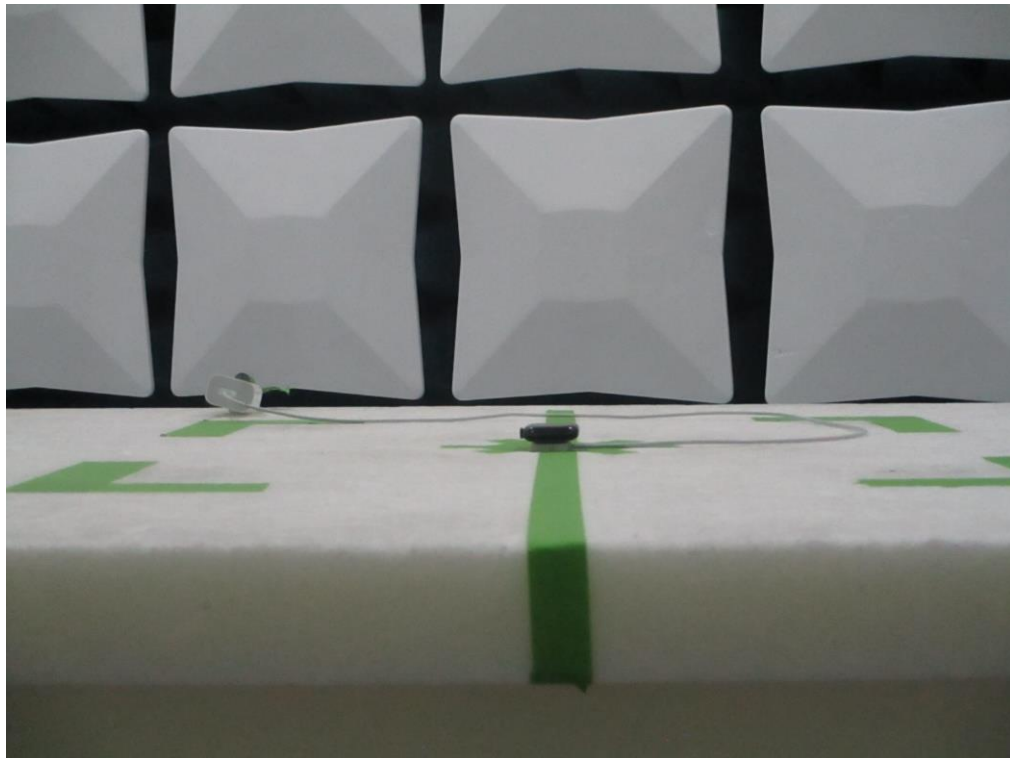
Figure 8: 30MHz-1GHz Test Setup (Rear View)
