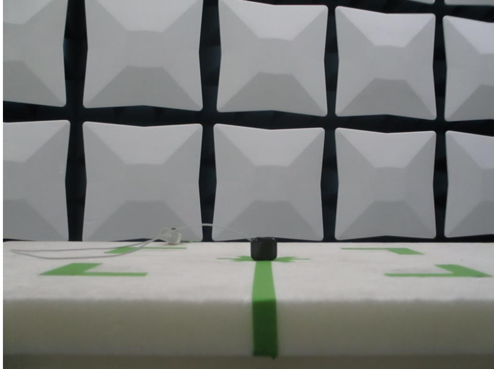
Figure 3: 1-18GHz Test Setup (Front View)
