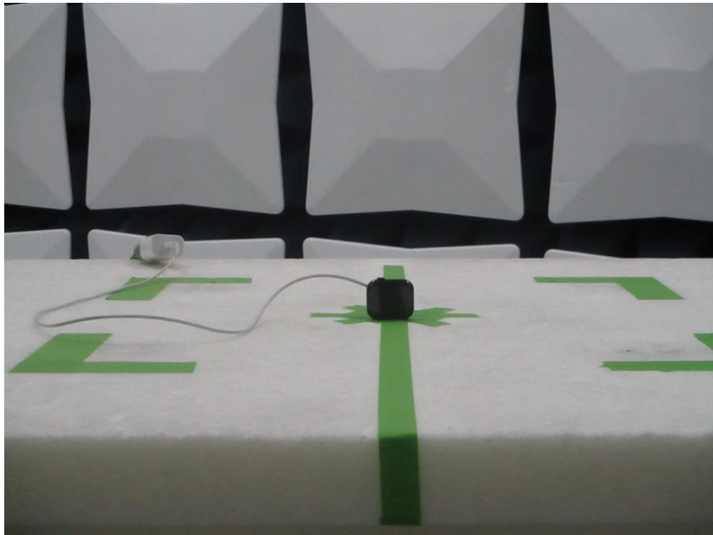
Figure 10: 30MHz-1GHz Test Setup (Rear View)
