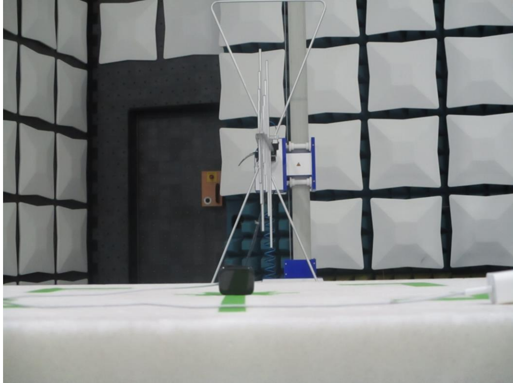
Figure 9: 30MHz-1GHz Test Setup (Front View)
