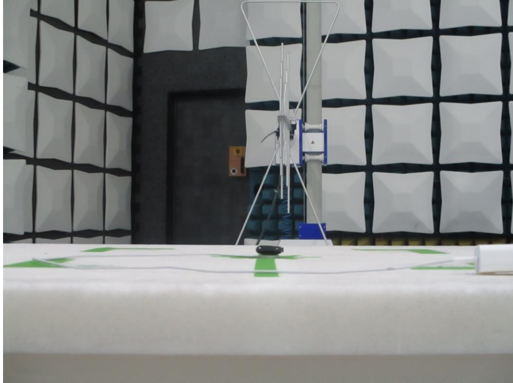
Figure 7: 30MHz-1GHz Test Setup (Front View)
