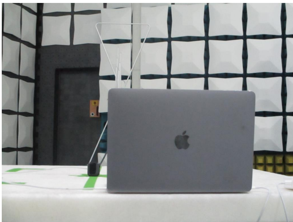
Figure 22: 30MHz-1GHz Test Setup (Rear View)
