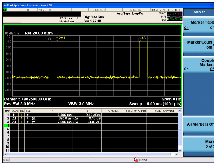
Figure 7-2 802.15.4 ab-NB Transmission Plot
