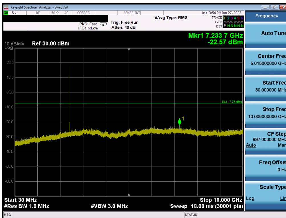
Plot 7-23. Conducted Spurious Plot (Bluetooth (HDR4), 4 Mbps, ePA – Ch. 1)
