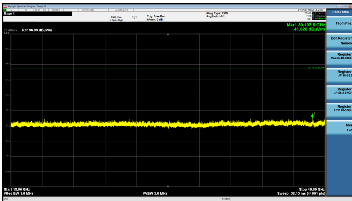
Plot 7-33. Radiated Spurious Plot Above 18GHz (4Mbps, HDR4, ePA – Ch.38, Ant. Pol. V)
