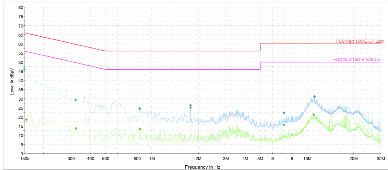
Plot 7-40. AC Line Conducted Plot with Bluetooth HDR (N, 4Mbps ePA - Ch.38 with AC/DC Adapter + Laptop Charger)
