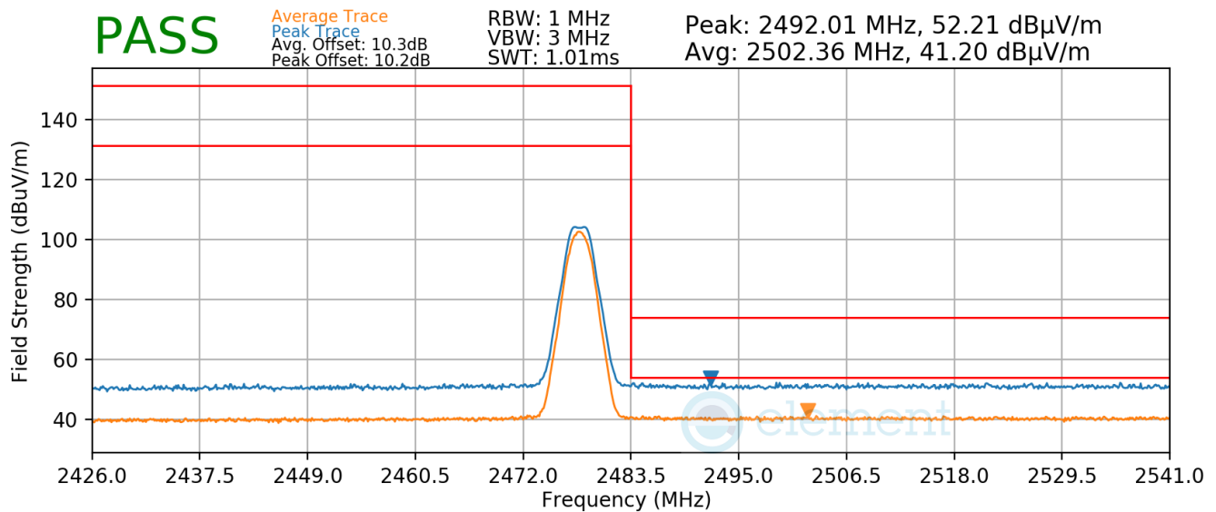
Plot 7-37. Radiated Restricted Upper Band Edge Measurement
