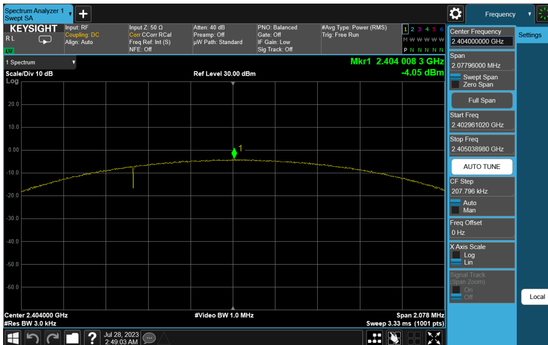
Plot 7-13. Power Spectral Density Plot (Bluetooth (LE), 2Mbps, ePA – Ch. 1)
