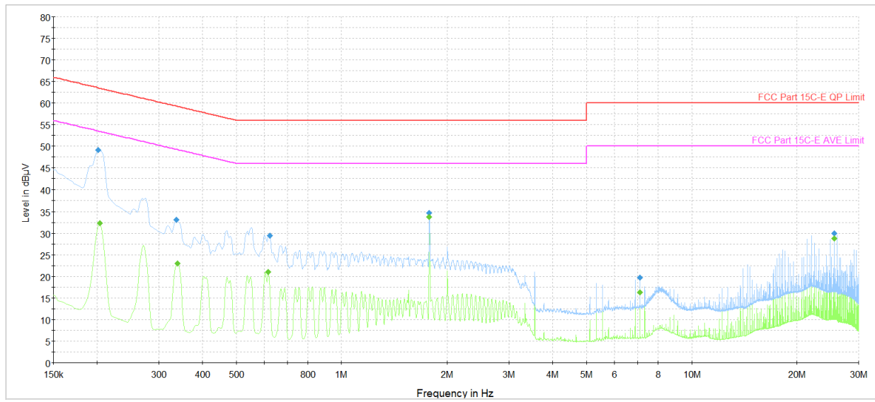
Plot 7-40. AC Line Conducted Plot with Bluetooth LE (N, 1Mbps ePA – Ch.19 with AC/DC Adapter + Laptop Charger)
