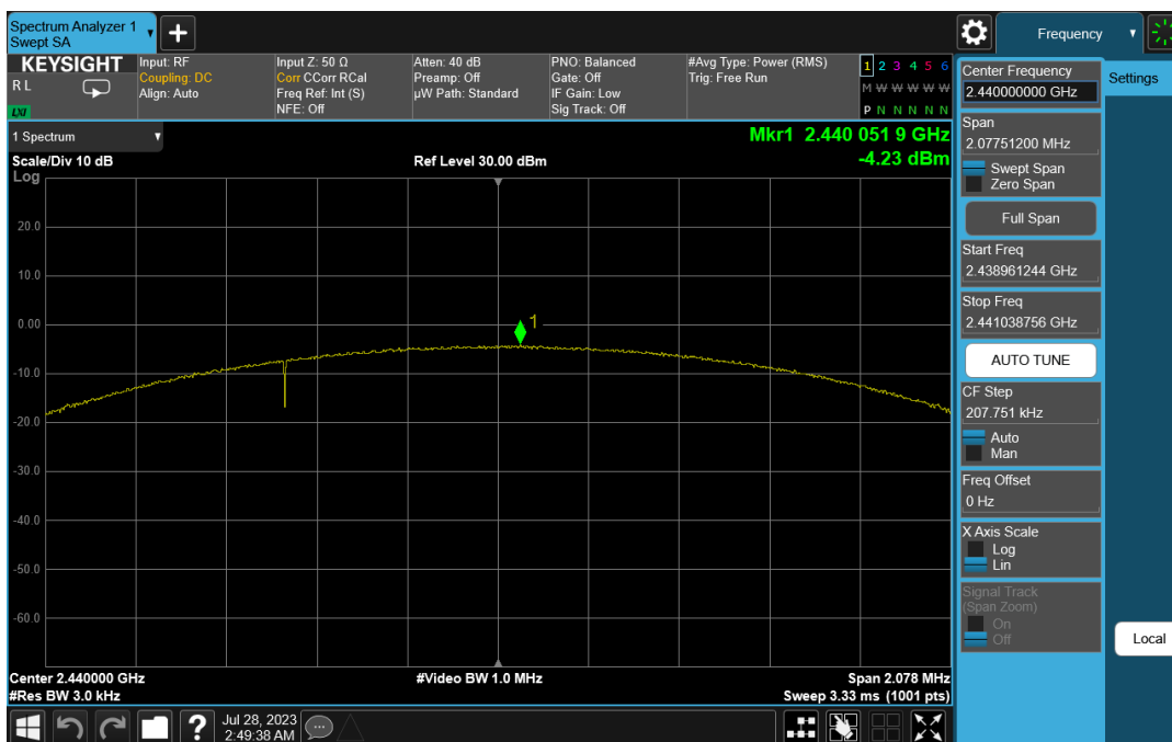
Plot 7-14. Power Spectral Density Plot (Bluetooth (LE), 2Mbps, ePA – Ch. 19)
