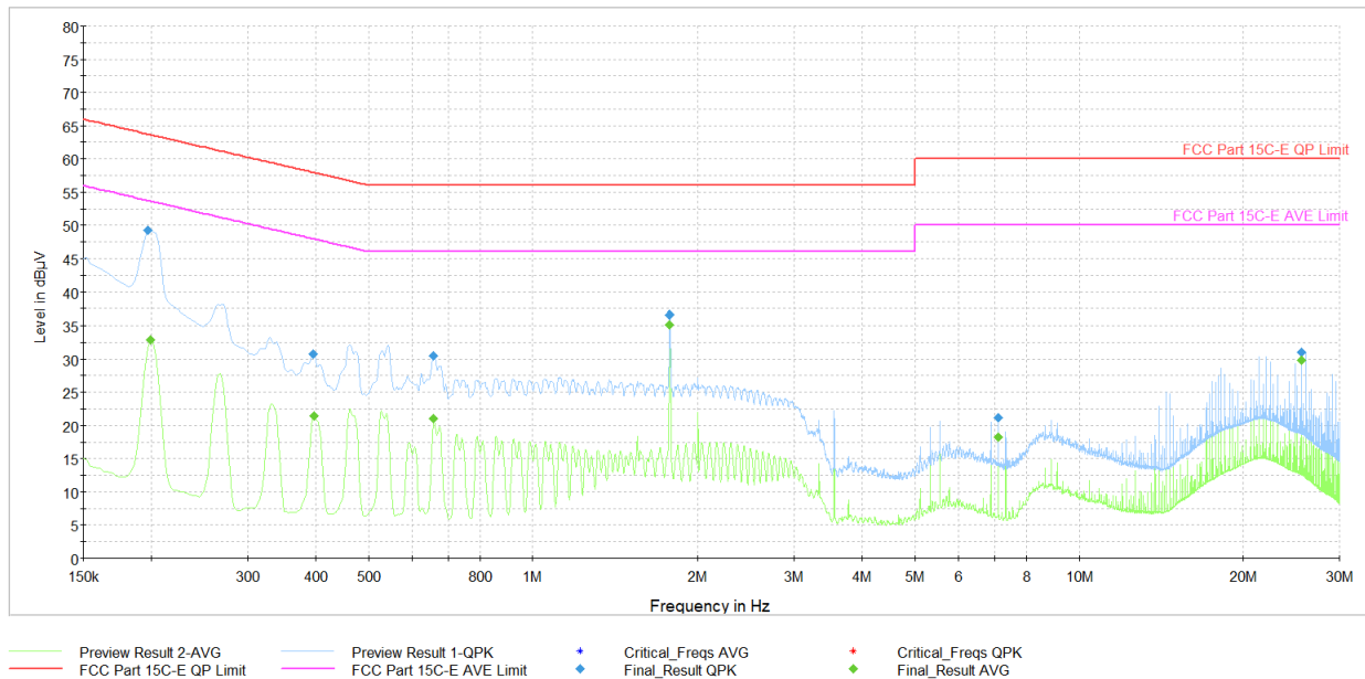
Plot 7-39. AC Line Conducted Plot with Bluetooth LE (L1, 1Mbps ePA – Ch.19 with AC/DC Adapter + Laptop Charger)
