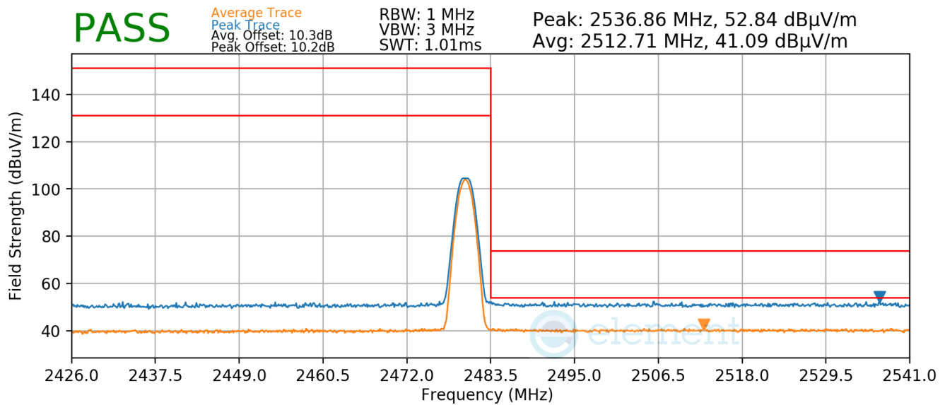
Plot 7-35. Radiated Restricted Upper Band Edge Measurement
