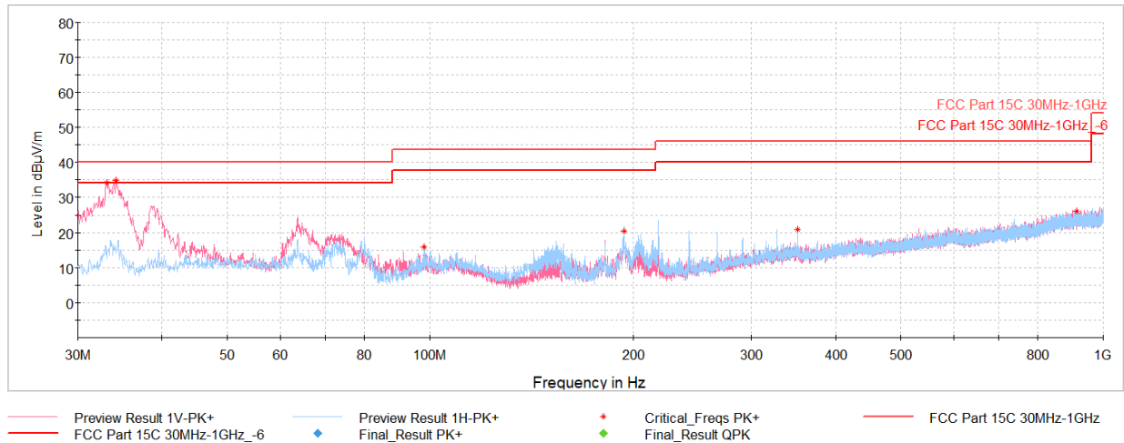
Plot 7-38. Radiated Spurious Emissions Below 1GHz (1Mbps, ePA – Ch.19, Pol. H & V, with AC/DC Adapter + Magnetic Charger)
