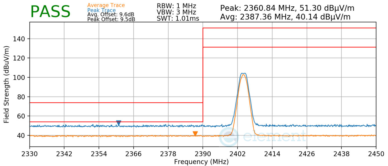
Plot 7-36. Radiated Restricted Lower Band Edge Measurement
