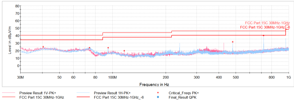
Plot 6-12. Radiated Spurious Emissions 30MHz – 1GHz (Mode 1, with Magnetic Charger & Laptop)
