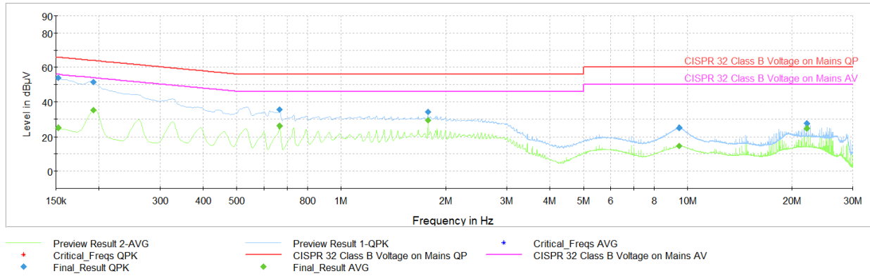
Plot 6-13. AC Line Conducted Plot (L1 - Mode 1, with Magnetic Charger & Laptop)
