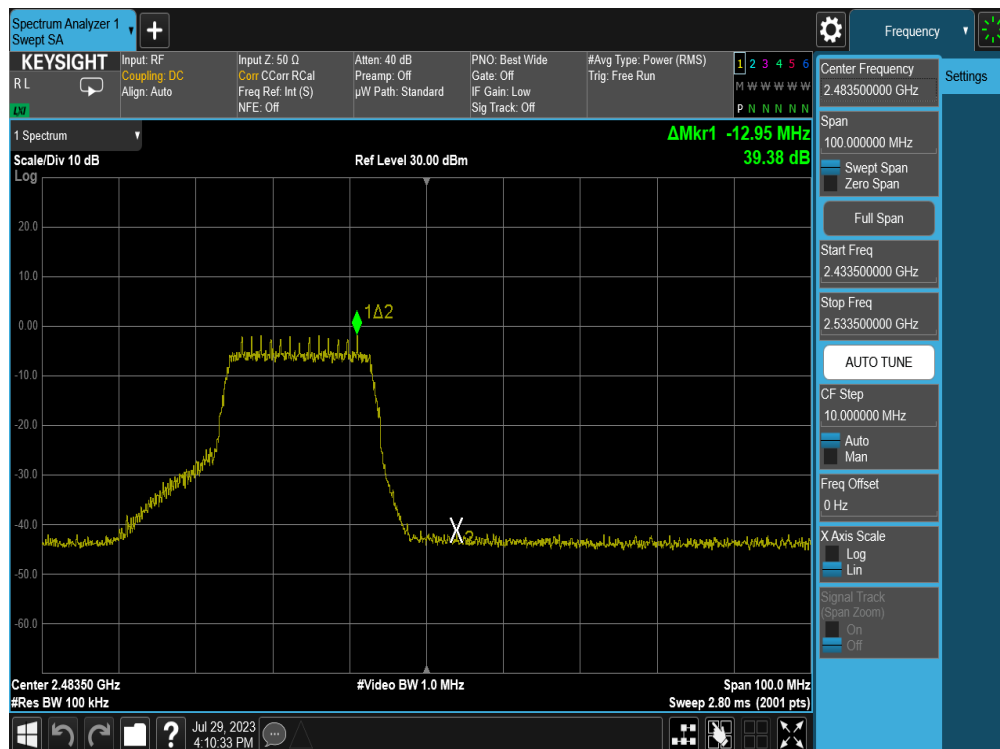
Plot 7-38. Band Edge Plot (802.11n (2.4GHz) – Ch. 12) – MCS0
