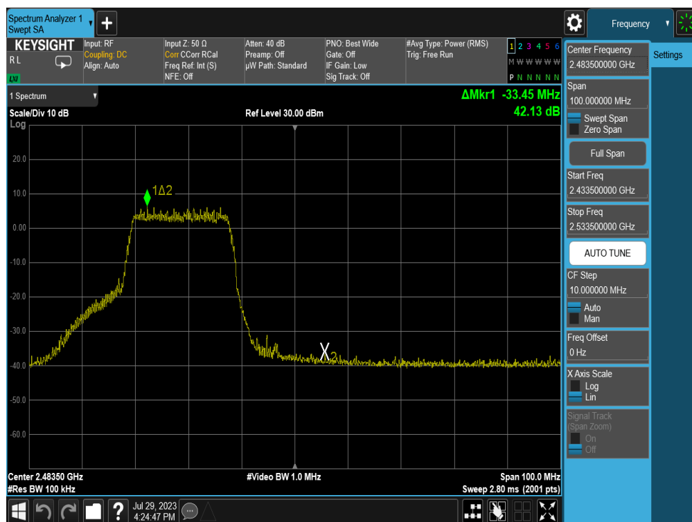
Plot 7-43. Band Edge Plot (802.11n (2.4GHz) – Ch. 11) – MCS7
