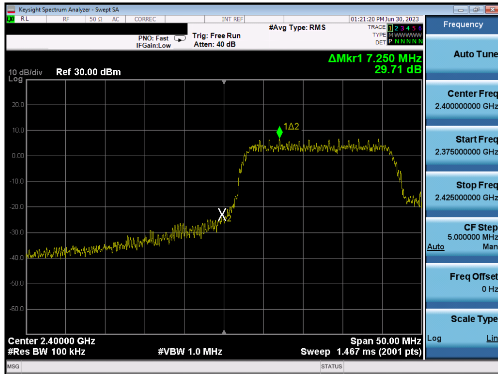
Plot 7-41. Band Edge Plot (802.11n (2.4GHz) – Ch. 2) – MCS7
