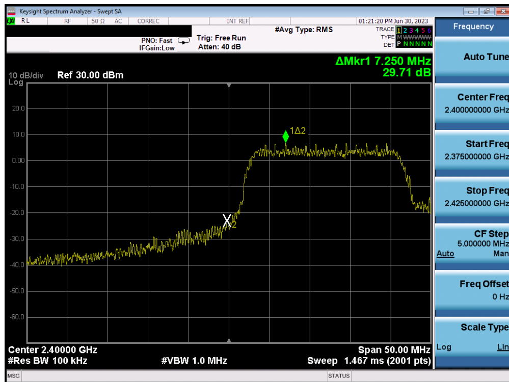
Plot 7-40. Band Edge Plot (802.11n (2.4GHz) – Ch. 1) – MCS7
