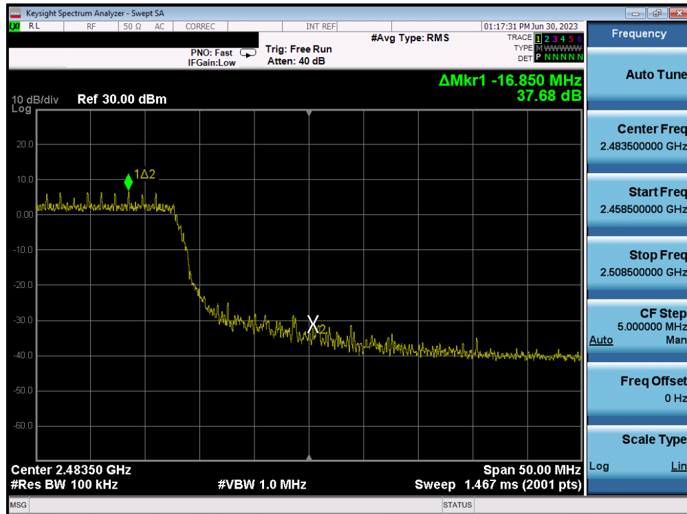
Plot 7-39. Band Edge Plot (802.11n (2.4GHz) – Ch. 13) – MCS0
