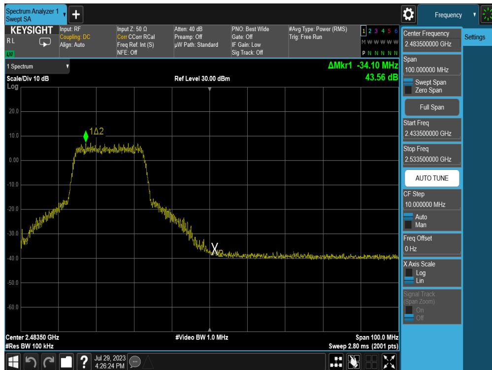
Plot 7-42. Band Edge Plot (802.11n (2.4GHz) – Ch. 10) – MCS7
