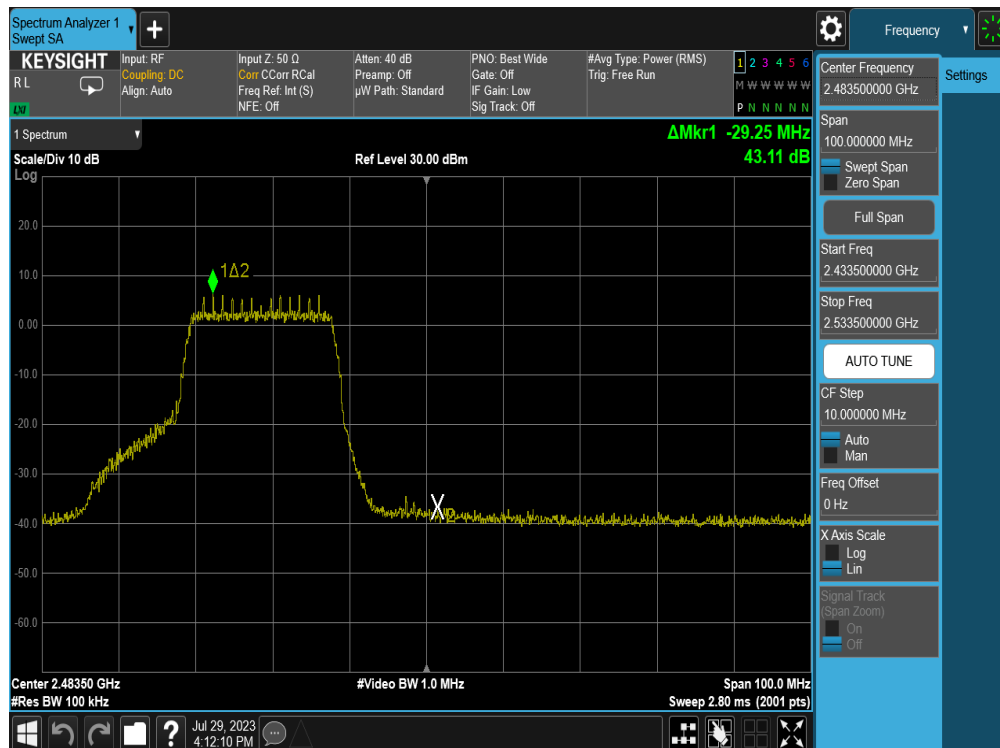
Plot 7-37. Band Edge Plot (802.11n (2.4GHz) – Ch. 11) – MCS0
