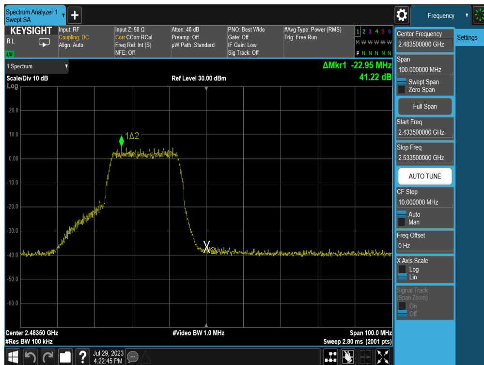
Plot 7-44. Band Edge Plot (802.11n (2.4GHz) – Ch. 12) – MCS7
