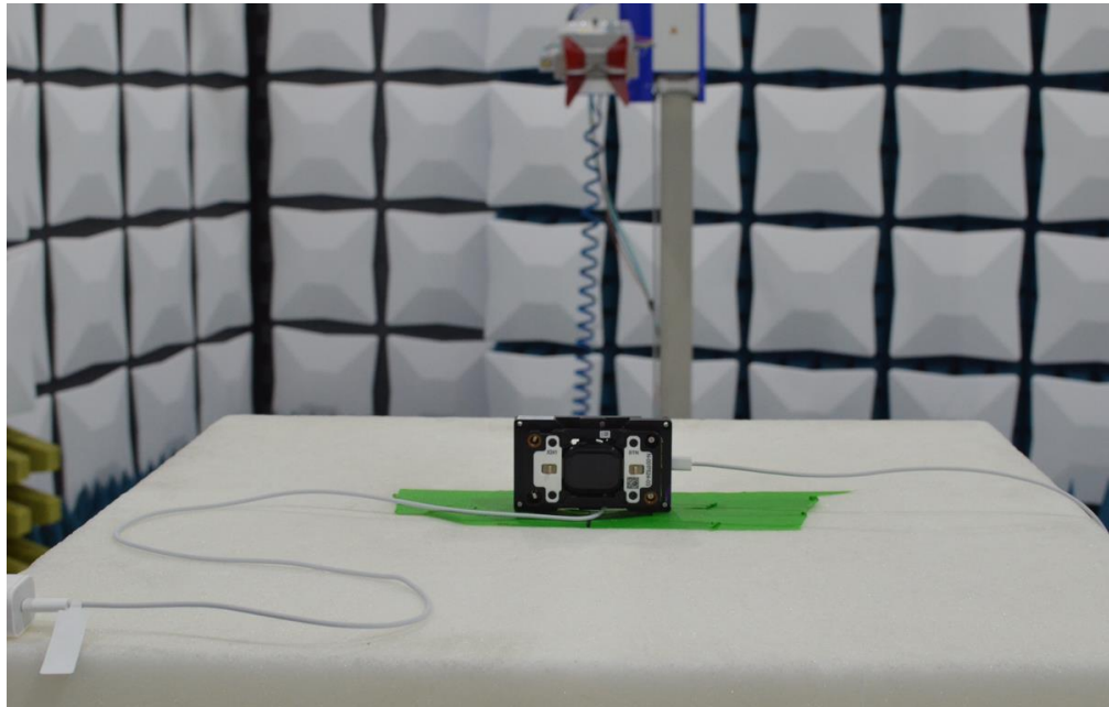
Figure 9: 1-18GHz Test Setup (Rear View)
