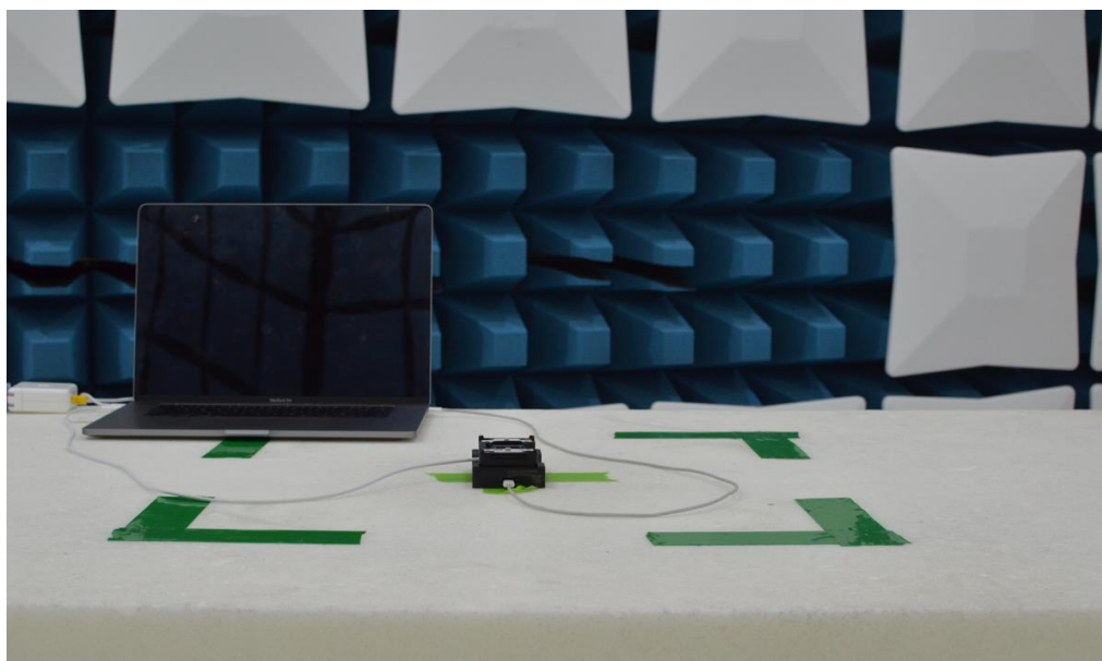
Figure 12: 30MHz-1GHz Test Setup (Front View)
