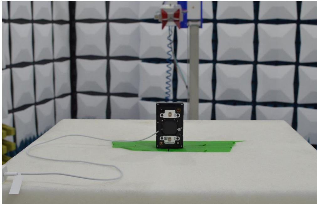
Figure 11: 1-18GHz Test Setup (Rear View)
