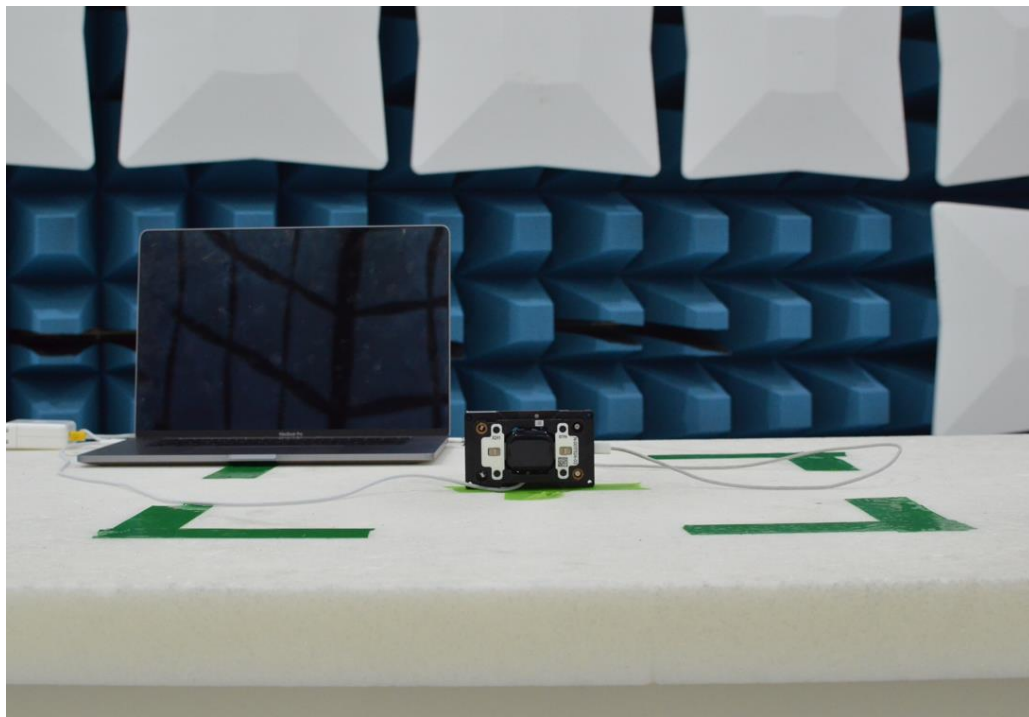
Figure 14: 30MHz-1GHz Test Setup (Front View)
