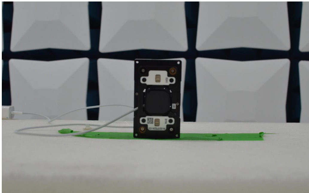
Figure 10: 1-18GHz Test Setup (Front View)
