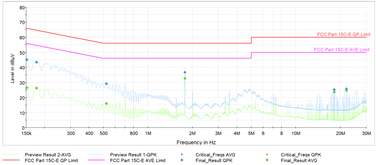
Plot 7-31. AC Line Conducted Plot (OQPSK – Ch. 24) (L1) with AC/DC Adapter & Magnetic charger
