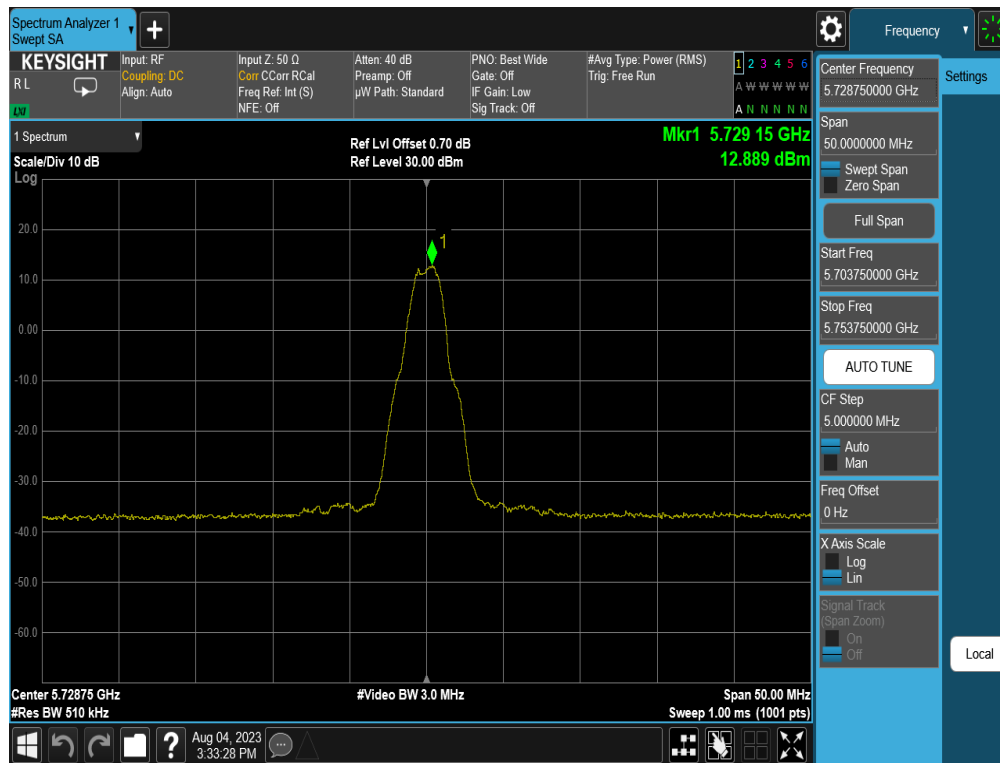
Plot 7-10. PSD (OQPSK, 5728.75MHz, 250kpbs)
