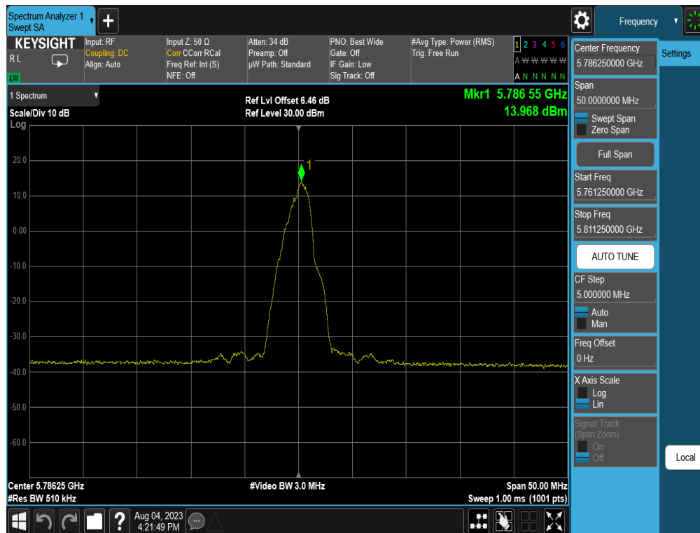
Plot 7-17. PSD (OQPSK, 5786.25MHz, 1000kpbs)
