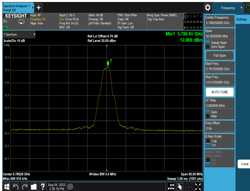
Plot 7-11. PSD (OQPSK, 5786.25MHz, 250kpbs)
