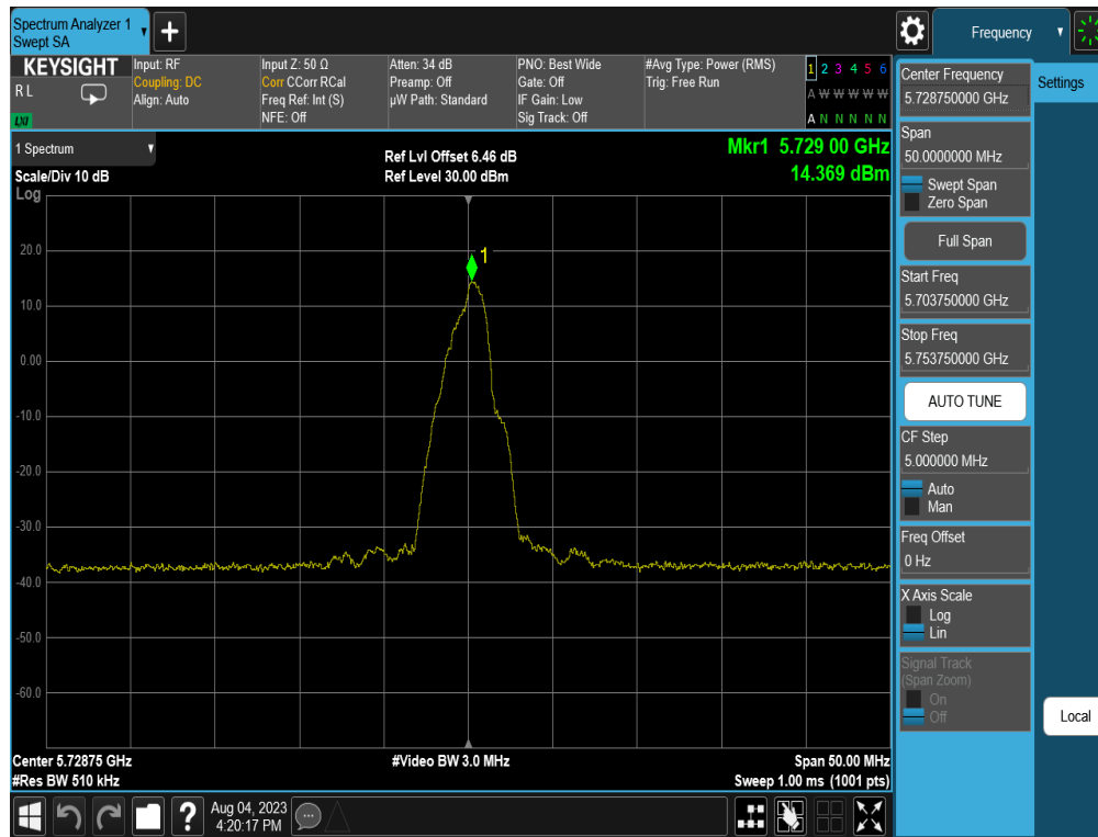
Plot 7-16. PSD (OQPSK, 5728.75MHz, 1000kpbs)
