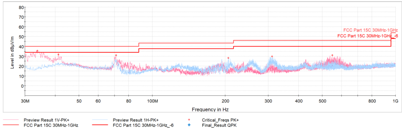
Plot 7-30. RSE 30MHz - 1GHz (OQPSK - Ch. 24), with Laptop & Magnetic charger
