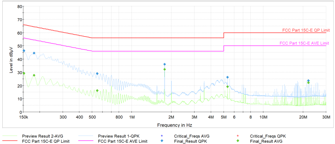
Plot 7-32. AC Line Conducted Plot (OQPSK – Ch. 24) (N) with AC/DC Adapter & Magnetic charger
