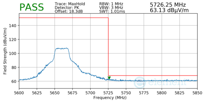
Plot 7-52. (Pk, Ch.132, 802.11n, MCS7)
