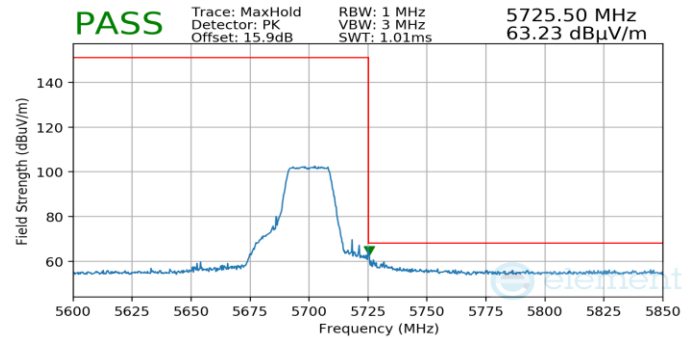
Plot 7-55. (Pk, Ch.140, 802.11n, MCS0)
