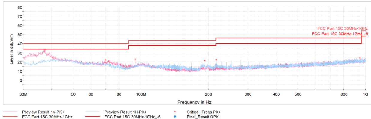
Plot 7-62. Radiated Spurious Emissions – Simultaneous Transmission 30MHz – 1GHz, with AC/DC Adapter & magnetic charger
