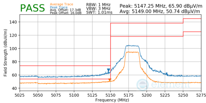
Plot 7-46. (Pk & Avg, Ch.36, 802.11n, MCS7)
