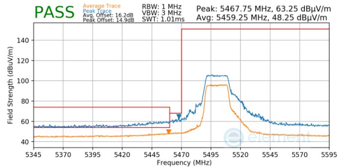
Plot 7-50. (Pk & Avg, Ch.100, 802.11n, MCS7)
