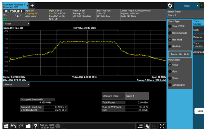
Plot 7-9. 26dB BW & 99% OBW (20MHz BW 802.11n – Ch. 144, MCS0)
