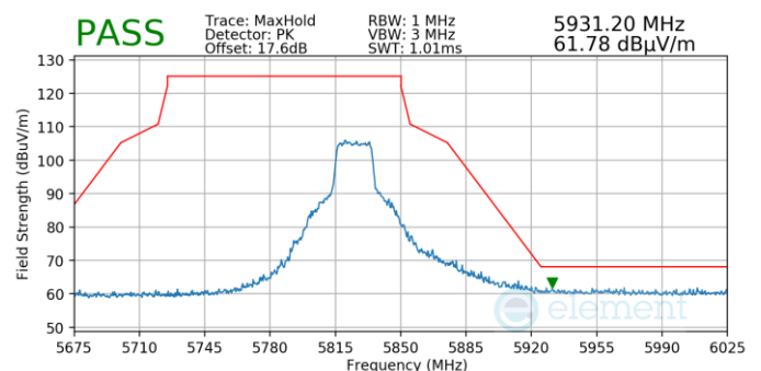
Plot 7-60. (Pk, Ch.165, 802.11n, MCS7)
