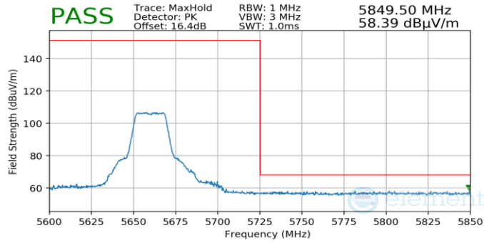
Plot 7-51. (Pk, Ch.132, 802.11n, MCS0)
