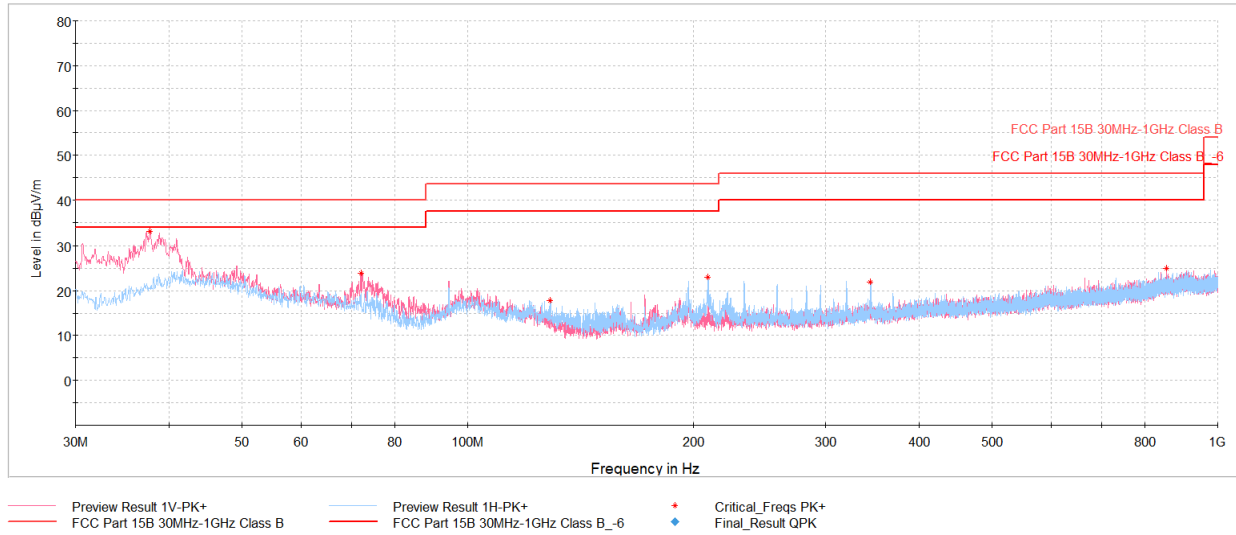
Plot 7-61. Radiated Spurious Emissions below 1GHz, 802.11n, Ch.144 with AC/DC Adapter & magnetic charger
