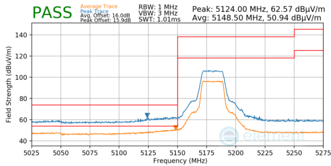
Plot 7-45. (Pk & Avg, Ch.36, 802.11n, MCS0)
