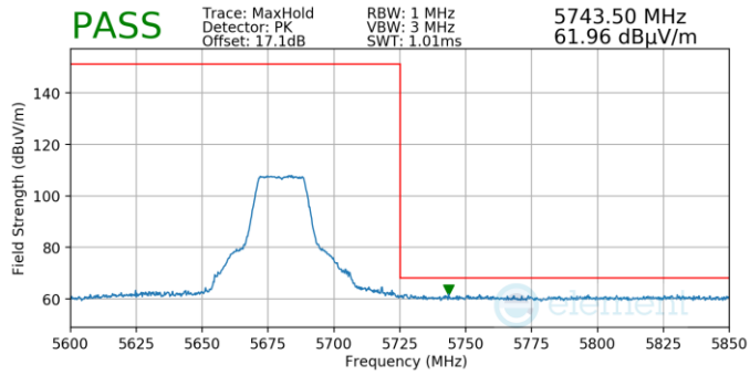
Plot 7-53. (Pk, Ch.136, 802.11n, MCS0)
