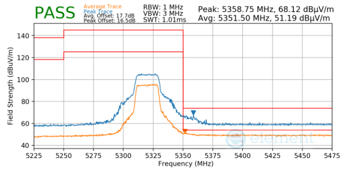
Plot 7-48. (Pk & Avg, Ch.64, 802.11n, MCS7)
