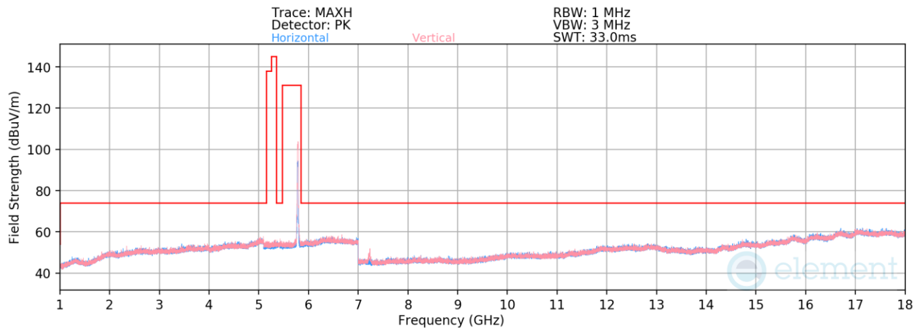
Plot 7-40. Radiated Spurious Emissions above 1GHz (802.11n – Ch. 157)
