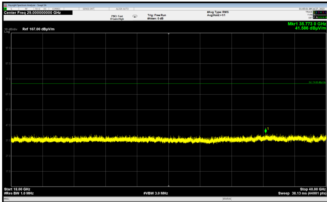
Plot 7-43. Radiated Spurious Emissions Simultaneous Transmission 18GHz – 40GHz Pol H
