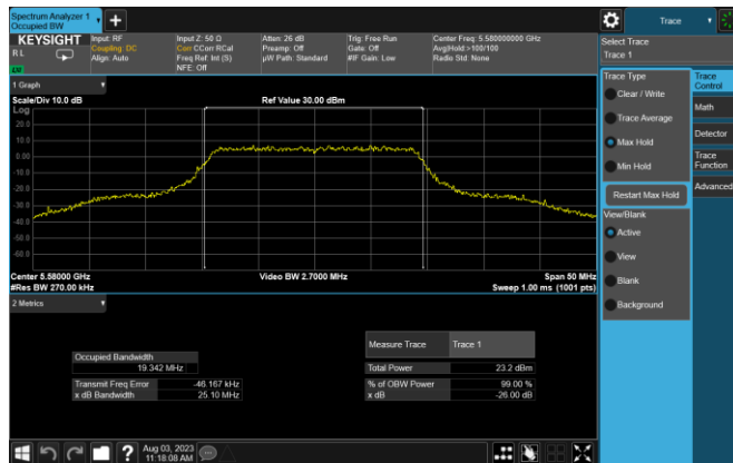
Plot 7-8. 26dB BW & 99% OBW (20MHz BW 802.11n – Ch. 116, MCS0)
