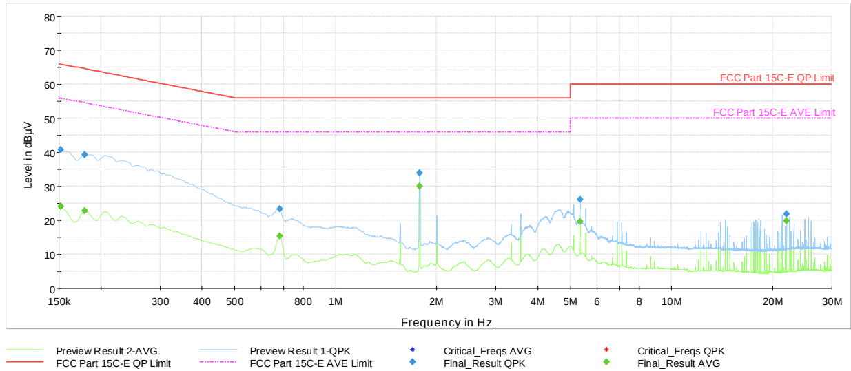
Plot 7-64. AC Line Conducted Plot with 802.11n- Ch.144 (N), with AC/DC Adapter & magnetic charger
