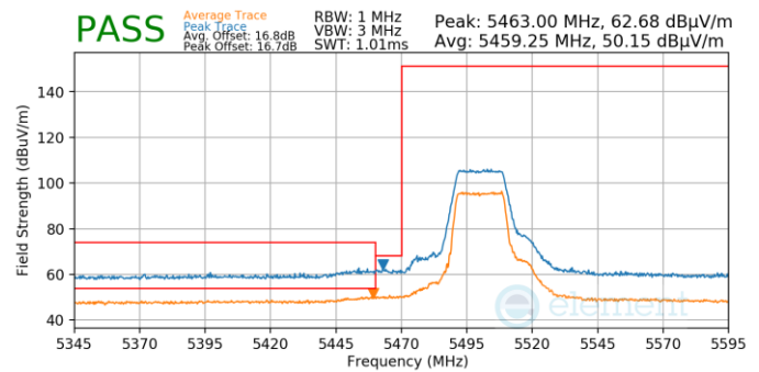
Plot 7-49. (Pk & Avg, Ch.100, 802.11n, MCS0)
