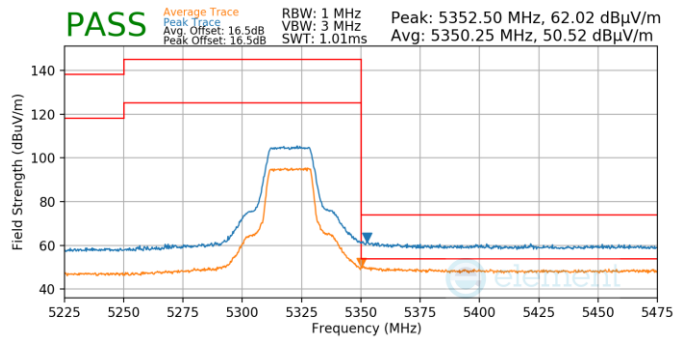
Plot 7-47. (Pk & Avg, Ch.64, 802.11n, MCS0)
