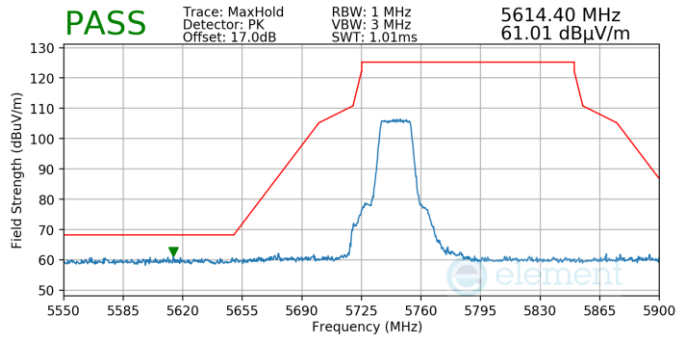
Plot 7-57. (Pk, Ch.149, 802.11n, MCS0)
