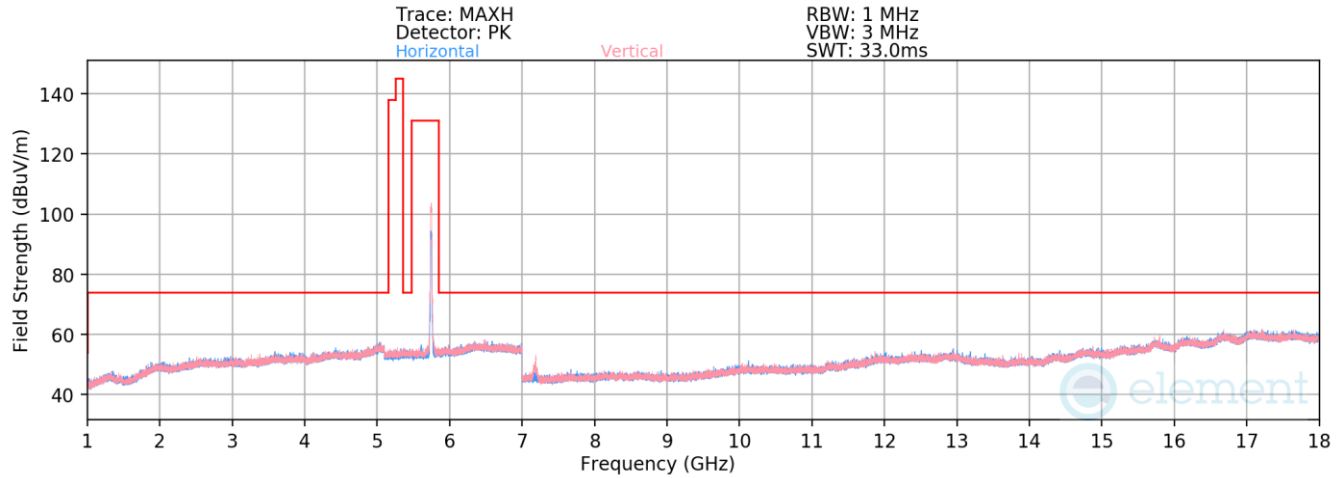
Plot 7-39. Radiated Spurious Emissions above 1GHz (802.11n – Ch. 149)
