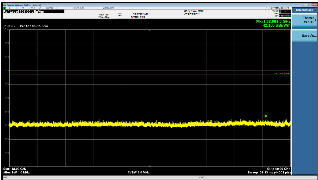
Plot 7-38. Radiated Spurious Emissions 18GHz-40GHz V Polarity (802.11n – Ch. 144)
