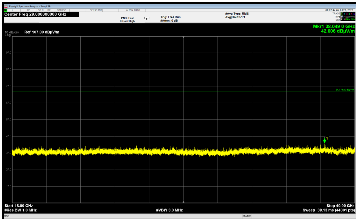
Plot 7-44. Radiated Spurious Emissions Simultaneous Transmission 18GHz – 40GHz Pol V
