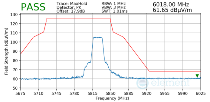
Plot 7-59. (Pk, Ch.165, 802.11n, MCS0)
