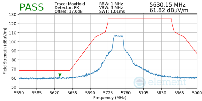
Plot 7-58. (Pk, Ch.149, 802.11n, MCS7)
