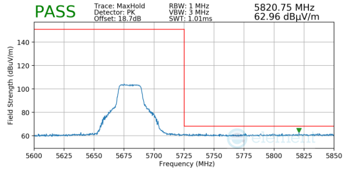
Plot 7-54. (Pk, Ch.136, 802.11n, MCS7)
