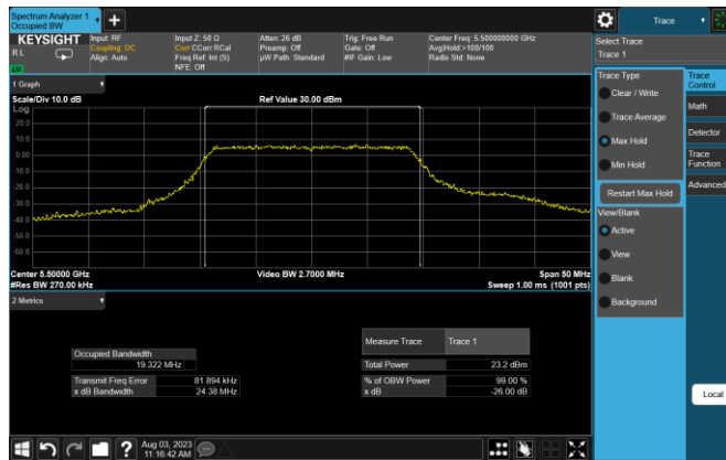
Plot 7-7. 26dB BW & 99% OBW (20MHz BW 802.11n – Ch. 100, MCS0)
