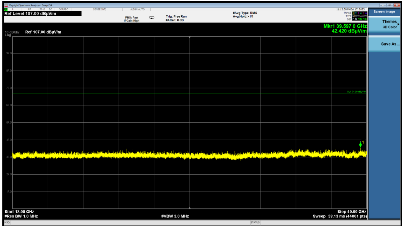
Plot 7-37. Radiated Spurious Emissions 18GHz-40GHz H Polarity (802.11n – Ch. 144)
