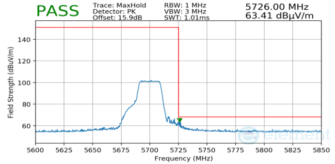
Plot 7-56. (Pk, Ch.140, 802.11n, MCS7)
