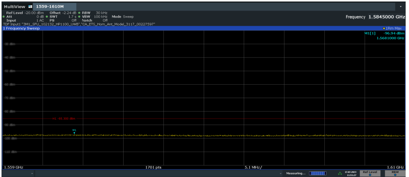
Plot 7-21. Radiated Spurious Emission 1559-1610MHz (Ch. 5, Config 409, Payload 4093 Ant. Pol. H)
