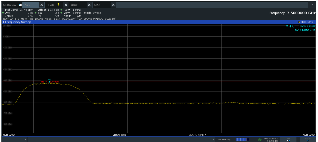
Plot 7-7. Average Radiated Power (Ch. 5, Config 409/Payload 4093)
