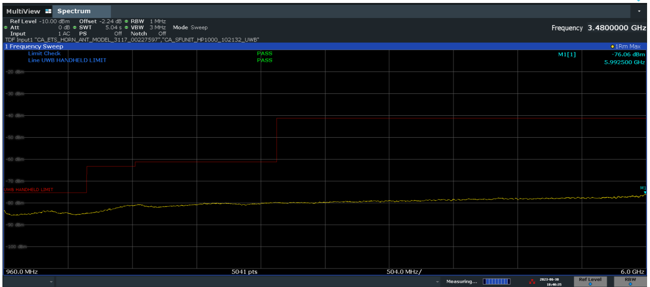
Plot 7-15. FCC Radiated Spurious Emission 960-6000MHz (Ch. 5, Config 409, Payload 4093 Ant. Pol. H)
