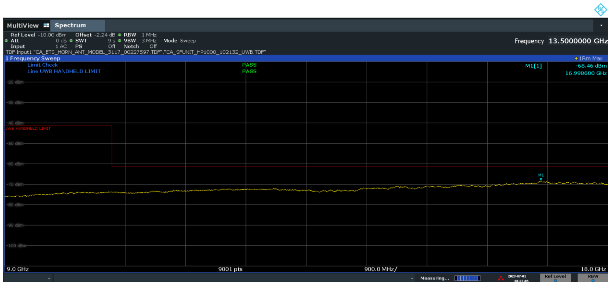
Plot 7-34. Radiated Spurious Emission 9-18GHz (Ch. 9, Config 409, Payload 4093 Ant. Pol. V)
