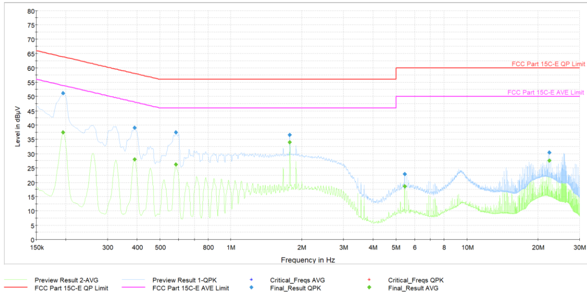
Plot 7-43. AC Line Conducted (Ch. 9, Config 409, Payload 4093 L1, with PC via USB-C cable with magnetic charger)
