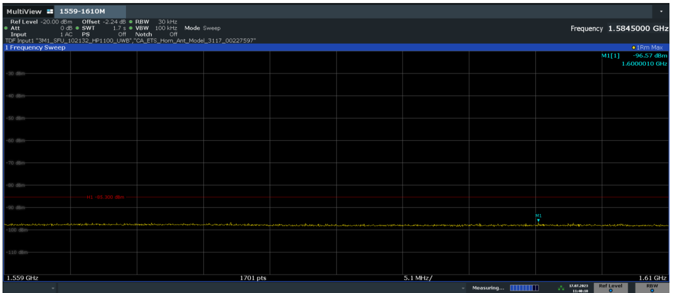
Plot 7-22. Radiated Spurious Emission 1559-1610MHz (Ch. 5, Config 409, Payload 4093 Ant. Pol. V)
