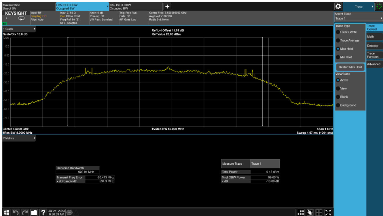
Plot 7-3. ISD 10dBc Occupied Bandwidth & 99% (Ch. 5, Config 409/Payload 4093)
