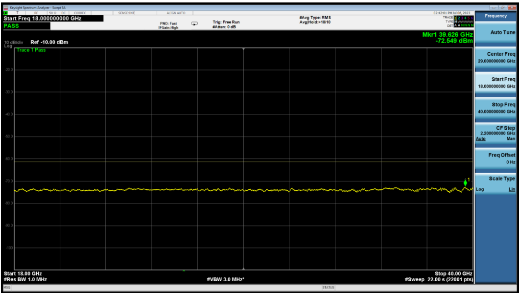
Plot 7-35. Radiated Spurious Emission 18-40GHz (Ch. 5, Config 409, Payload 4093 Ant. Pol. H)
