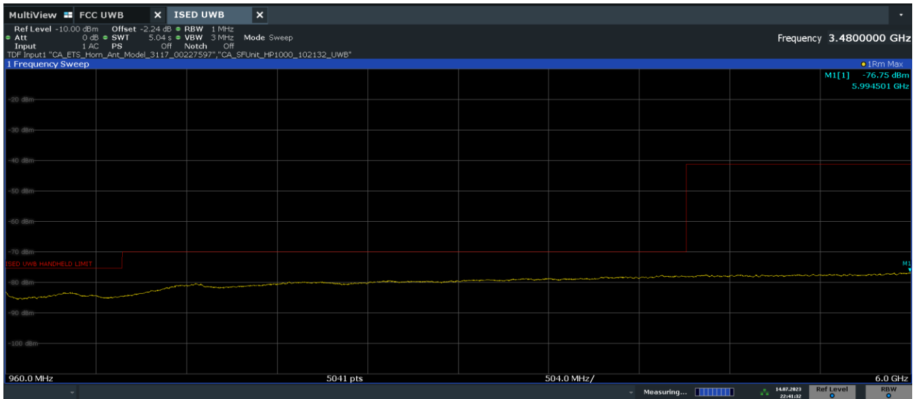
Plot 7-27. ISED Radiated Spurious Emission 960-6000MHz (Ch. 9, Config 409, Payload 4093 Ant. Pol. H)
