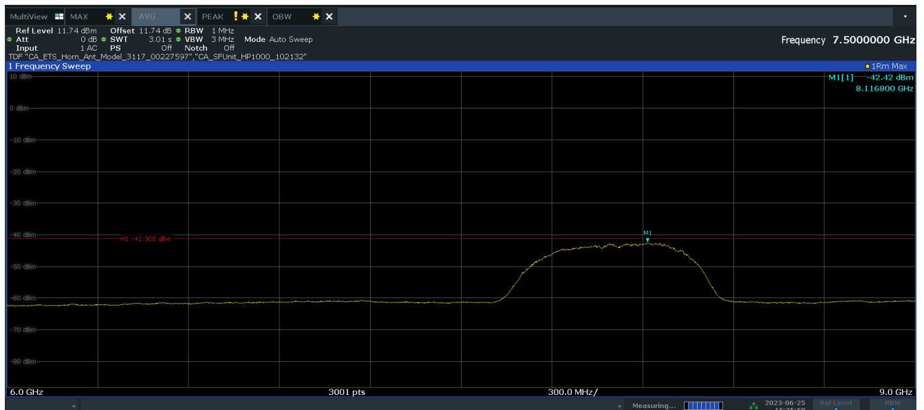
Plot 7-8. Average Radiated Power (Ch. 9, Config 409/Payload 4093)
