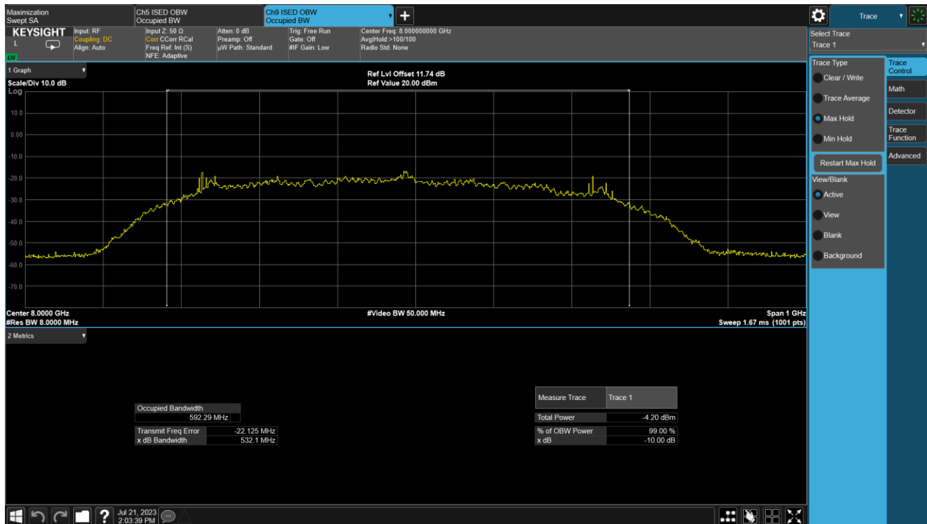
Plot 7-4. ISD 10dBc Occupied Bandwidth & 99 (Ch. 9, Config 409/Payload 4093)
