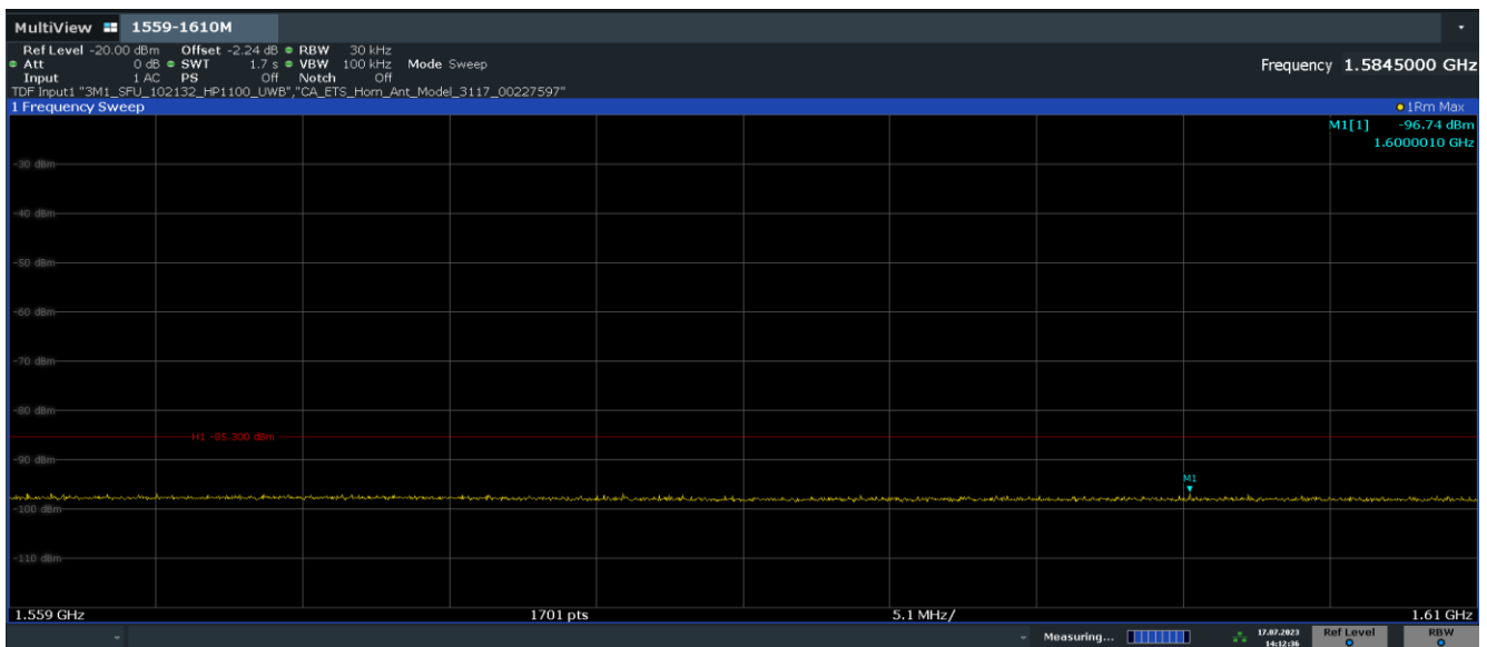
Plot 7-32. Radiated Spurious Emission 1559-1610MHz (Ch. 9, Config 409, Payload 4093 Ant. Pol. V)
