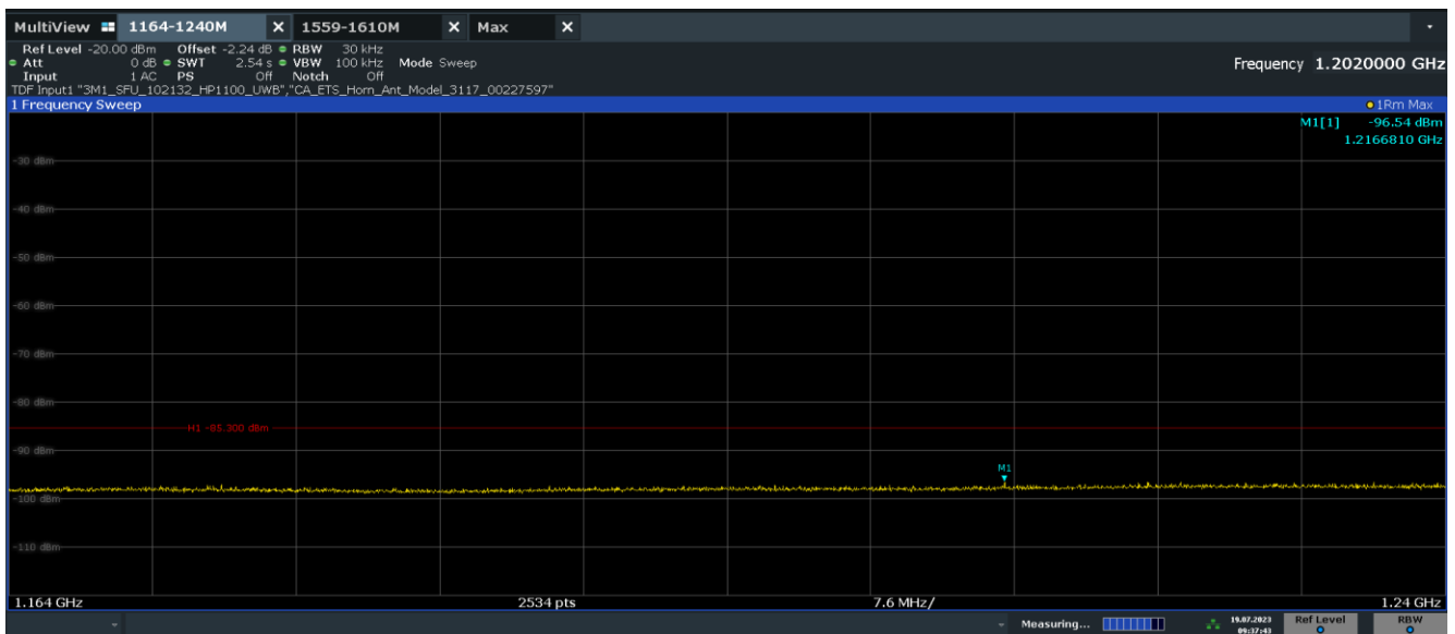
Plot 7-20. Radiated Spurious Emission 1164-1240MHz (Ch. 5, Config 409, Payload 4093 Ant. Pol. V)
