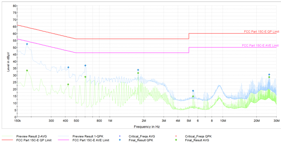
Plot 7-42. AC Line Conducted (Ch. 5, Config 409, Payload 4093 N, with PC via USB-C cable with magnetic charger)
