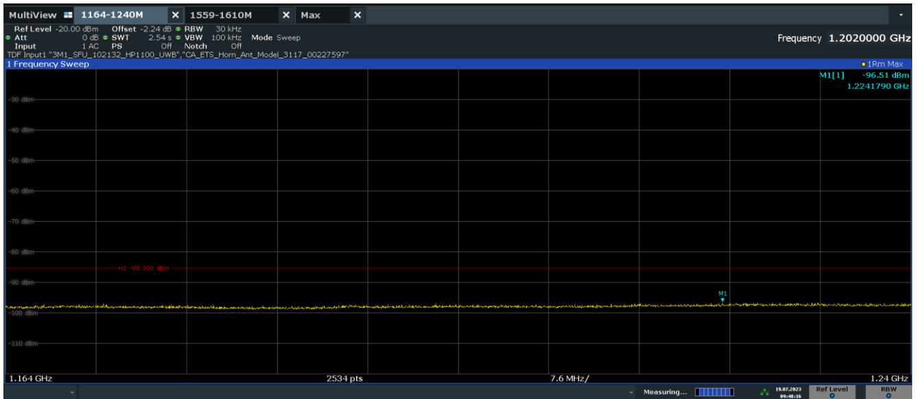
Plot 7-19. Radiated Spurious Emission 1164-1240MHz (Ch. 5, Config 409, Payload 4093 Ant. Pol. H)
