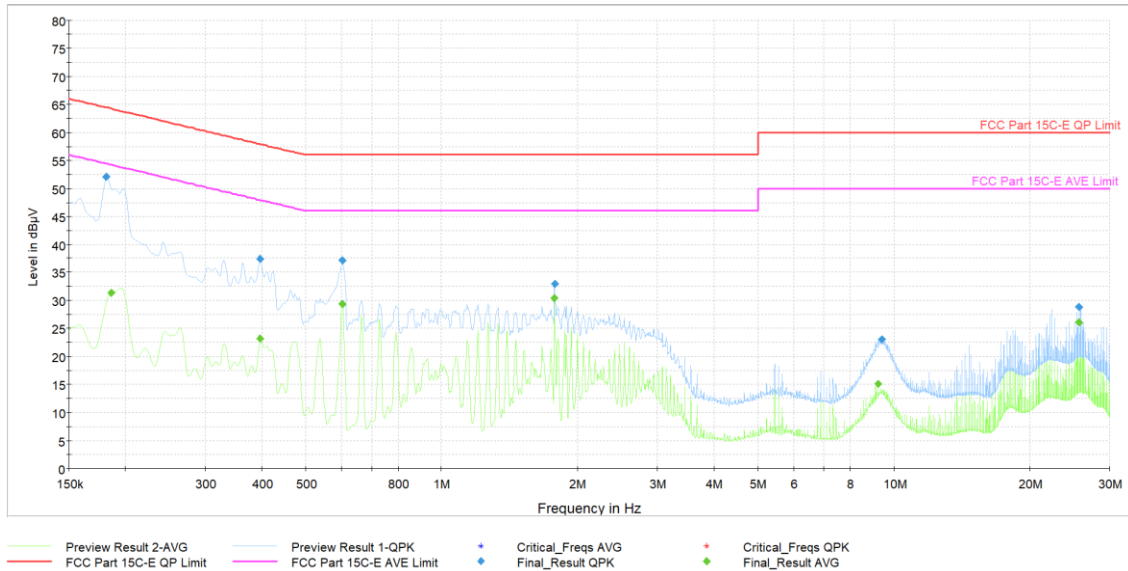
Plot 7-44. AC Line Conducted Plot (Ch. 9, Config 409, Payload 4093 N, with PC via USB-C cable with magnetic charger)
