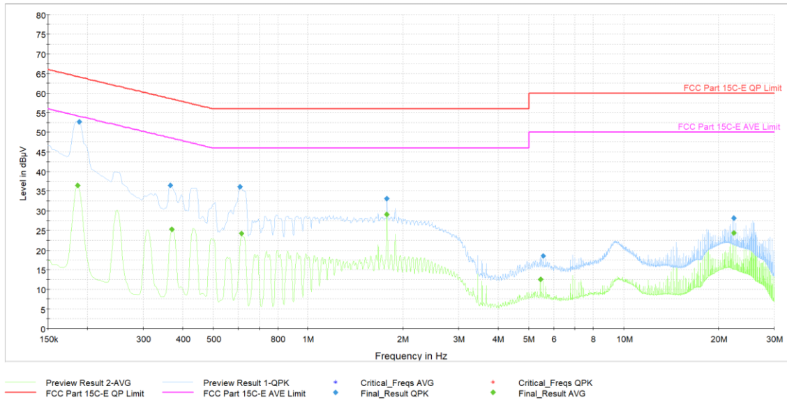
Plot 7-41. AC Line Conducted (Ch. 5, Config 409, Payload 4093 L1, with PC via USB-C cable with magnetic charger)
