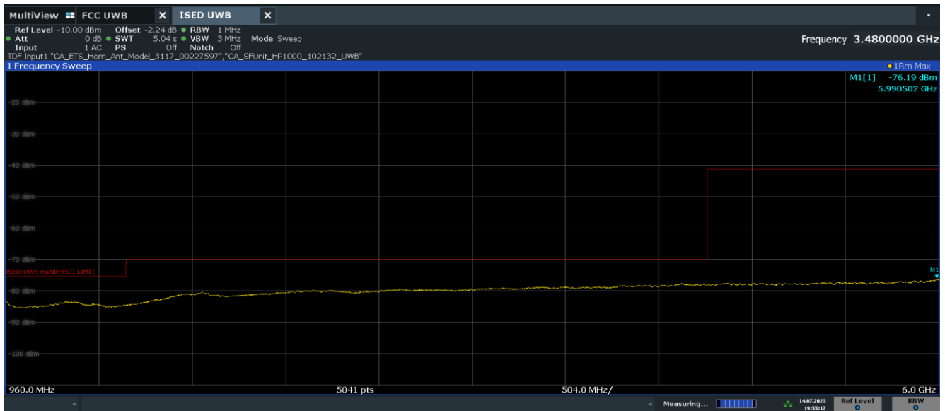
Plot 7-17. ISED Radiated Spurious Emission 960-6000MHz (Ch. 5, Config 409, Payload 4093 Ant. Pol. H)
