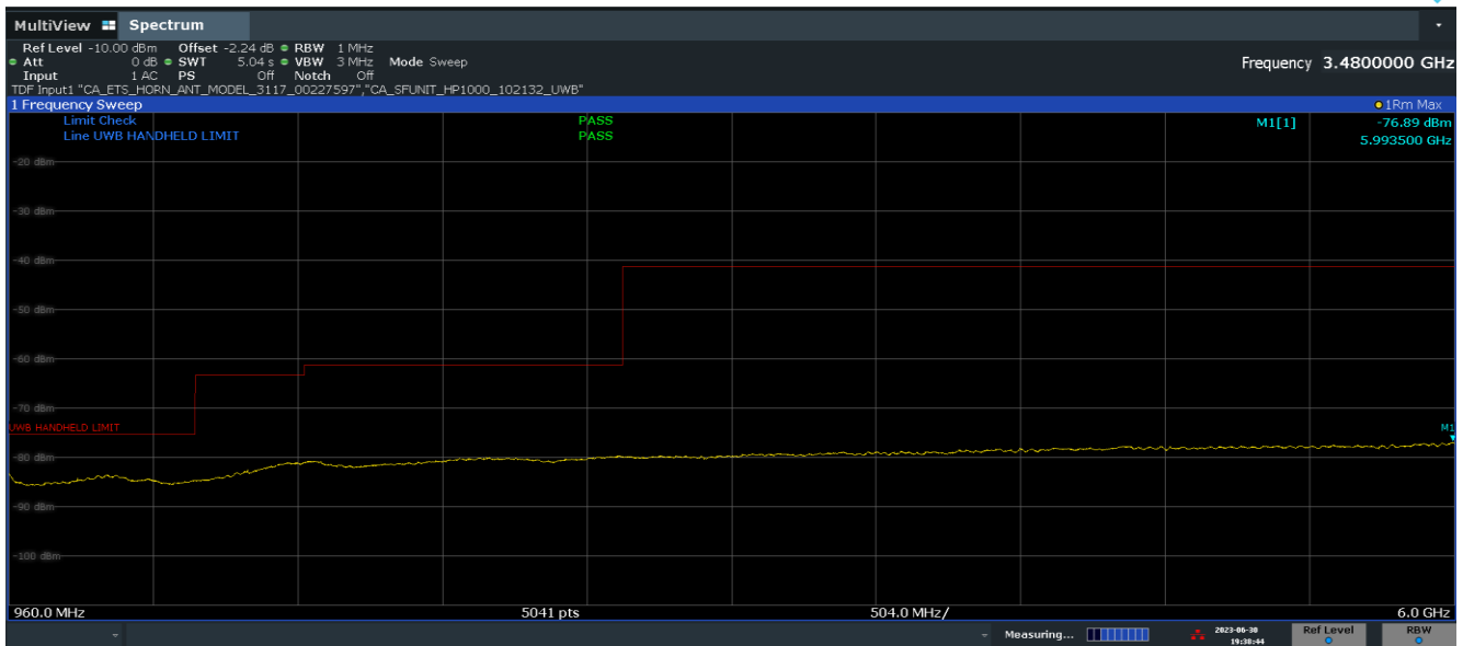
Plot 7-25. FCC Radiated Spurious Emission 960-6000MHz (Ch. 9, Config 409, Payload 4093 Ant. Pol. H)
