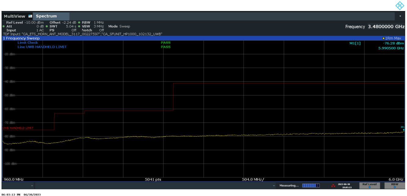
Plot 7-16. FCC Radiated Spurious Emissions 960-6000MHz (Ch. 5, Config 409, Payload 4093 Ant. Pol. V)
