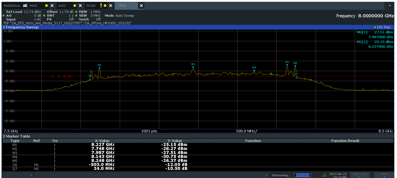
Plot 7-2. 10dBc Bandwidth (Ch. 9, Config 409/Payload 4093)
