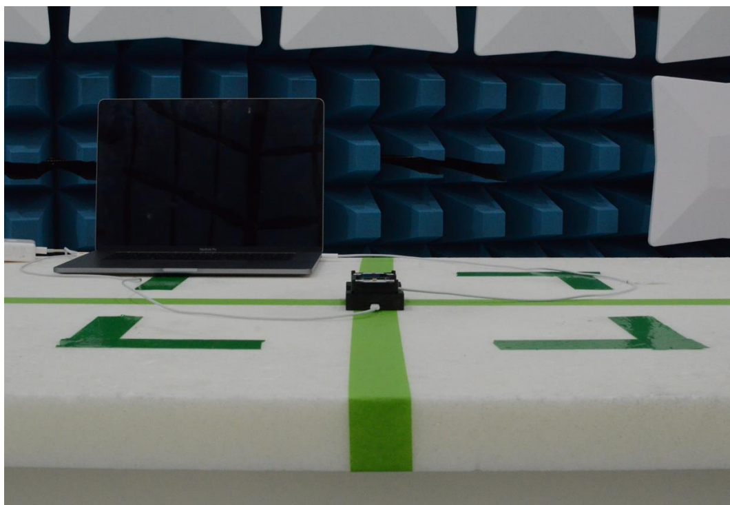
Figure 12: 30MHz-1GHz Test Setup (Front View)
