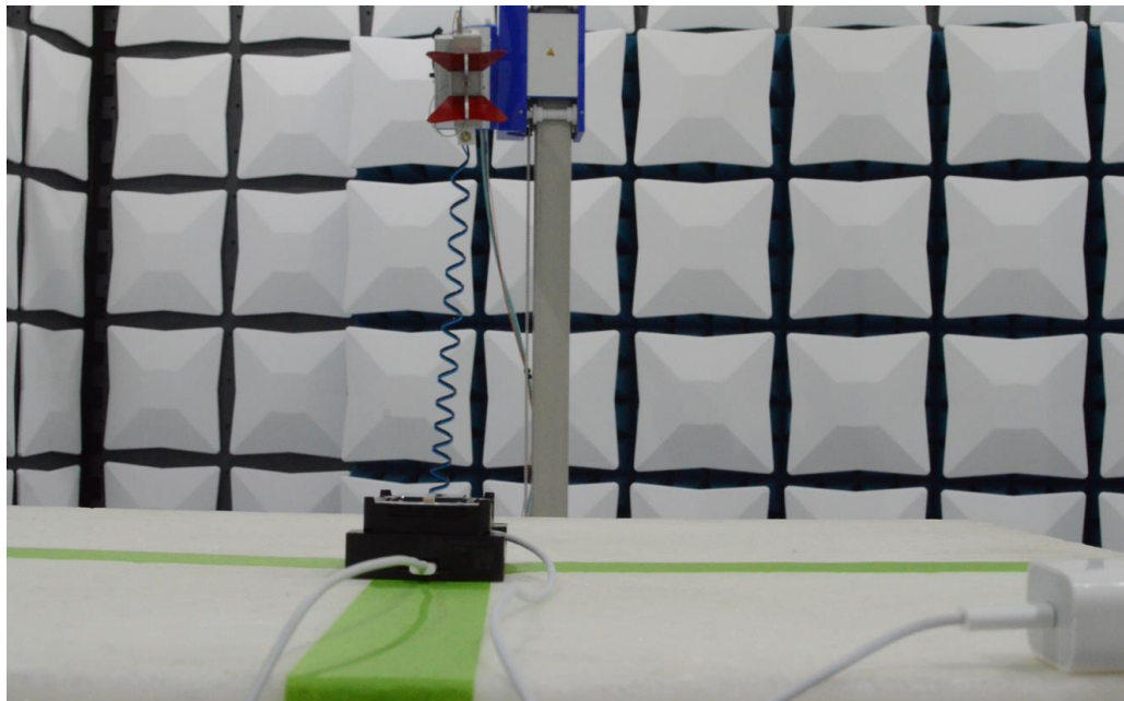
Figure 7: 1-18GHz Test Setup (Rear View)
