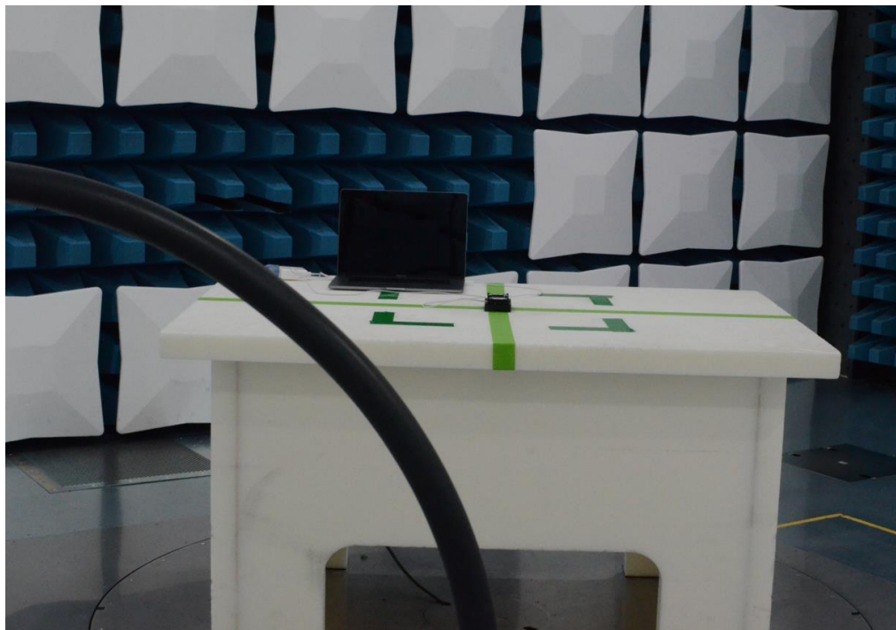
Figure 18: 9kHz-30MHz Test Setup (Front View)
