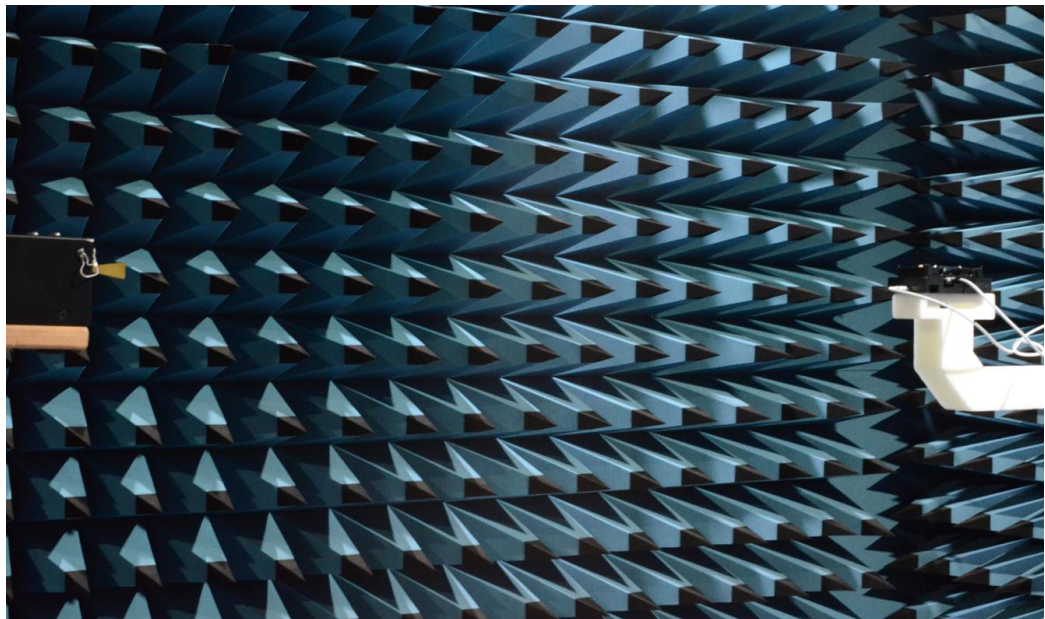
Figure 4: 90-140GHz Test Setup
