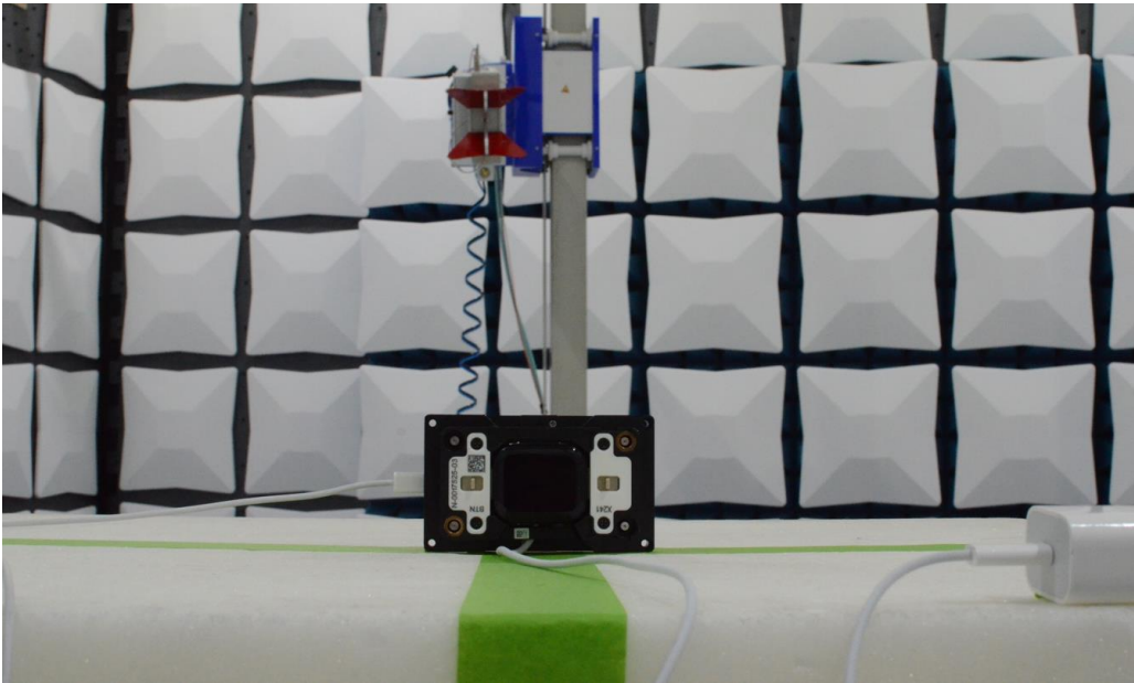
Figure 9: 1-18GHz Test Setup (Rear View)
