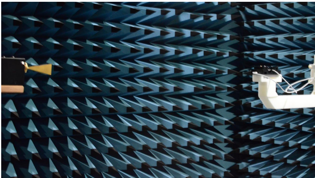
Figure 2: 40-60GHz Test Setup
