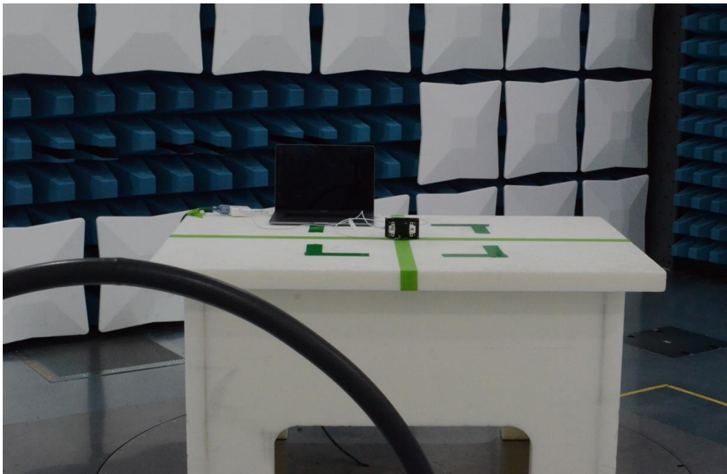
Figure 19: 9kHz-30MHz Test Setup (Front View)
