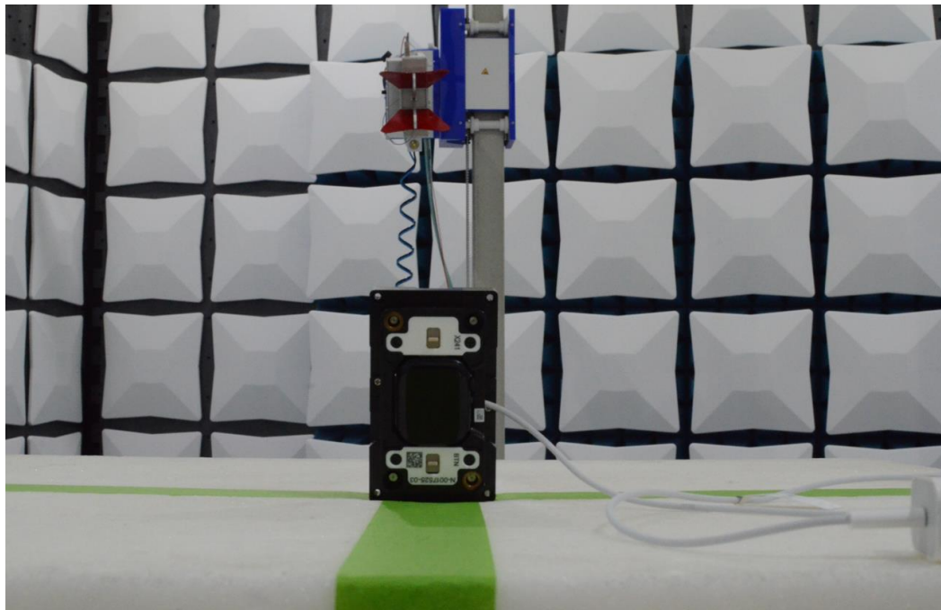
Figure 11: 1-18GHz Test Setup (Rear View)
