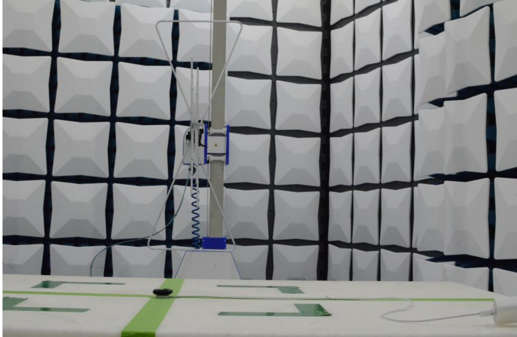
Figure 9: 30MHz-1GHz Test Setup (Rear View)
