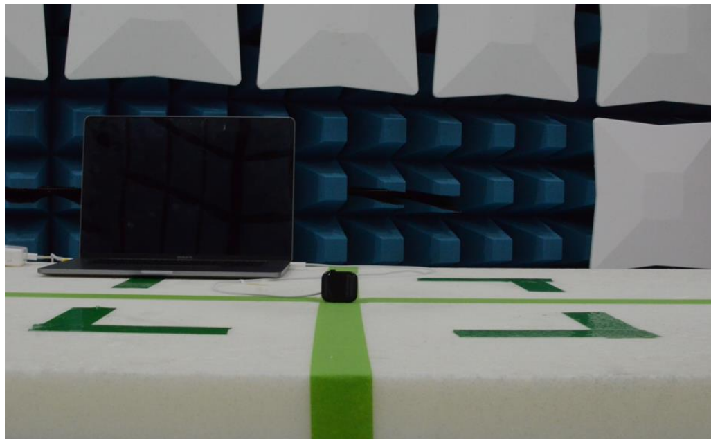
Figure 16: 30MHz-1GHz Test Setup (Front View)
