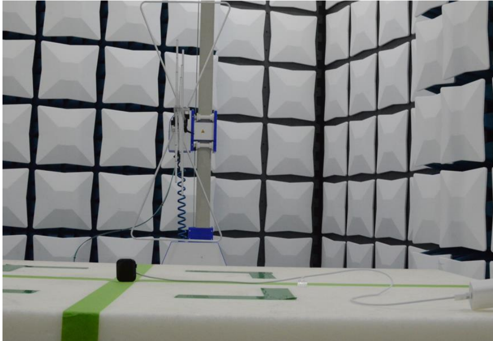
Figure 13: 30MHz-1GHz Test Setup (Rear View)
