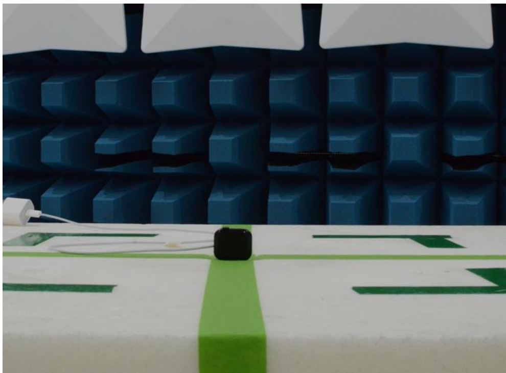
Figure 10: 30MHz-1GHz Test Setup (Front View)
