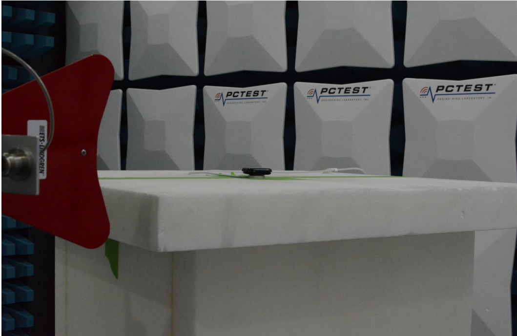
Figure 5: Above 960MHz Test Setup
