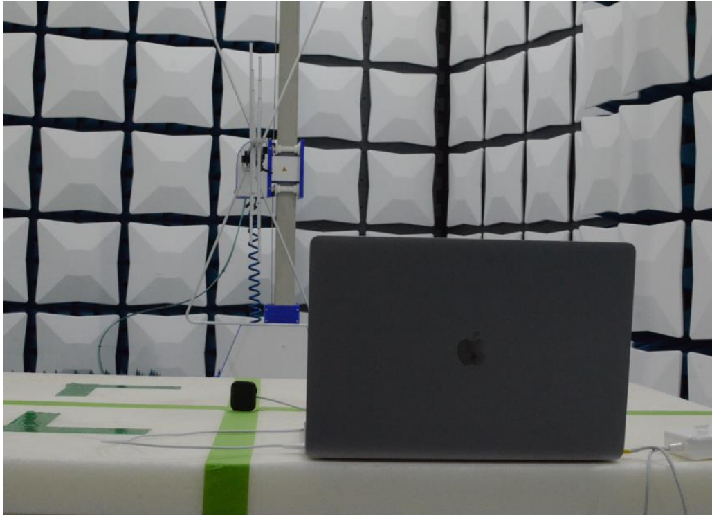
Figure 19: 30MHz-1GHz Test Setup (Rear View)
