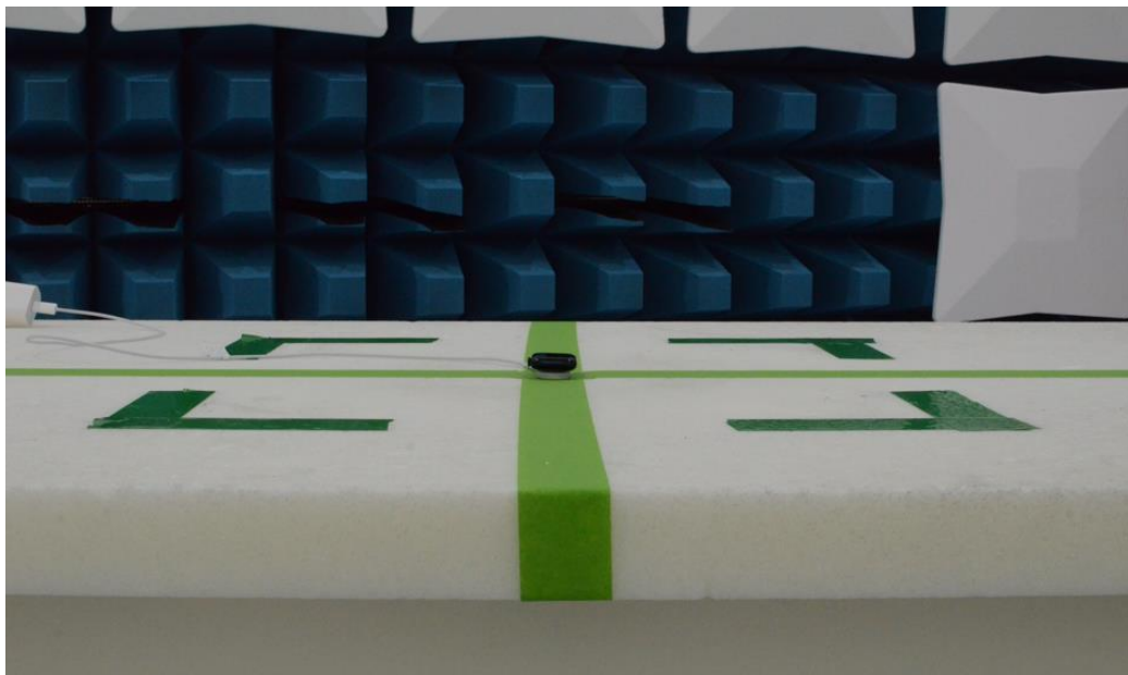
Figure 8: 30MHz-1GHz Test Setup (Front View)
