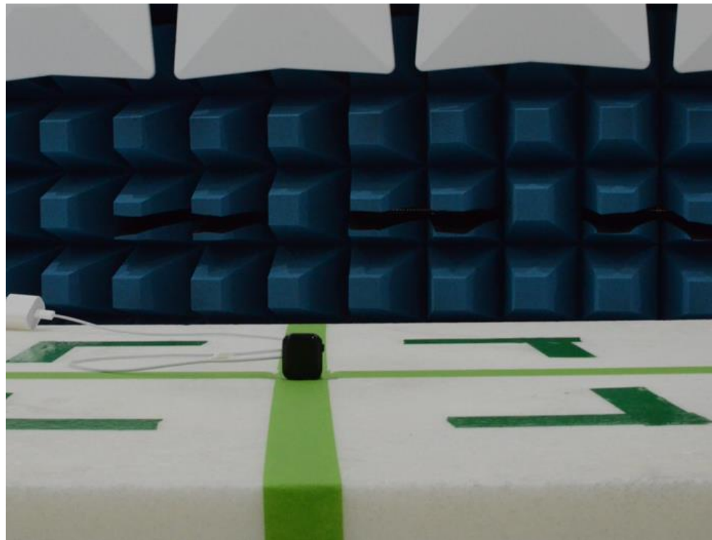
Figure 12: 30MHz-1GHz Test Setup (Front View)
