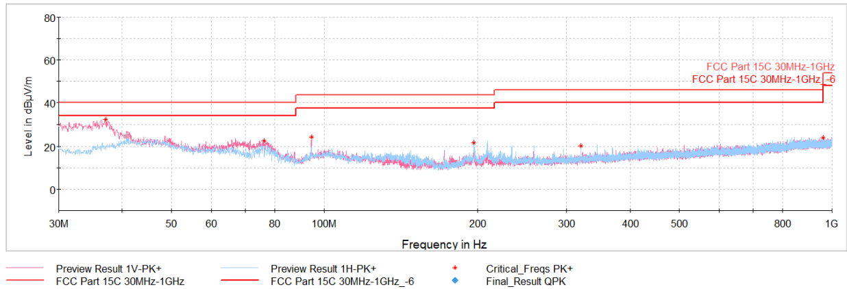
Plot 7-38. Radiated Spurious Emissions Below 1GHz (HDR4 ePA – Ch.38 with AC/DC Adapter + Magnetic Charger)
