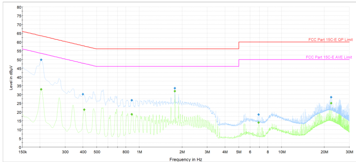
Plot 7-39. AC Line Conducted Plot with Bluetooth HDR (L1, 4Mbps ePA - Ch.38 with Laptop + Magnetic Charger)
