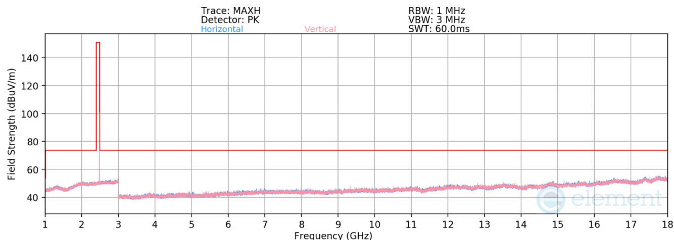
Plot 7-31. Radiated Spurious Emissions 1-18GHz (1Mbps ePA – Ch. 39, Ant. Pol. H & V)
