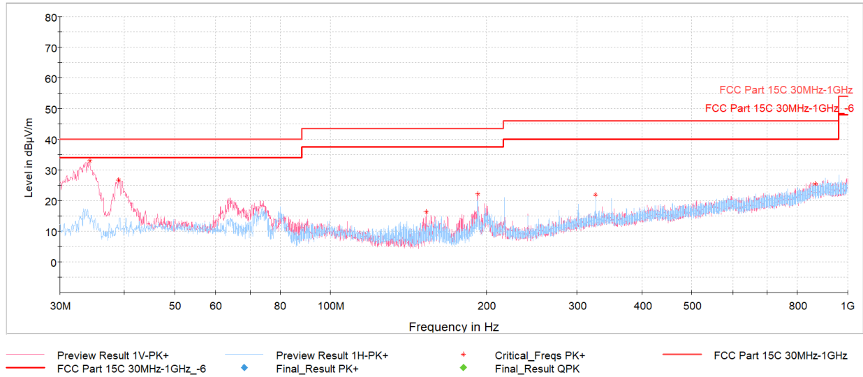
Plot 7-38. Radiated Spurious Emissions Below 1GHz (1Mbps, ePA – Ch.19, Pol. H & V, with AC/DC Adapter + Magnetic Charger)
