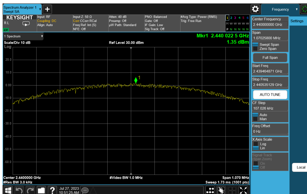
Plot 7-8. Power Spectral Density Plot (Bluetooth (LE), 1Mbps, ePA – Ch. 19)
