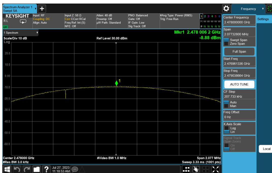
Plot 7-18. Power Spectral Density Plot (Bluetooth (LE), 2Mbps, iPA – Ch. 38)
