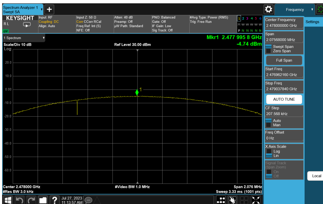
Plot 7-15. Power Spectral Density Plot (Bluetooth (LE), 2Mbps, ePA – Ch. 38)
