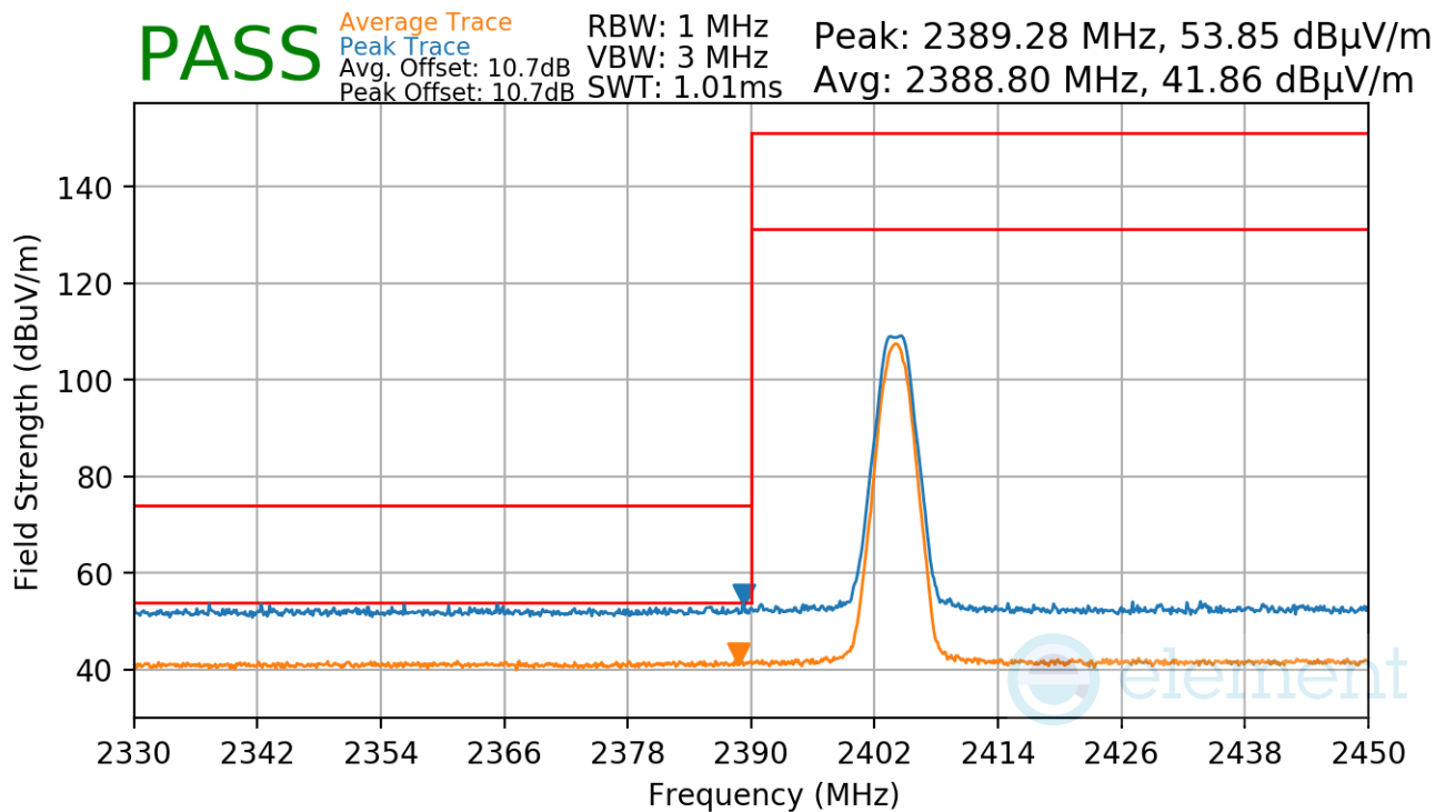
Plot 7-36. Radiated Restricted Lower Band Edge Measurement
