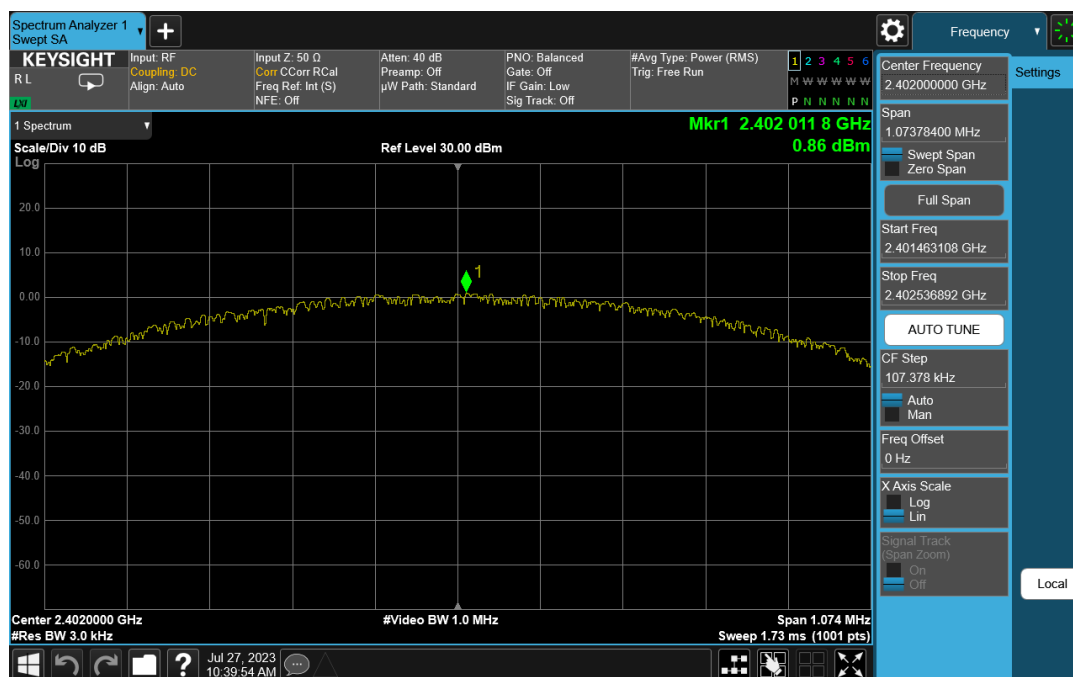
Plot 7-7. Power Spectral Density Plot (Bluetooth (LE), 1Mbps, ePA – Ch. 0)
