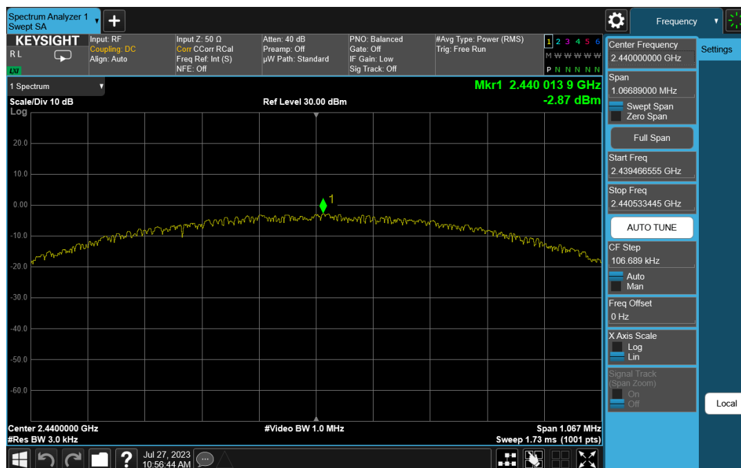
Plot 7-11. Power Spectral Density Plot (Bluetooth (LE), 1Mbps, iPA – Ch. 19)
