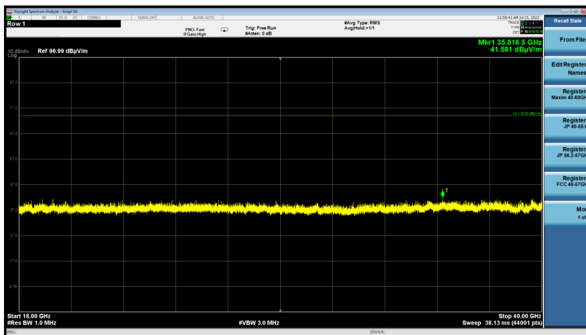
Plot 7-32. Radiated Spurious Emissions above 18GHz (1Mbps ePA – Ch.19, Pol.H)
