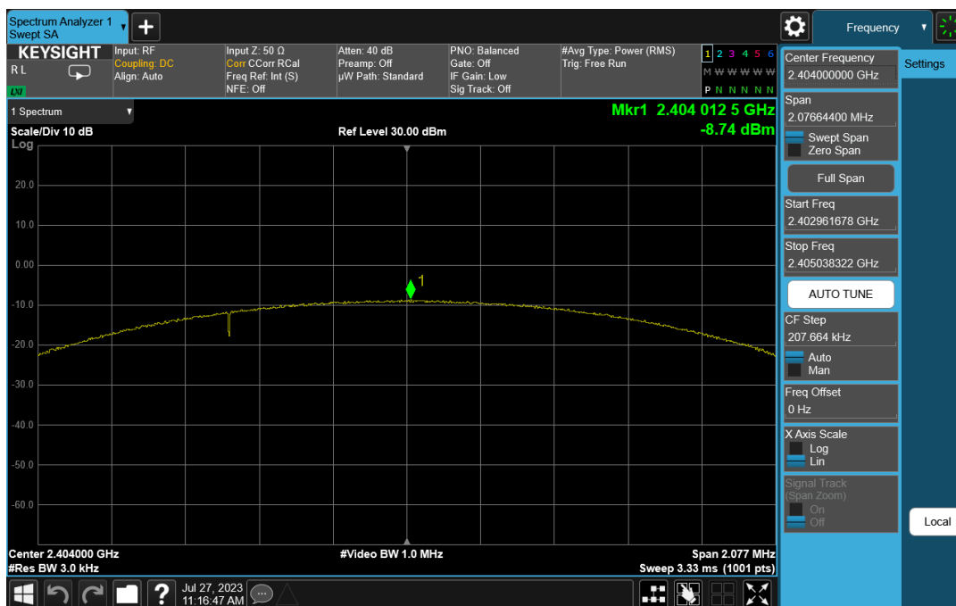
Plot 7-16. Power Spectral Density Plot (Bluetooth (LE), 2Mbps, iPA – Ch. 1)
