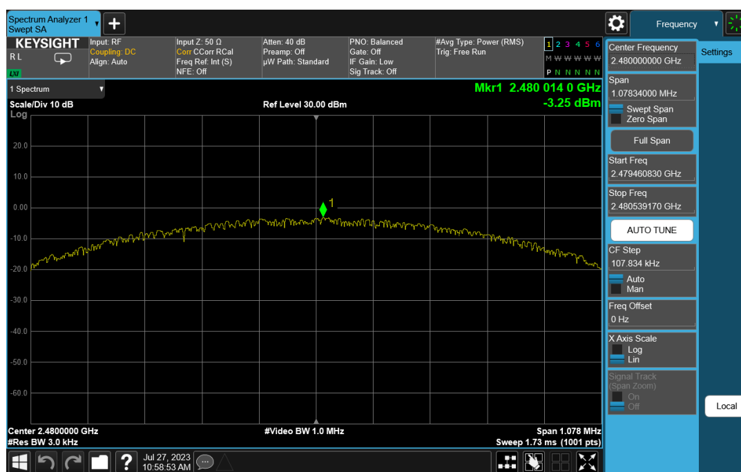
Plot 7-12. Power Spectral Density Plot (Bluetooth (LE), 1Mbps, iPA – Ch. 39)
