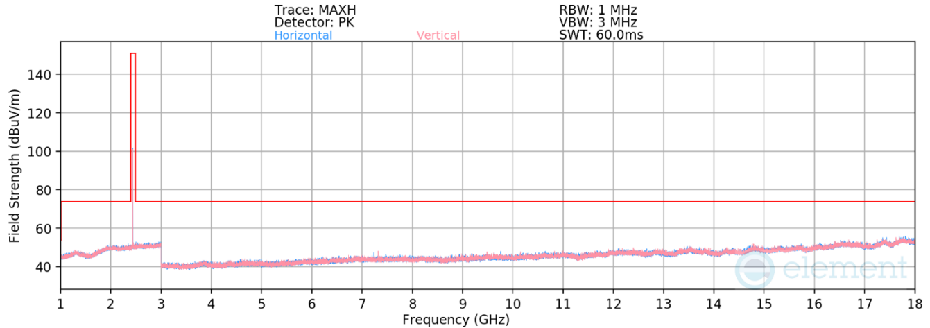
Plot 7-30. Radiated Spurious Emissions 1-18GHz (1Mbps, ePA – Ch. 19, Ant. Pol. H & V)
