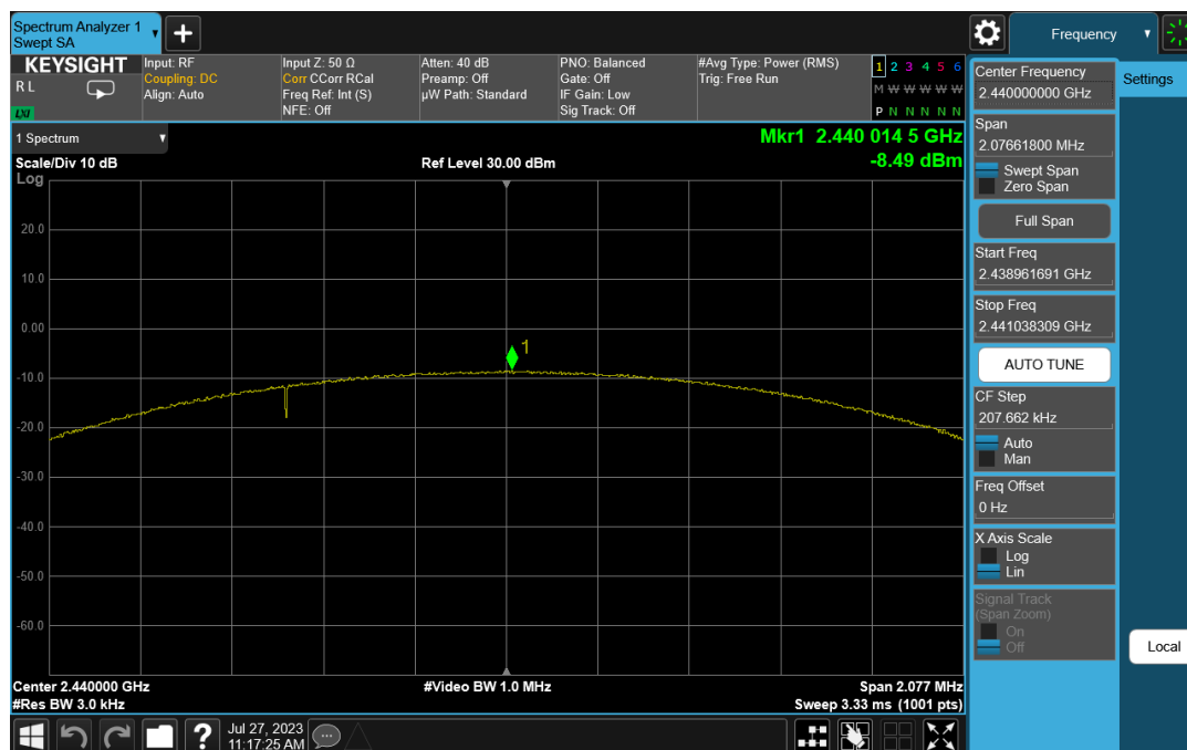
Plot 7-17. Power Spectral Density Plot (Bluetooth (LE), 2Mbps, iPA – Ch. 19)
