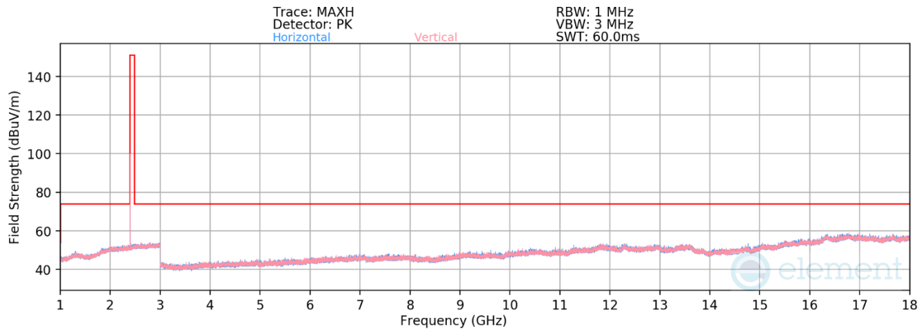
Plot 7-29. Radiated Spurious Emissions 1-18GHz (1Mbps, ePA – Ch. 0, Ant. Pol. H & V)
