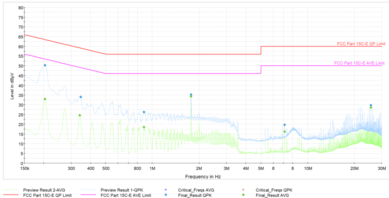
Plot 7-40. AC Line Conducted Plot with Bluetooth LE (N, 1Mbps ePA – Ch.19 with Laptop & Magnetic Charger)
