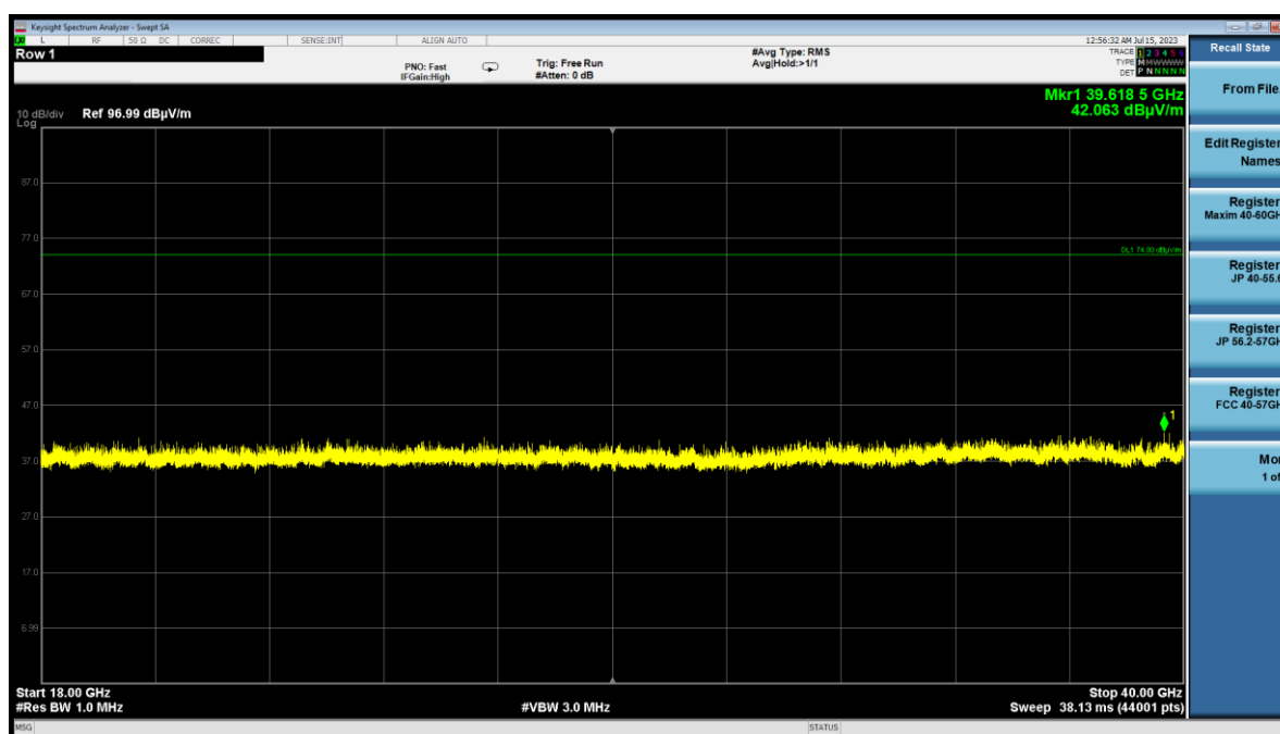
Plot 7-33. Radiated Spurious Emissions above 18GHz (1Mbps ePA – Ch.19, Pol V)
