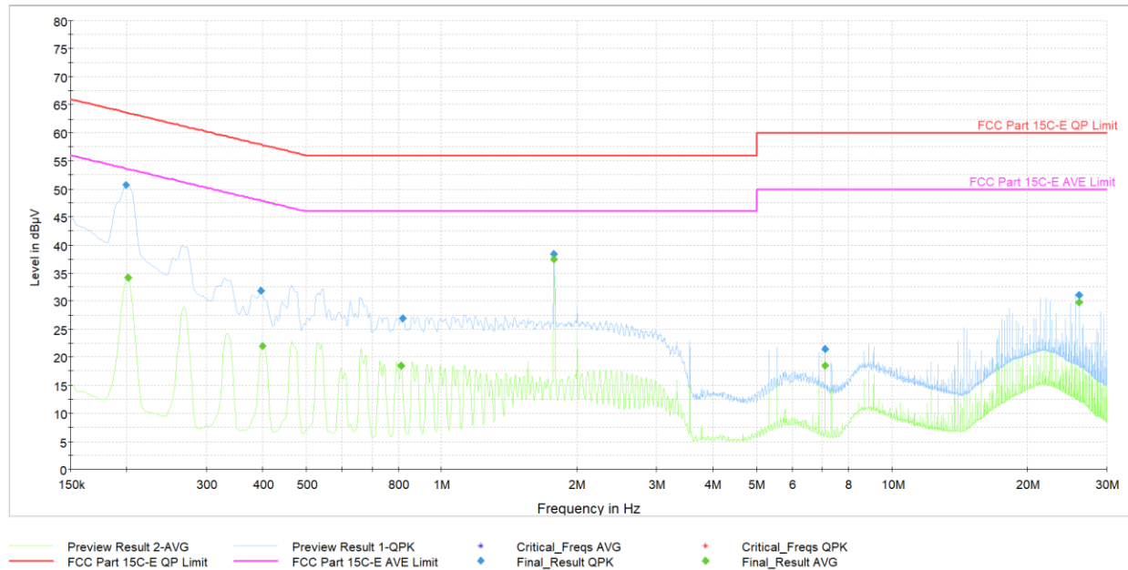
Plot 7-39. AC Line Conducted Plot with Bluetooth LE (L1, 1Mbps ePA – Ch.19 with Laptop & Magnetic Charger)
