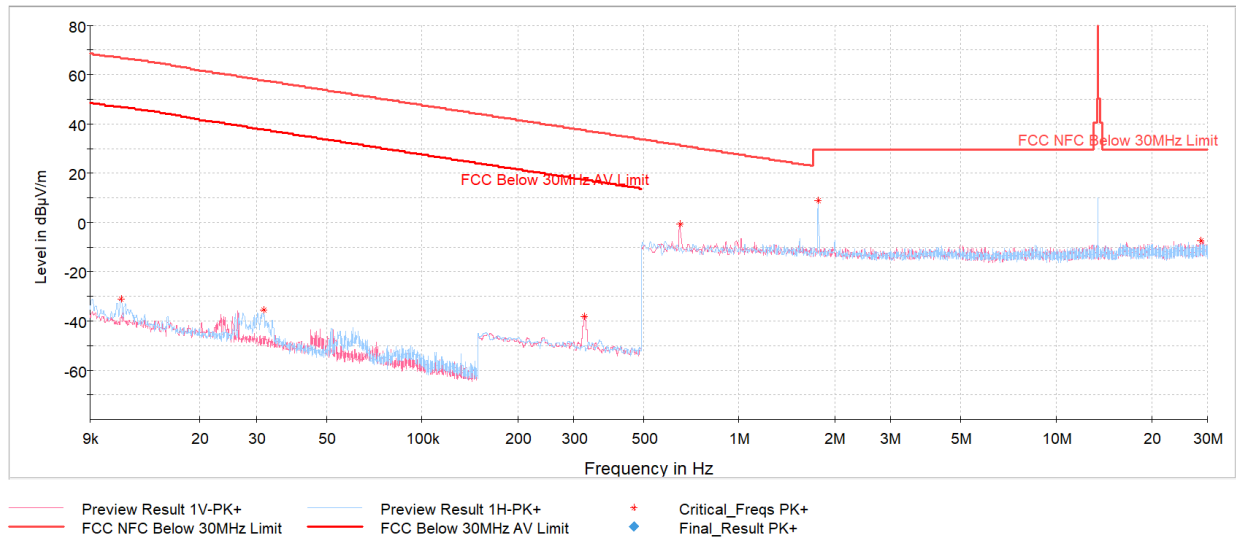
Plot 7-8. Radiated Spurious Emissions 9kHz – 30MHz (CE B 848kbps, with AC/DC Adapter and Magnetic Charger)
