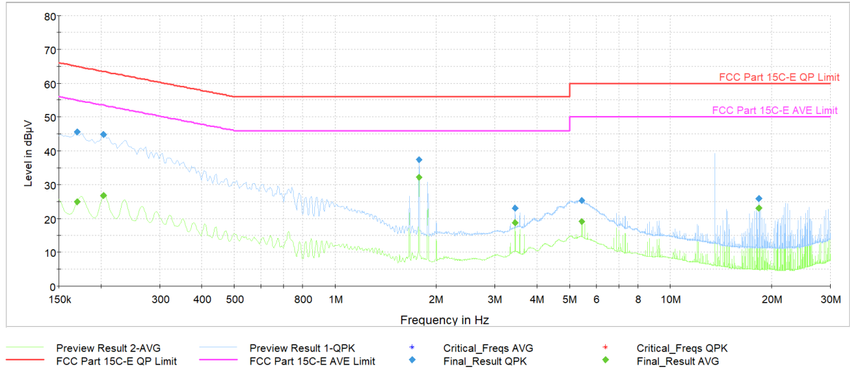
Plot 7-12. AC Line-Conducted Plot (L1, CE B 848kbps, with AC/DC Adapter and Magnetic Charger)
