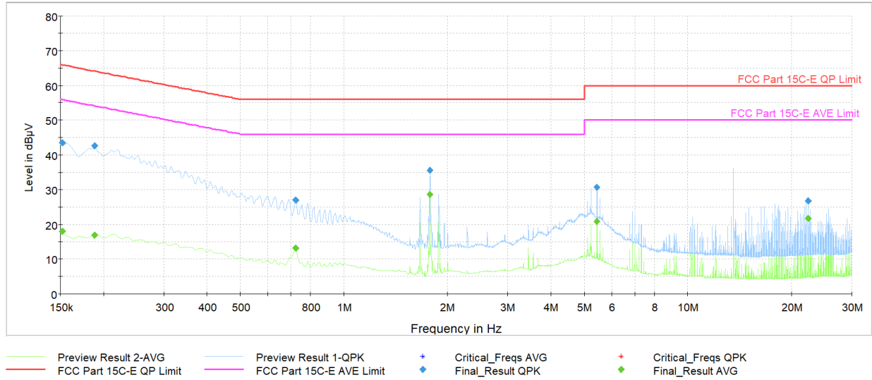
Plot 7-13. AC Line-Conducted Plot (N, CE B 848kbps, with AC/DC Adapter and Magnetic Charger)
