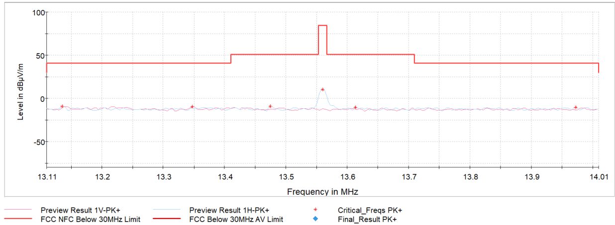
Plot 7-6. In Band Radiated Spurious Emissions (CE B 848kbps, with AC/DC Adapter and Magnetic Charger)
