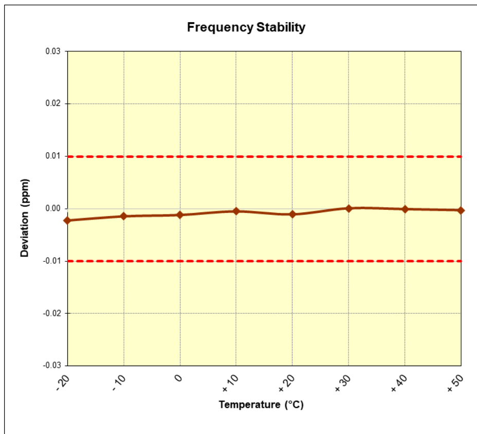
Figure 7-3. Frequency Stability Plot (CE B 848kbps)
