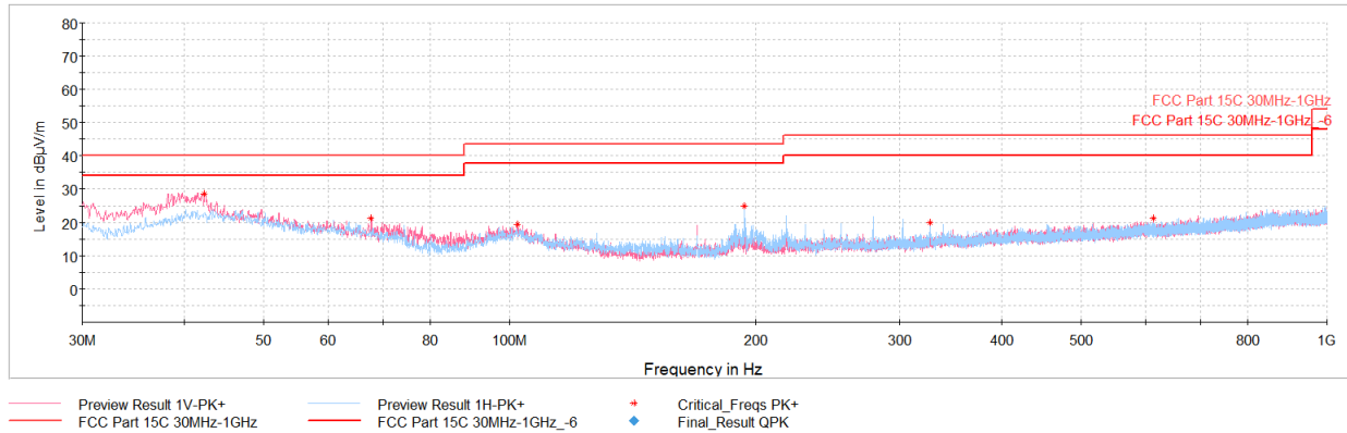
Plot 7-10. Radiated Spurious Emissions 30MHz – 1GHz (CE B 848kbps, with AC/DC Adapter and Magnetic Charger)
