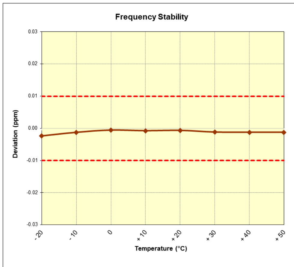
Figure 7-4. Frequency Stability Plot (Reader 10% ASK 1 out of 4)
