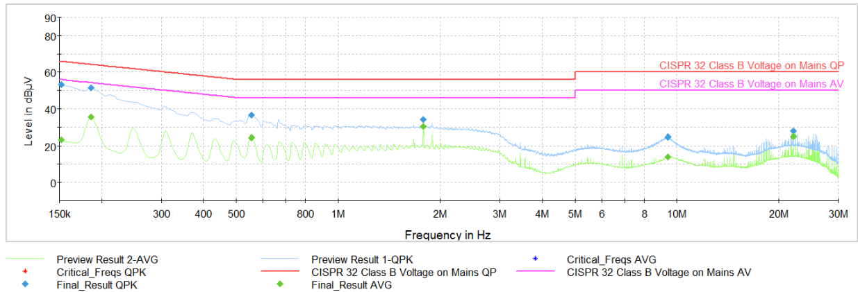
Plot 6-13. AC Line Conducted Plot (L1 - Mode 1, with Magnetic Charger & Laptop)
