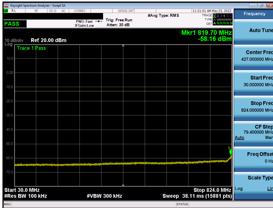
Plot 7-16. Conducted Spurious Plot (LTE Band 26/5 - 10MHz QPSK - RB Size 1, RB Offset 0 - High Channel)
