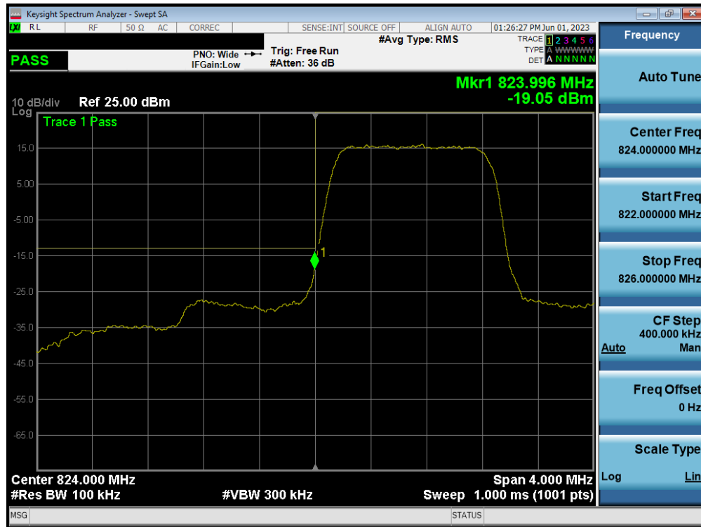
Plot 7-28. Lower BE Plot (LTE Band 26 – 1.4MHz QPSK – Full RB Configuration)
