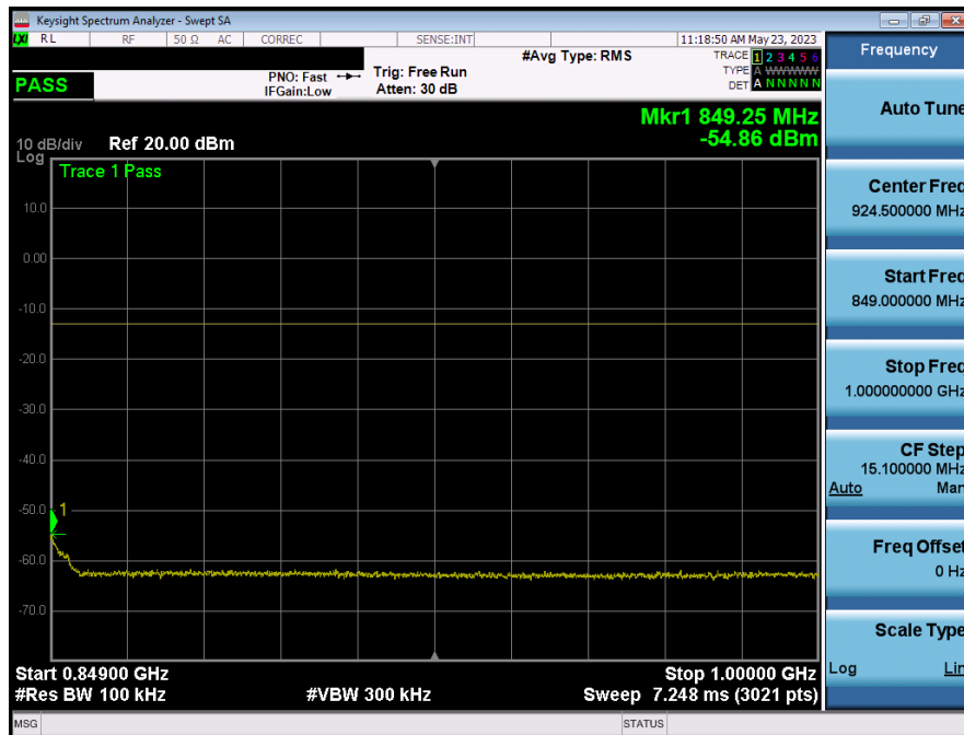
Plot 7-11. Conducted Spurious Plot (LTE Band 26/5 - 10MHz QPSK - RB Size 1, RB Offset 0 - Low Channel)
