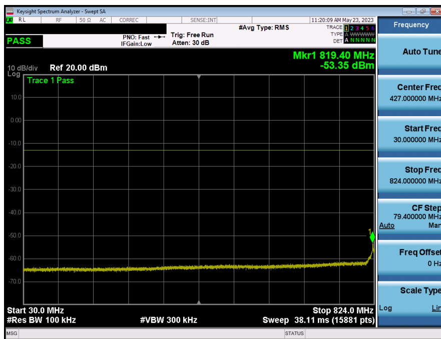
Plot 7-13. Conducted Spurious Plot (LTE Band 26/5 - 10MHz QPSK - RB Size 1, RB Offset 0 - Mid Channel)
