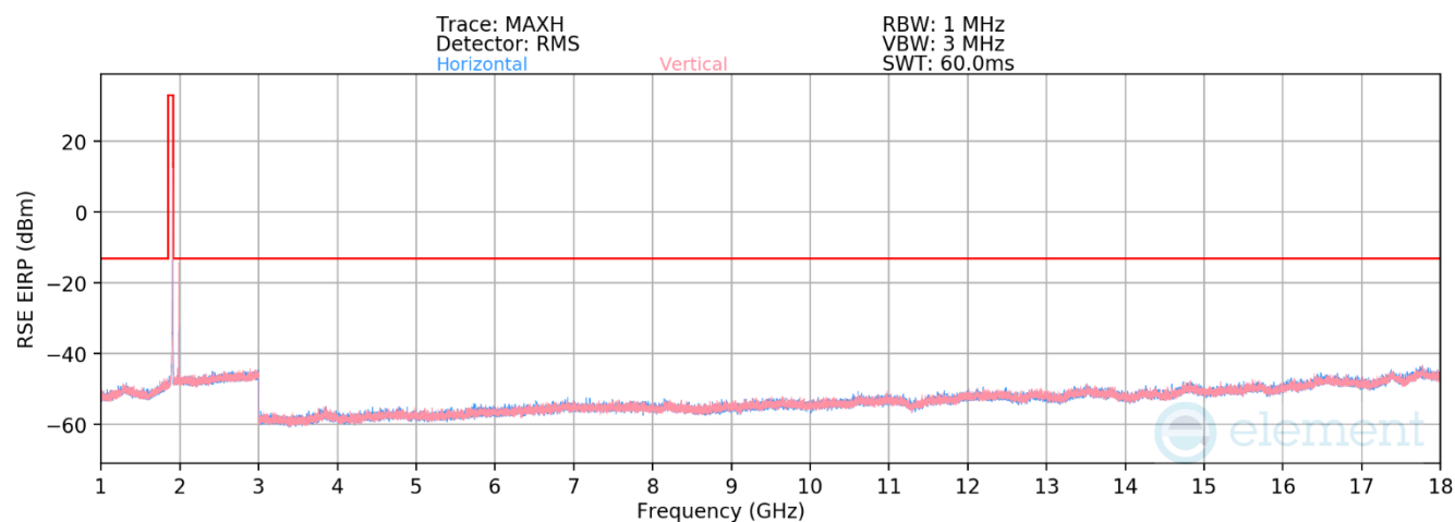
Plot 7-110. Antenna FCM Radiated Spurious Plot (WCDMA PCS)
