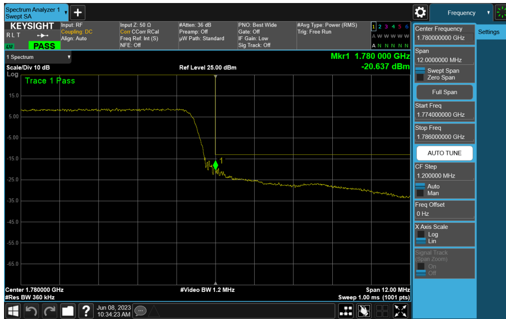
Plot 7-74. Upper Band Edge Plot (LTE Band 66 - 15MHz QPSK – Full RB)
