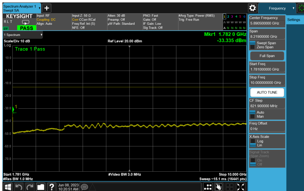
Plot 7-33. Conducted Spurious Plot (LTE Band 66/4 - 20MHz QPSK - RB Size 1, RB Offset 0 - High Channel)
