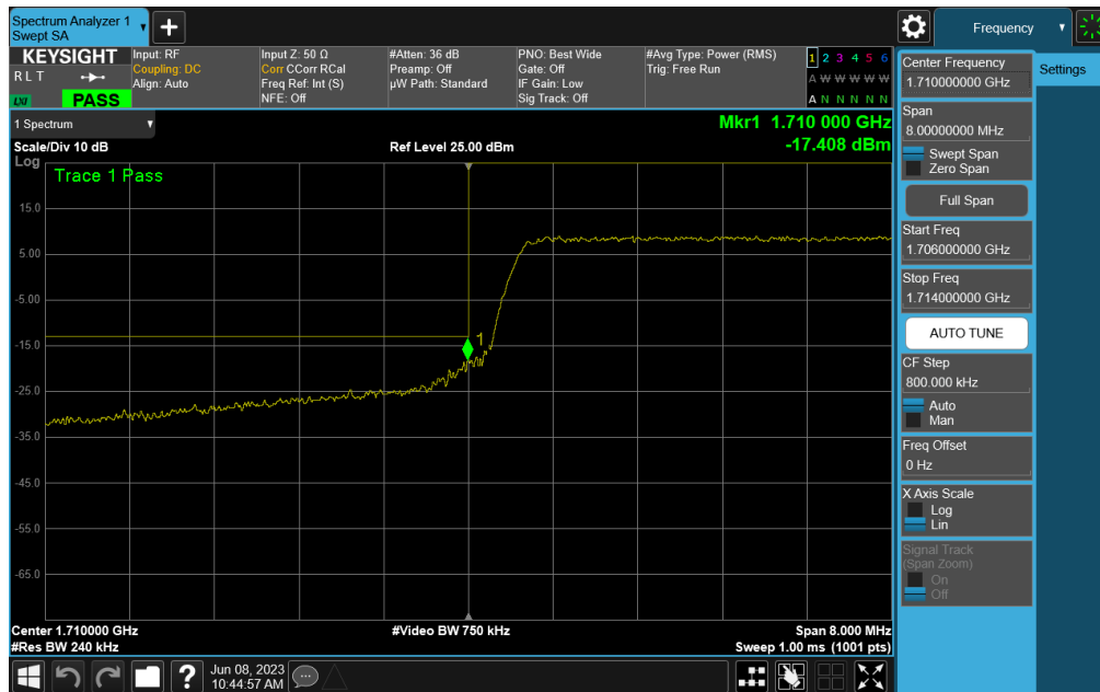
Plot 7-68. Lower Band Edge Plot (LTE Band 66 - 10MHz QPSK – Full RB)
