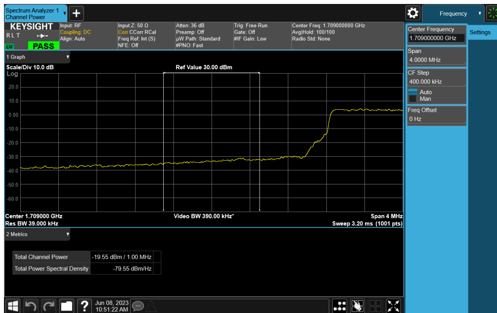
Plot 7-65. Lower Extended Band Edge Plot (LTE Band 66 - 5MHz QPSK – Full RB)
