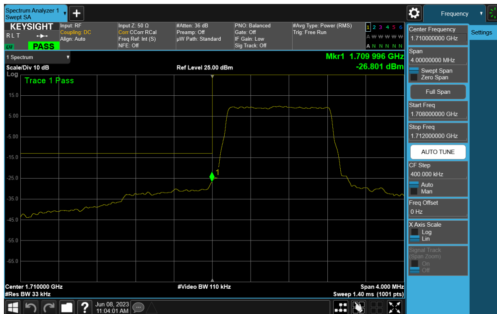
Plot 7-56. Lower Band Edge Plot (LTE Band 66 – 1.4MHz QPSK – Full RB)
