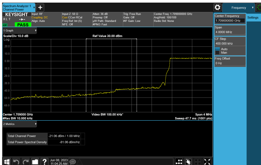
Plot 7-57. Lower Extended Band Edge Plot (LTE Band 66 – 1.4MHz QPSK – Full RB)
