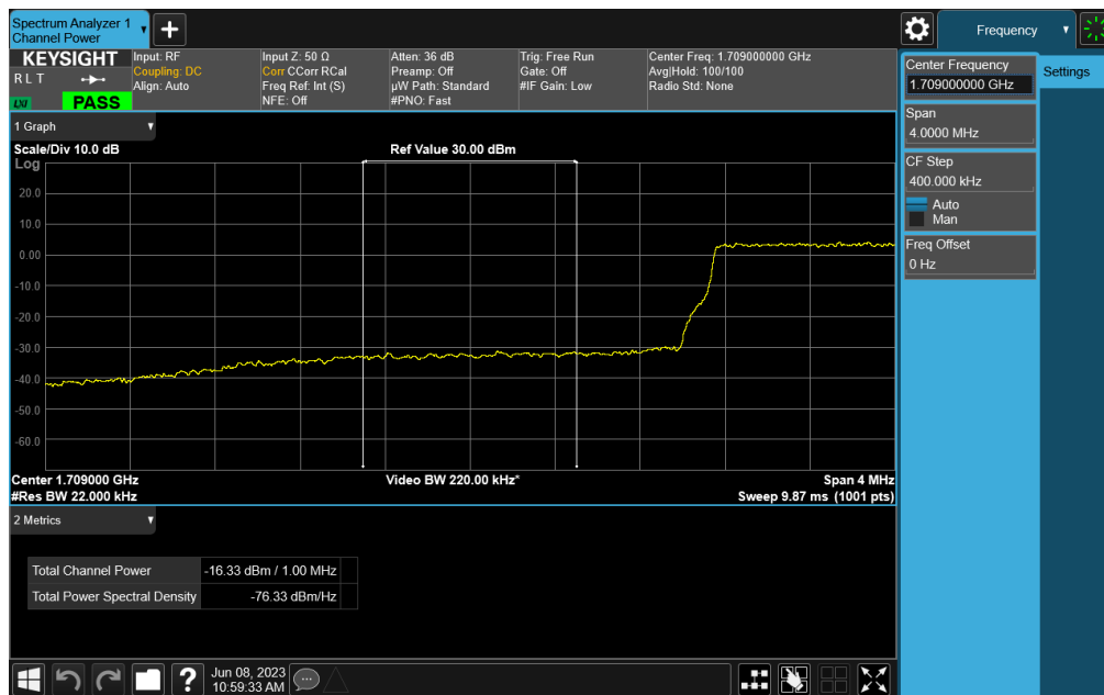
Plot 7-61. Lower Extended Band Edge Plot (LTE Band 66 - 3MHz QPSK – Full RB)
