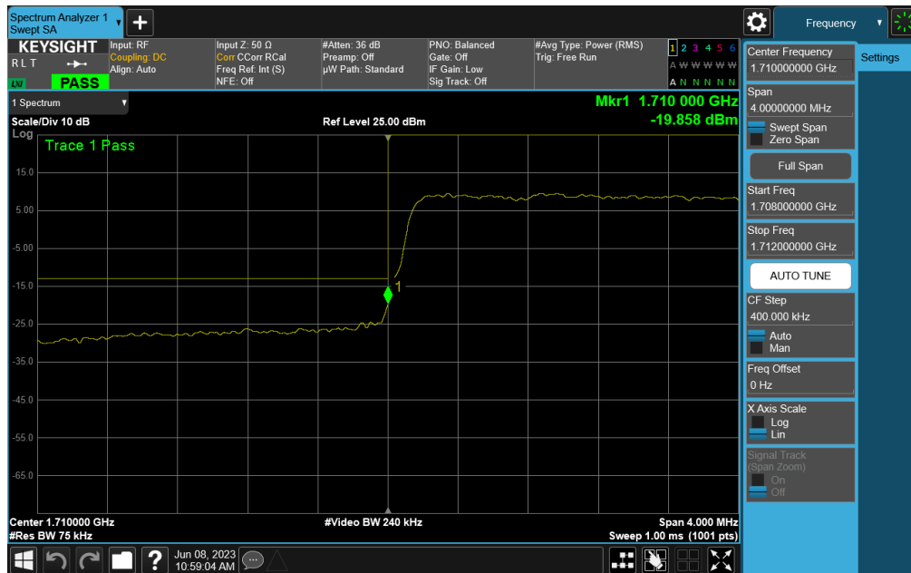
Plot 7-60. Lower Band Edge Plot (LTE Band 66 - 3MHz QPSK – Full RB)
