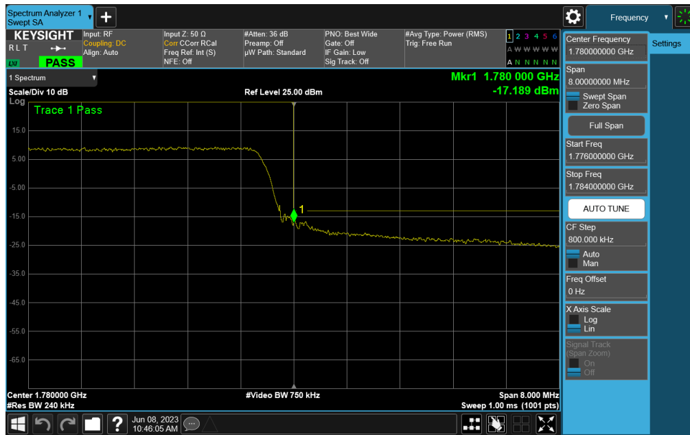
Plot 7-70. Upper Band Edge Plot (LTE Band 66 - 10MHz QPSK – Full RB)
