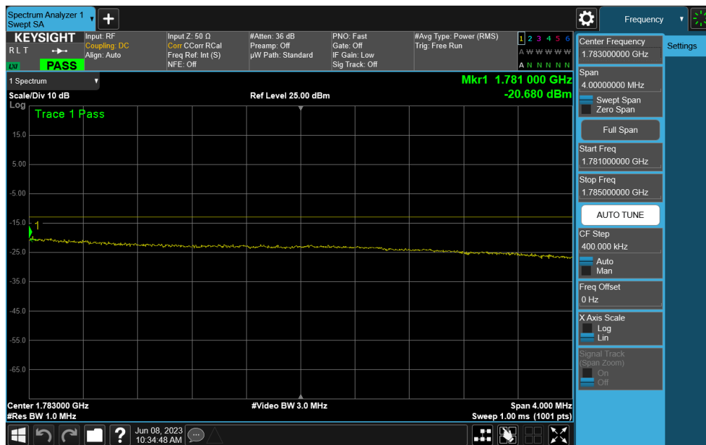
Plot 7-75. Upper Extended Band Edge Plot (LTE Band 66 - 15MHz QPSK – Full RB)
