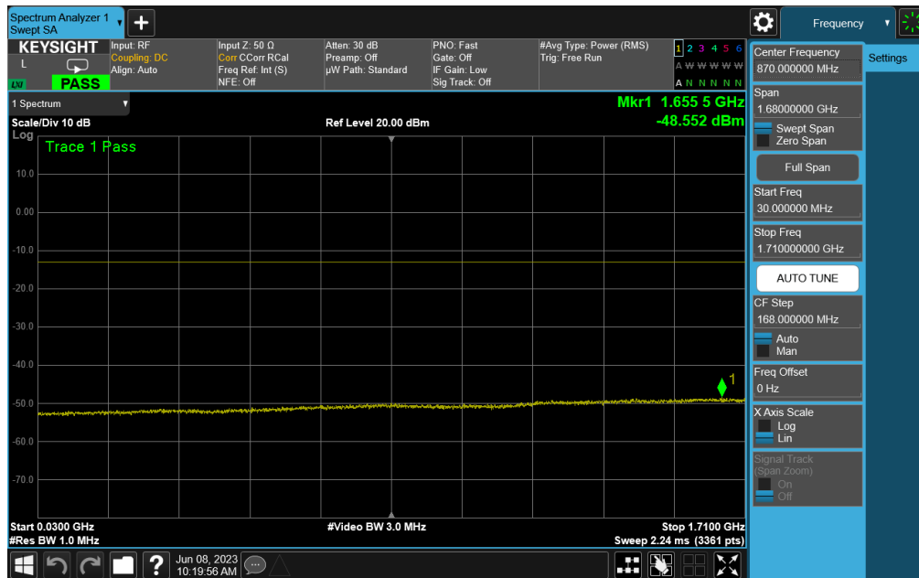
Plot 7-32. Conducted Spurious Plot (LTE Band 66/4 - 20MHz QPSK - RB Size 1, RB Offset 0 - High Channel)
