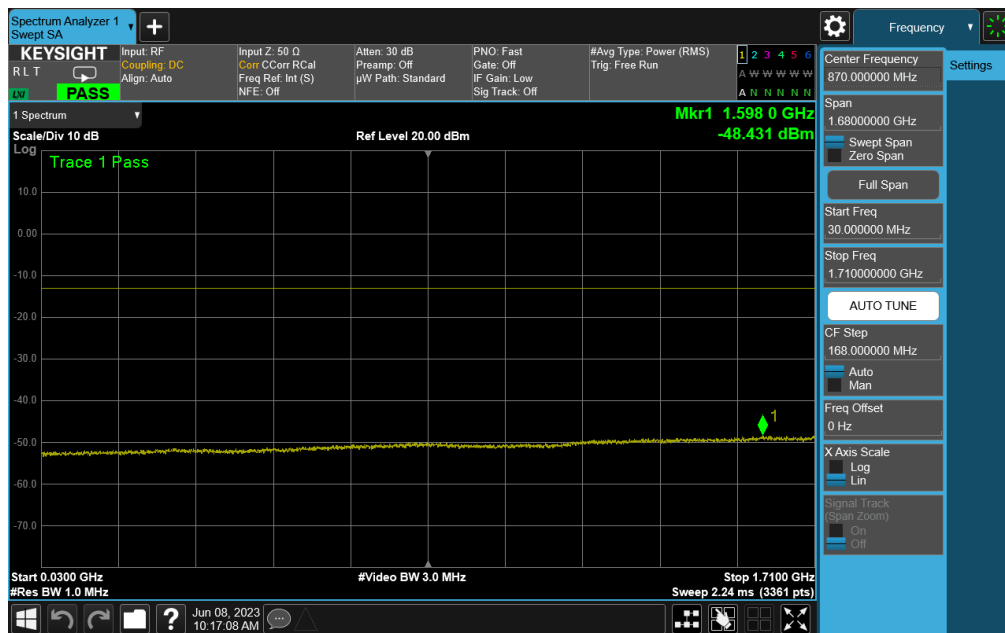
Plot 7-29. Conducted Spurious Plot (LTE Band 66/4 - 20MHz QPSK - RB Size 1, RB Offset 0 - Mid Channel)
