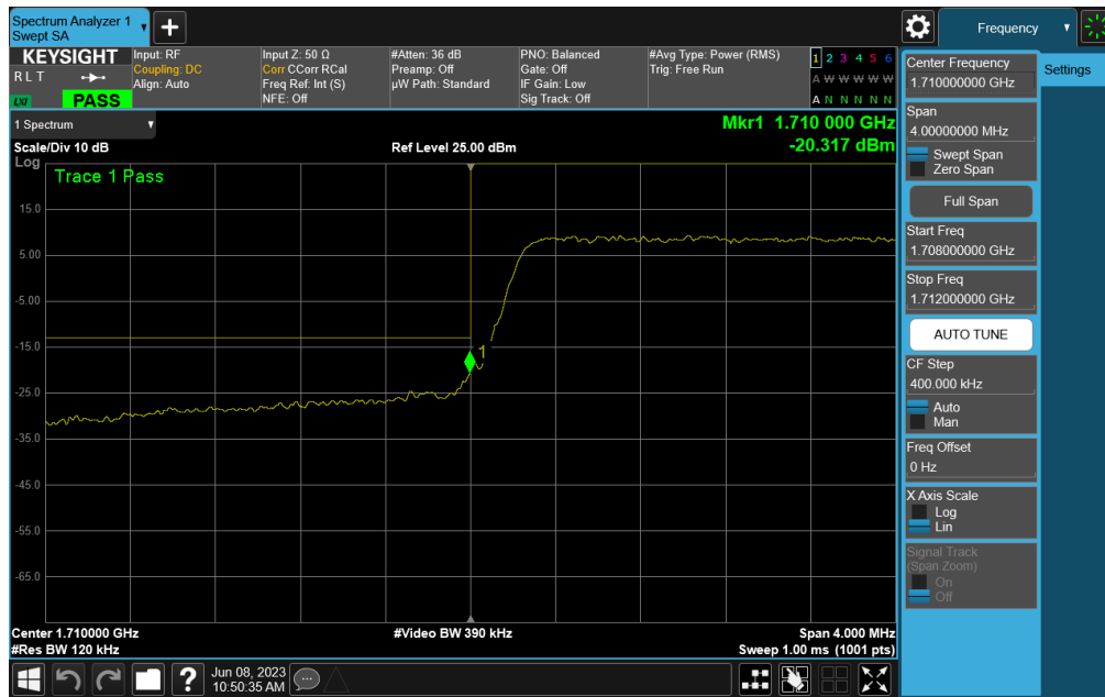
Plot 7-64. Lower Band Edge Plot (LTE Band 66 - 5MHz QPSK – Full RB)
