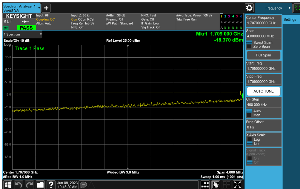
Plot 7-69. Lower Extended Band Edge Plot (LTE Band 66 - 10MHz QPSK – Full RB)
