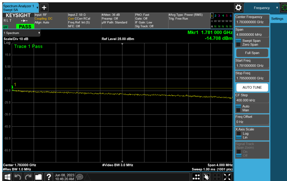
Plot 7-71. Upper Extended Band Edge Plot (LTE Band 66 - 10MHz QPSK – Full RB)
