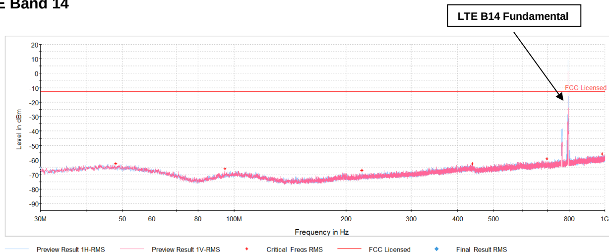
Plot 7-48. Antenna BCM Radiated Spurious Plot below 1GHz (LTE Band 14)
