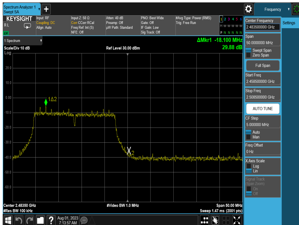
Plot 7-42. Band Edge Plot (802.11n (2.4GHz) – Ch. 13) – MCS0
