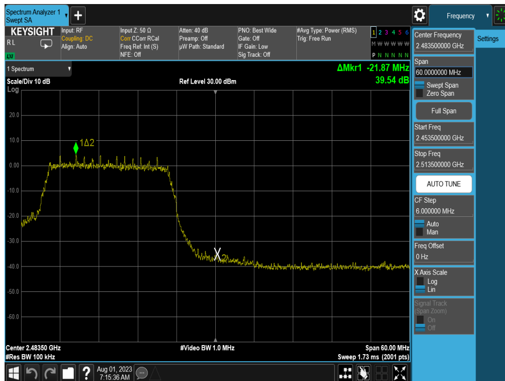
Plot 7-41. Band Edge Plot (802.11n (2.4GHz) – Ch. 12) – MCS0
