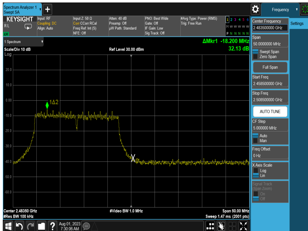
Plot 7-48. Band Edge Plot (802.11n (2.4GHz) – Ch. 13) – MCS7
