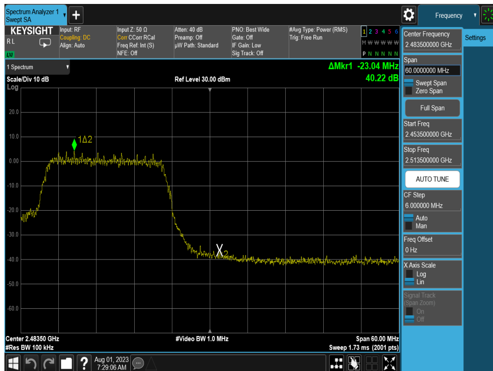
Plot 7-47. Band Edge Plot (802.11n (2.4GHz) – Ch. 12) – MCS7
