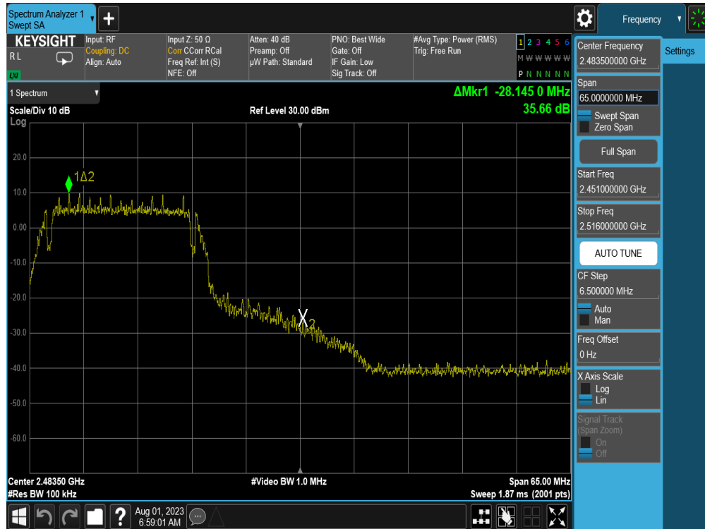
Plot 7-33. Band Edge Plot (802.11g – Ch. 11) – 6Mbps
