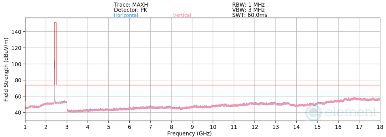
Plot 7-55. Radiated Spurious Emissions above 1GHz (802.11b – Ch. 1)
