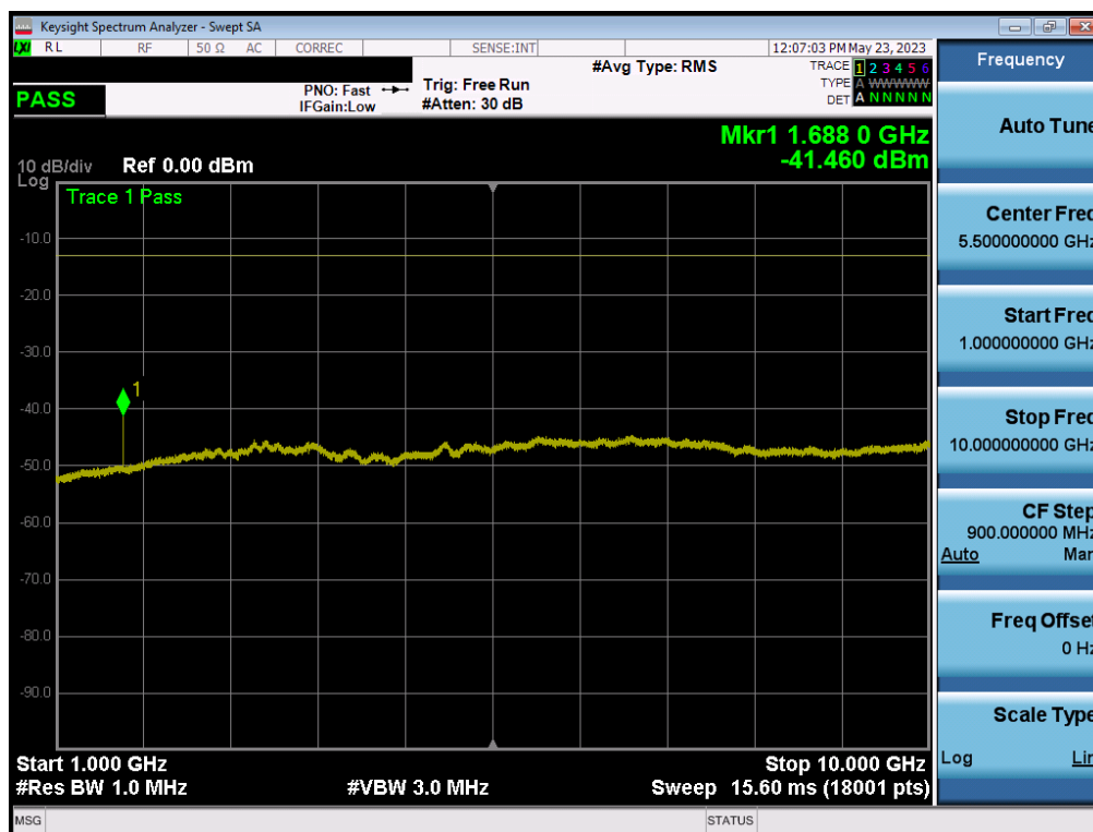
Plot 7-18. Conducted Spurious Plot (LTE Band 26/5 - 10MHz QPSK - RB Size 1, RB Offset 0 - High Channel)
