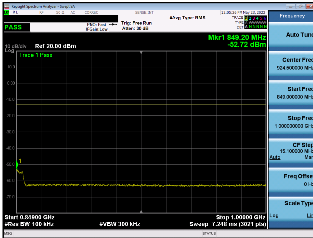
Plot 7-14. Conducted Spurious Plot (LTE Band 26/5 - 10MHz QPSK - RB Size 1, RB Offset 0 - Mid Channel)
