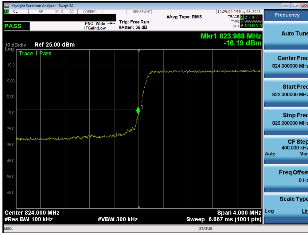
Plot 7-38. Lower BE Plot (LTE Band 5 - 3MHz QPSK – Full RB Configuration)
