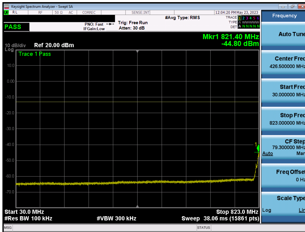
Plot 7-10. Conducted Spurious Plot (LTE Band 26/5 - 10MHz QPSK - RB Size 1, RB Offset 0 - Low Channel)
