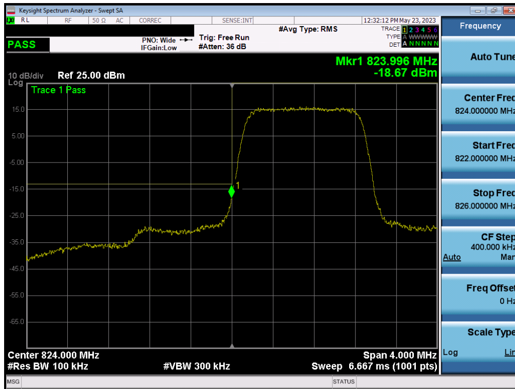
Plot 7-36. Lower BE Plot (LTE Band 5 – 1.4MHz QPSK – Full RB Configuration)
