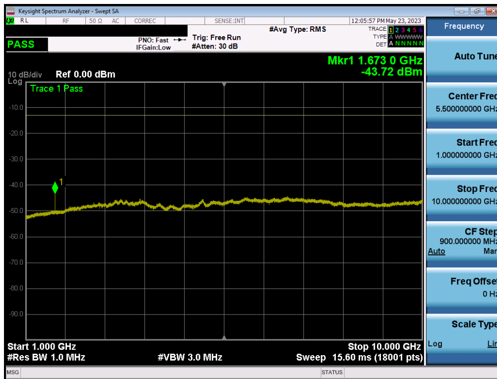
Plot 7-15. Conducted Spurious Plot (LTE Band 26/5 - 10MHz QPSK - RB Size 1, RB Offset 0 - Mid Channel)
