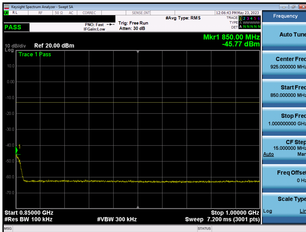
Plot 7-17. Conducted Spurious Plot (LTE Band 26/5 - 10MHz QPSK - RB Size 1, RB Offset 0 - High Channel)
