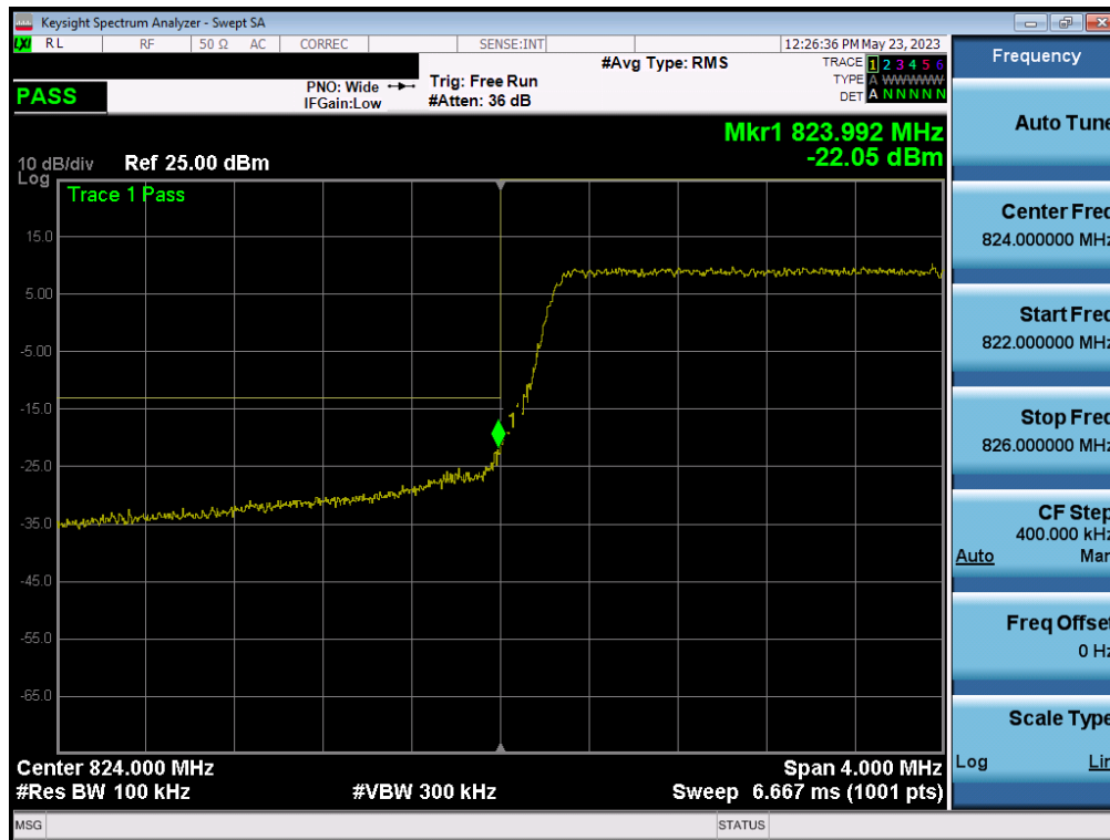
Plot 7-40. Lower BE Plot (LTE Band 5 - 5MHz QPSK – Full RB Configuration)
