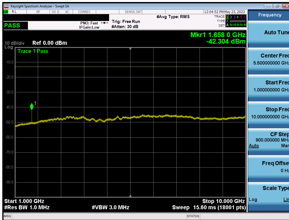
Plot 7-12. Conducted Spurious Plot (LTE Band 26/5 - 10MHz QPSK - RB Size 1, RB Offset 0 - Low Channel)
