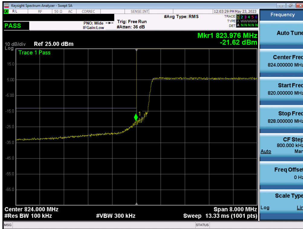
Plot 7-42. Lower BE Plot (LTE Band 5 - 10MHz QPSK – Full RB Configuration)
