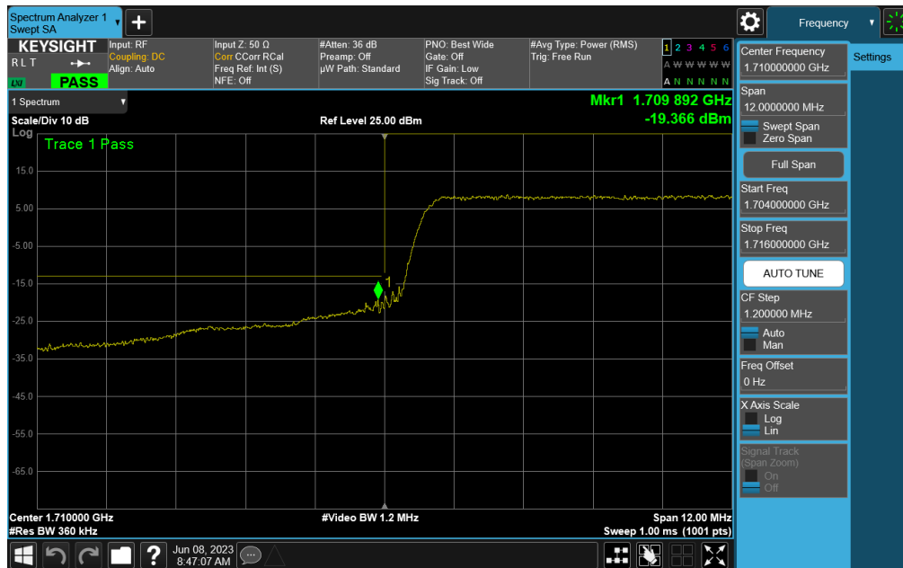
Plot 7-72. Lower Band Edge Plot (LTE Band 66 - 15MHz QPSK – Full RB)
