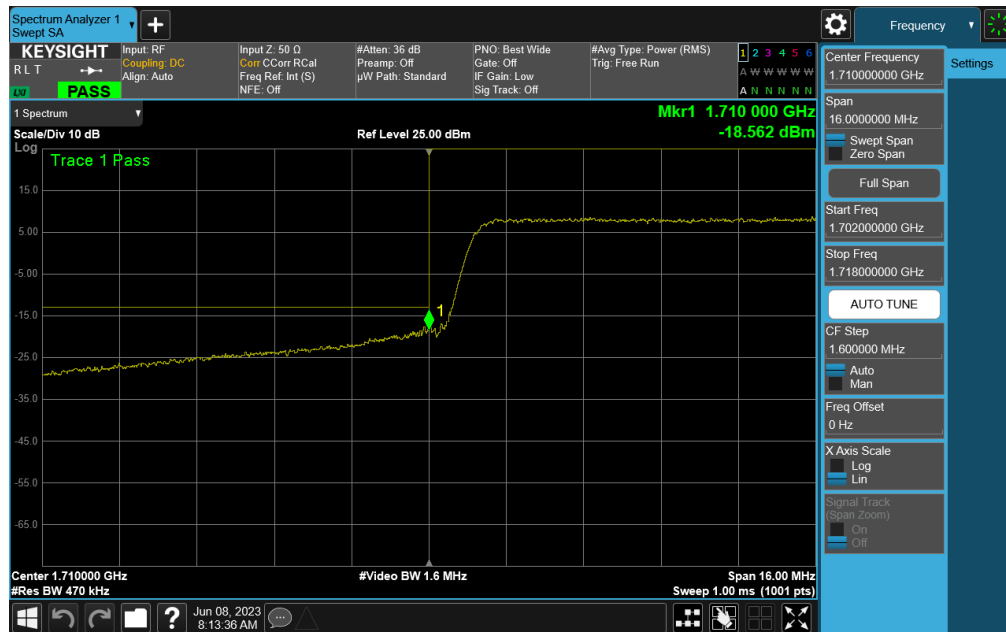
Plot 7-76. Lower Band Edge Plot (LTE Band 66 - 20MHz QPSK – Full RB)
