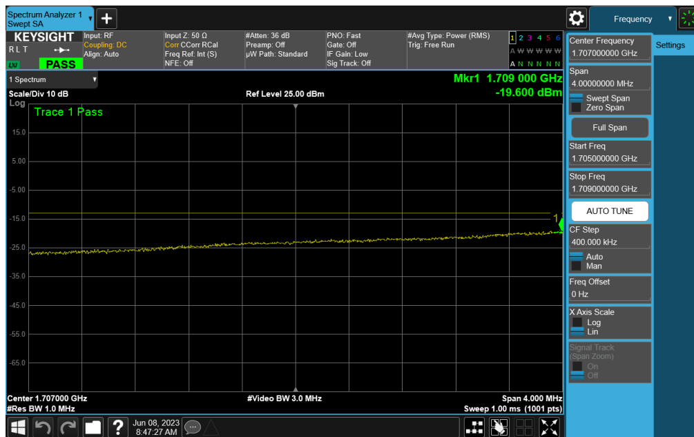
Plot 7-73. Lower Extended Band Edge Plot (LTE Band 66 - 15MHz QPSK – Full RB)
