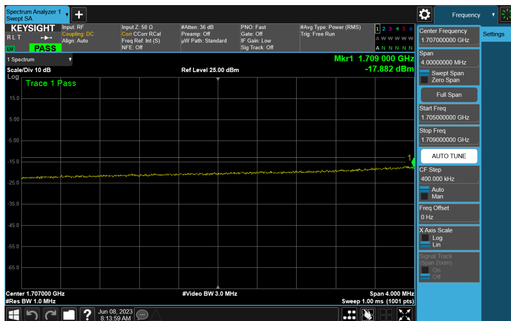
Plot 7-77. Lower Extended Band Edge Plot (LTE Band 66 - 20MHz QPSK – Full RB)
