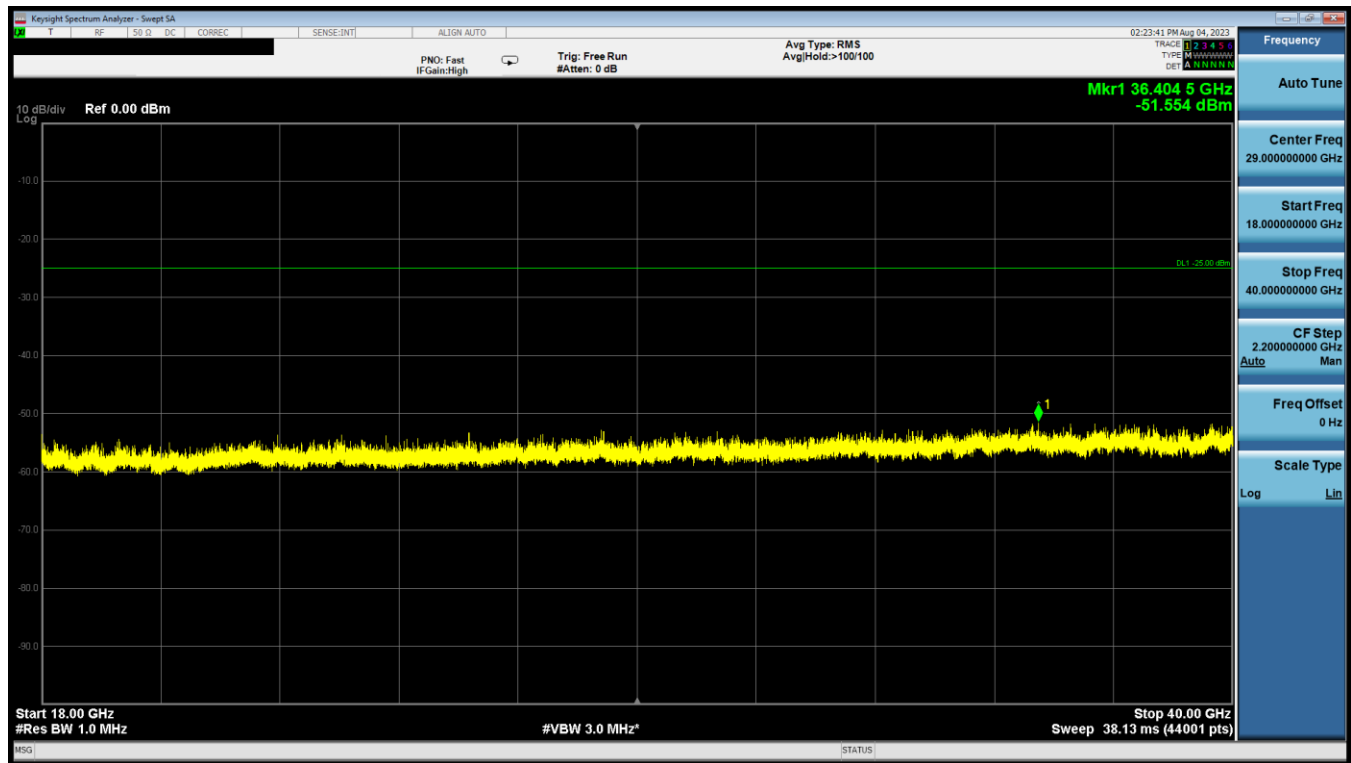
Plot 7-67. Antenna FCM Radiated Spurious Plot above 18GHz (Simultaneous Transmission, Pol. H)
