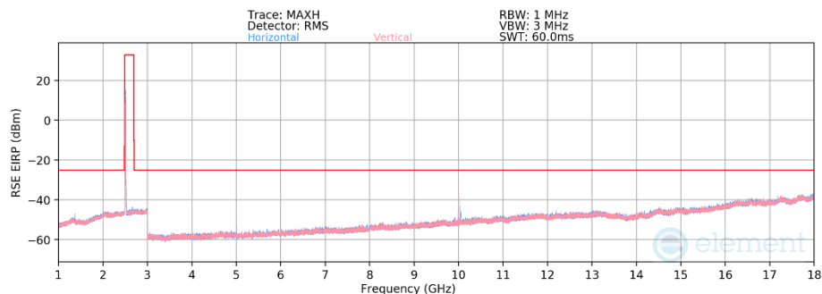
Plot 7-62. Antenna FCM Radiated Spurious Plot above 1GHz (LTE Band 41)
