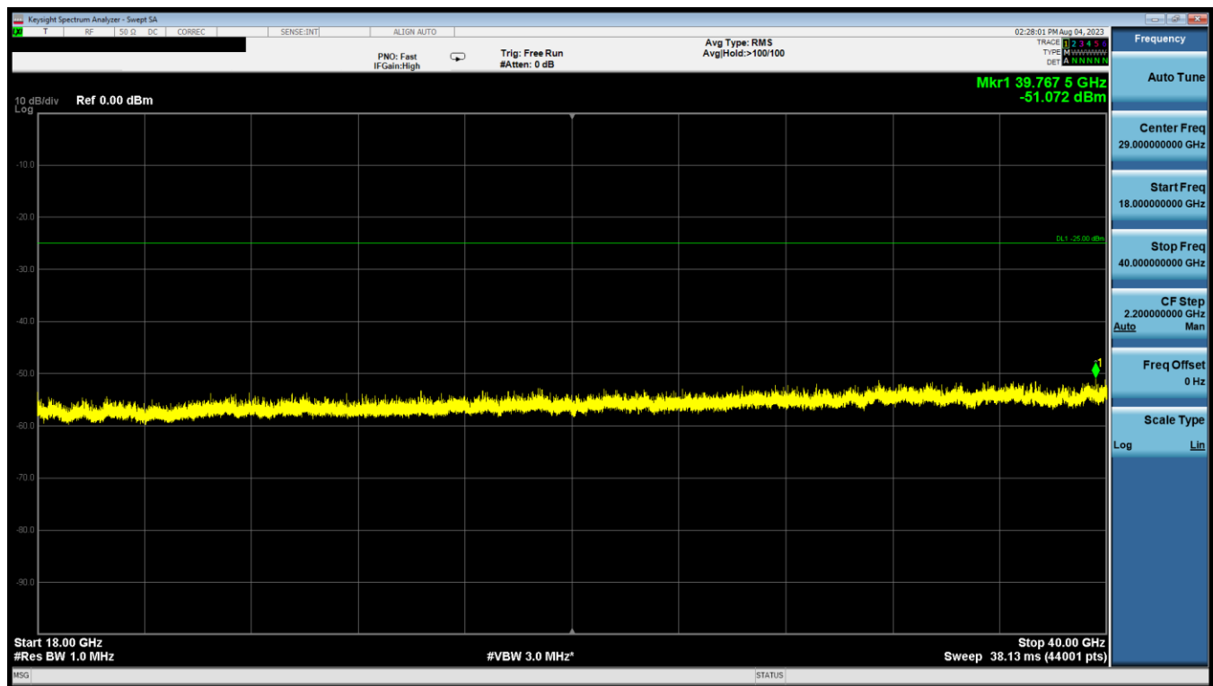
Plot 7-68. Antenna FCM Radiated Spurious Plot above 18GHz (Simultaneous Transmission, Pol. V)
