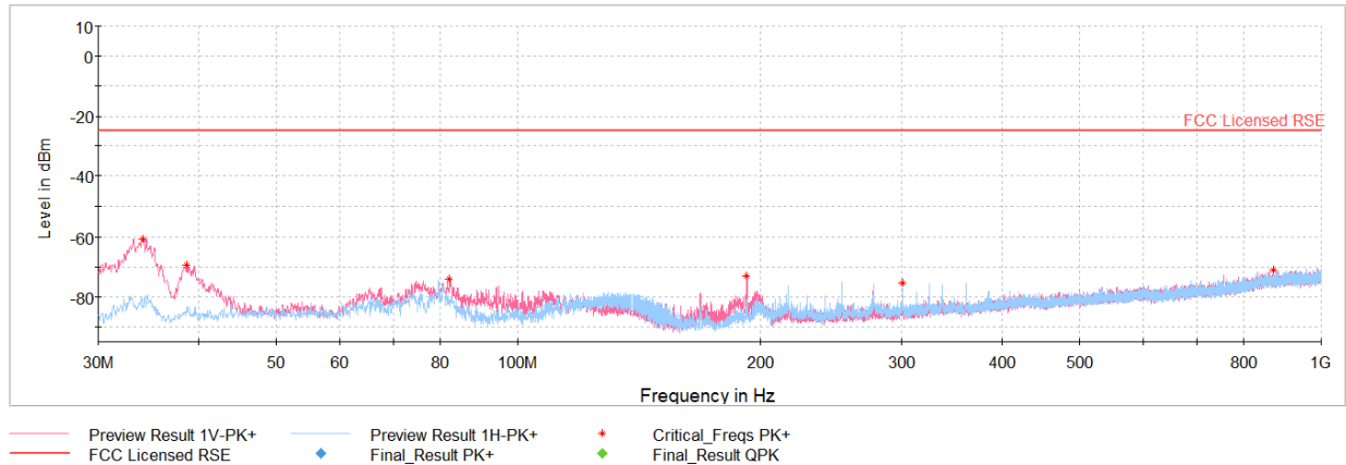
Plot 7-65. Antenna FCM Radiated Spurious Emissions -Simultaneous Transmission 30MHz – 1GHz
