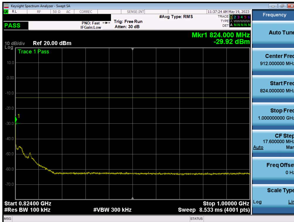
Plot 7-17. Conducted Spurious Plot (LTE Band 26 - 10MHz QPSK - RB Size 1, RB Offset 0)
