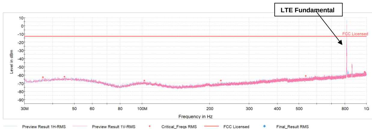
Plot 7-46. Antenna BCM Radiated Spurious Plot below 1GHz (LTE Band 26)
