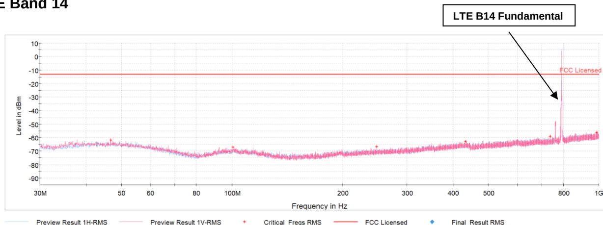
Plot 7-48. Antenna BCM Radiated Spurious Plot below 1GHz (LTE Band 14)
