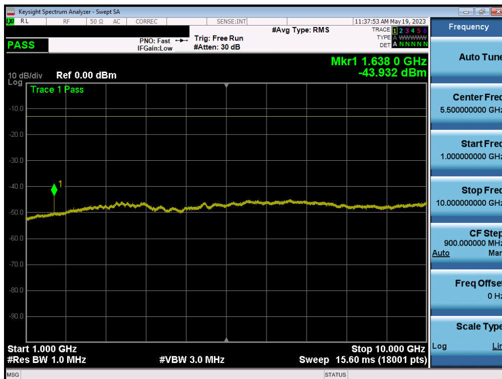
Plot 7-18. Conducted Spurious Plot (LTE Band 26 - 10MHz QPSK - RB Size 1, RB Offset 0)
