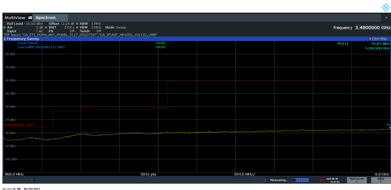
Plot 7-26. FCC Radiated Spurious Emission 960-6000MHz (Ch.9, Config 409, Payload 4093 Ant. Pol. V)
