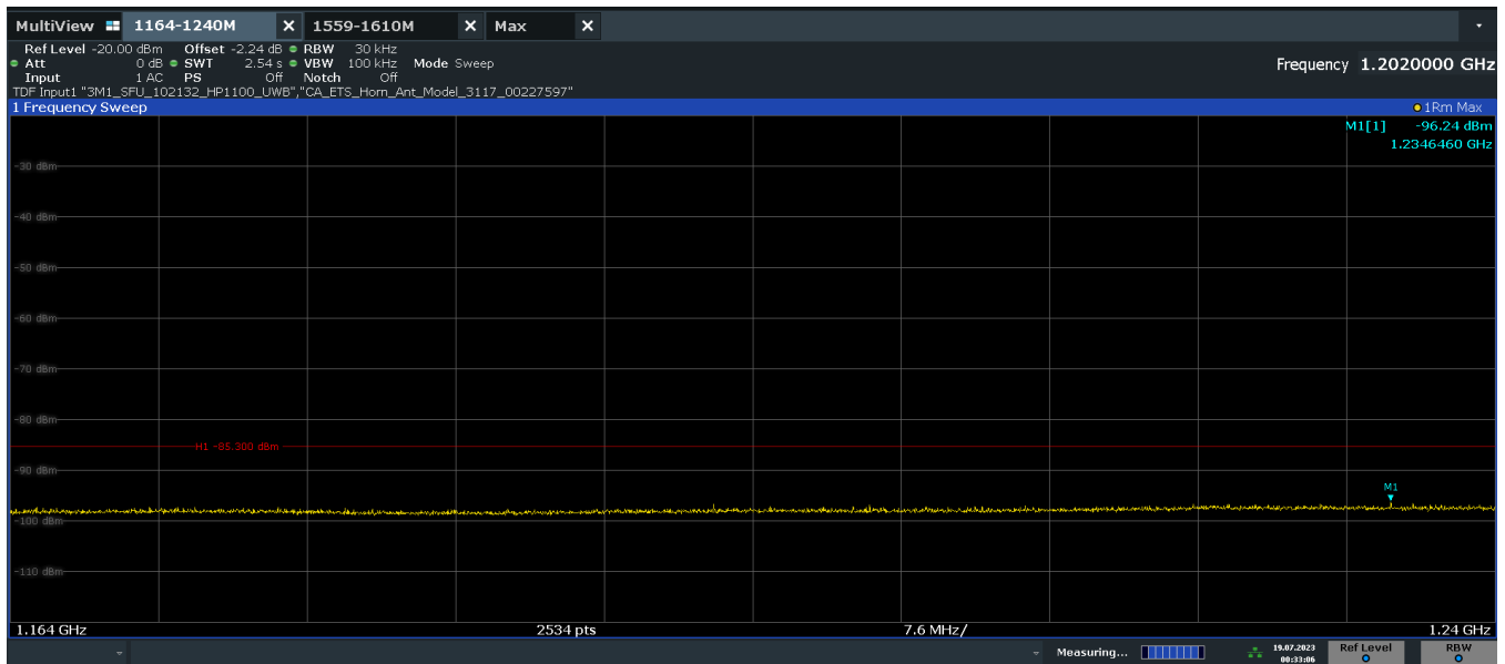
Plot 7-30. Radiated Spurious Emission 1164-1240MHz (Ch. 9, Config 409, Payload 4093 Ant. Pol. V)
