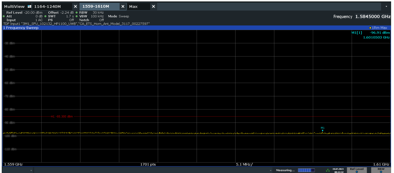
Plot 7-31. Radiated Spurious Emission 1559-1610MHz (Ch. 9, Config 409, Payload 4093 Ant. Pol. H)
