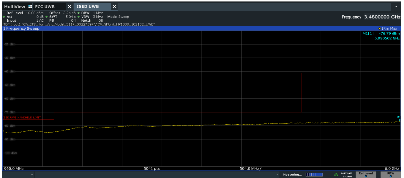
Plot 7-27. ISED Radiated Spurious Emission 960-6000MHz (Ch. 9, Config 409, Payload 4093 Ant. Pol. H)
