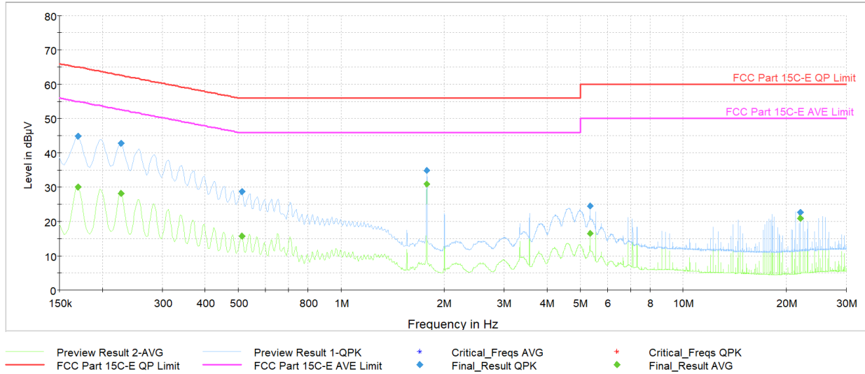
Plot 7-44. AC Line Conducted Plot (Ch. 9, Config 409, Payload 4093 N, with AC/DC Adapter + Magnetic Charger)
