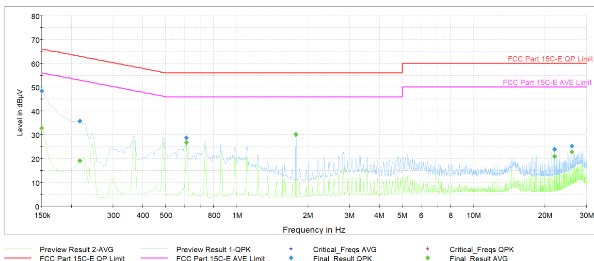
Plot 7-41. AC Line Conducted (Ch. 5, Config 409, Payload 4093 L1, with PC via USB-C cable with magnetic charger)
