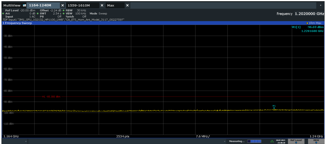
Plot 7-19. Radiated Spurious Emission 1164-1240MHz (Ch. 5, Config 409, Payload 4093 Ant. Pol. H)
