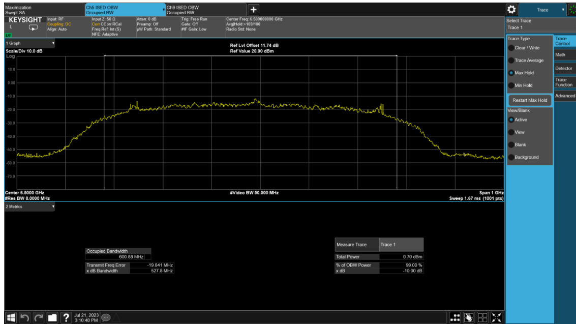
Plot 7-3. ISD 10dBc Occupied Bandwidth & 99% (Ch. 5, Config 409/Payload 4093)
