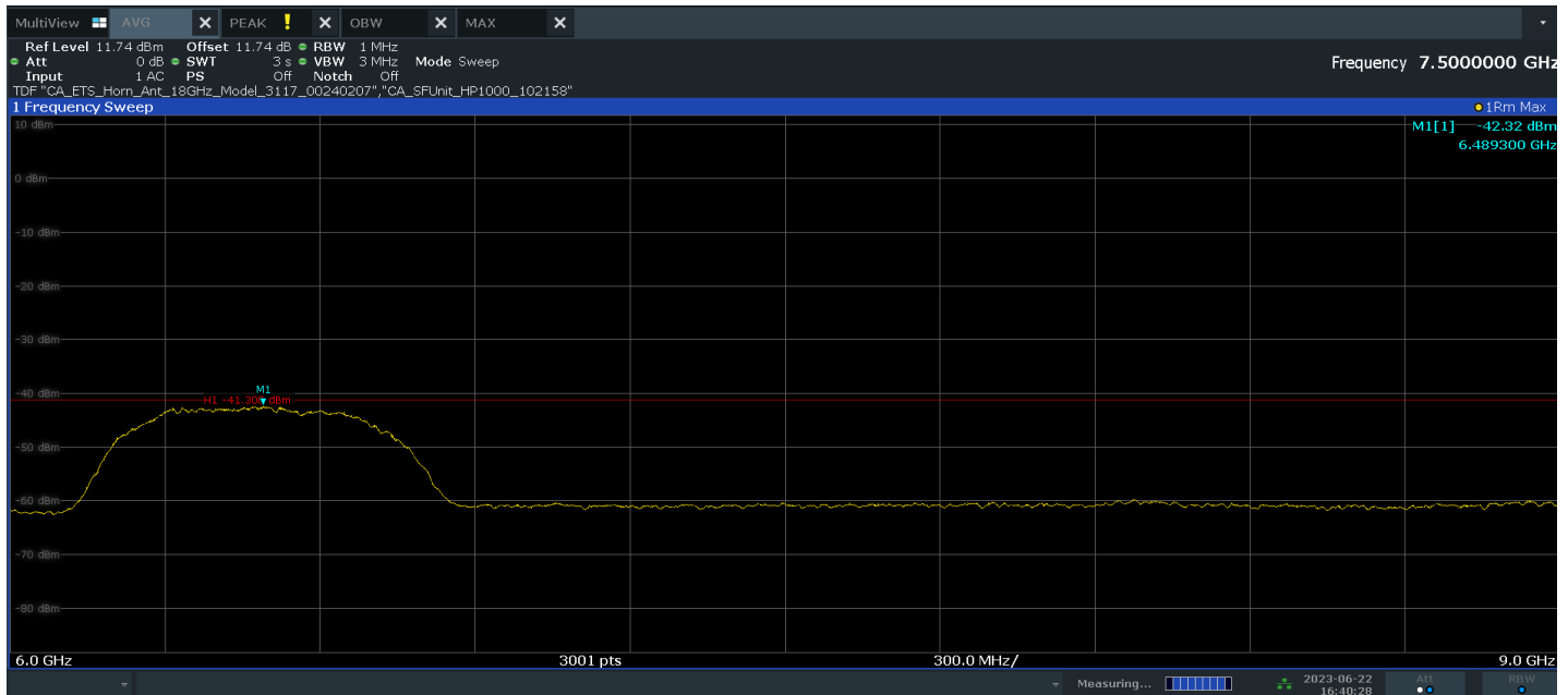
Plot 7-7. Average Radiated Power (Ch. 5, Config 409/Payload 4093)
