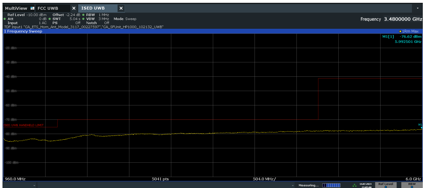
Plot 7-18. ISED Radiated Spurious Emission 960-6000MHz (Ch. 5, Config 409, Payload 4093 Ant. Pol. V)
