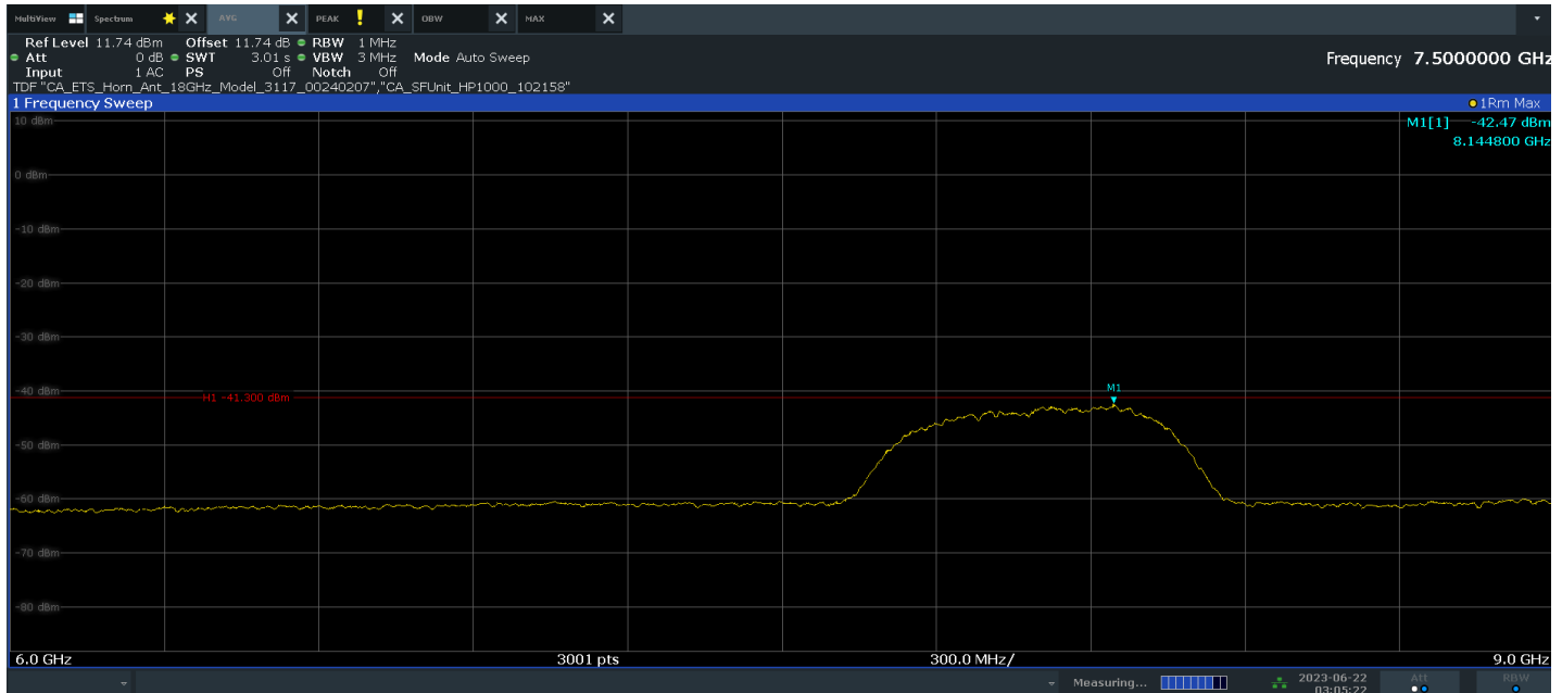
Plot 7-8. Average Radiated Power (Ch. 9, Config 409/Payload 4093)
