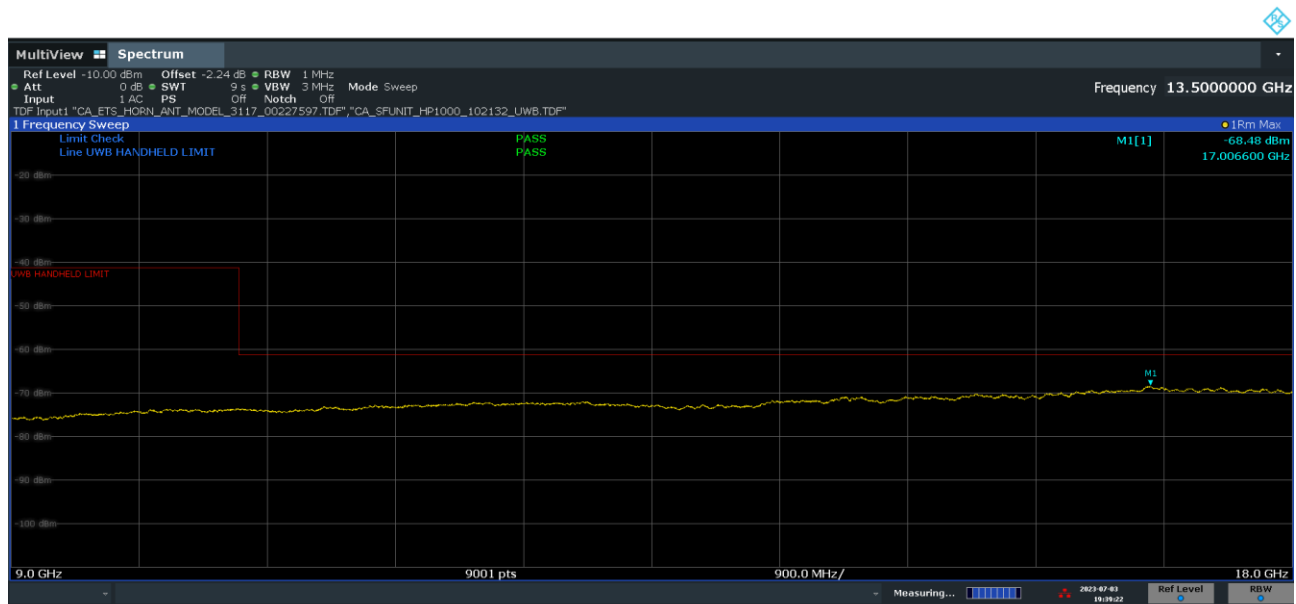
Plot 7-24. Radiated Spurious Emission 9-18GHz (Ch. 5, Config 409, Payload 4093 Ant. Pol. V)
