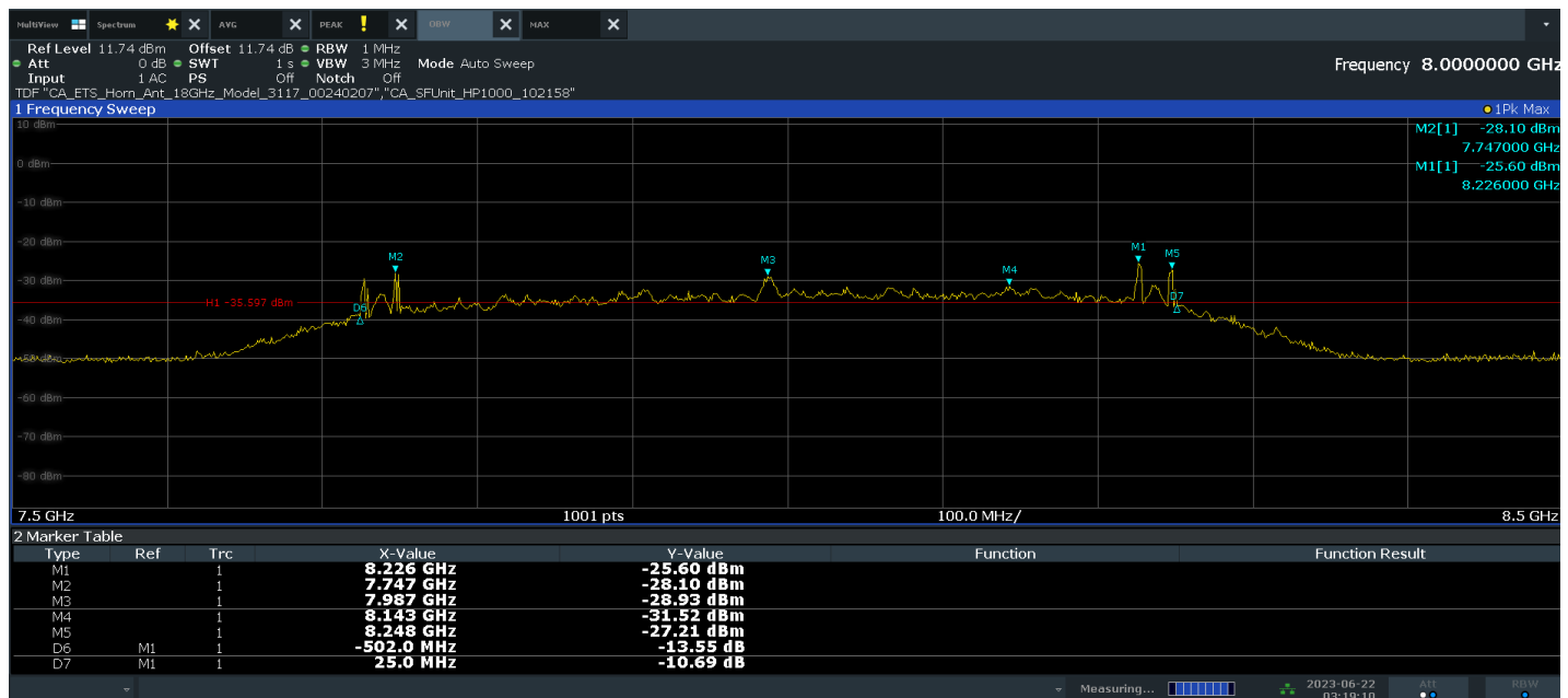
Plot 7-2. 10dBc Bandwidth (Ch. 9, Config 409/Payload 4093)
