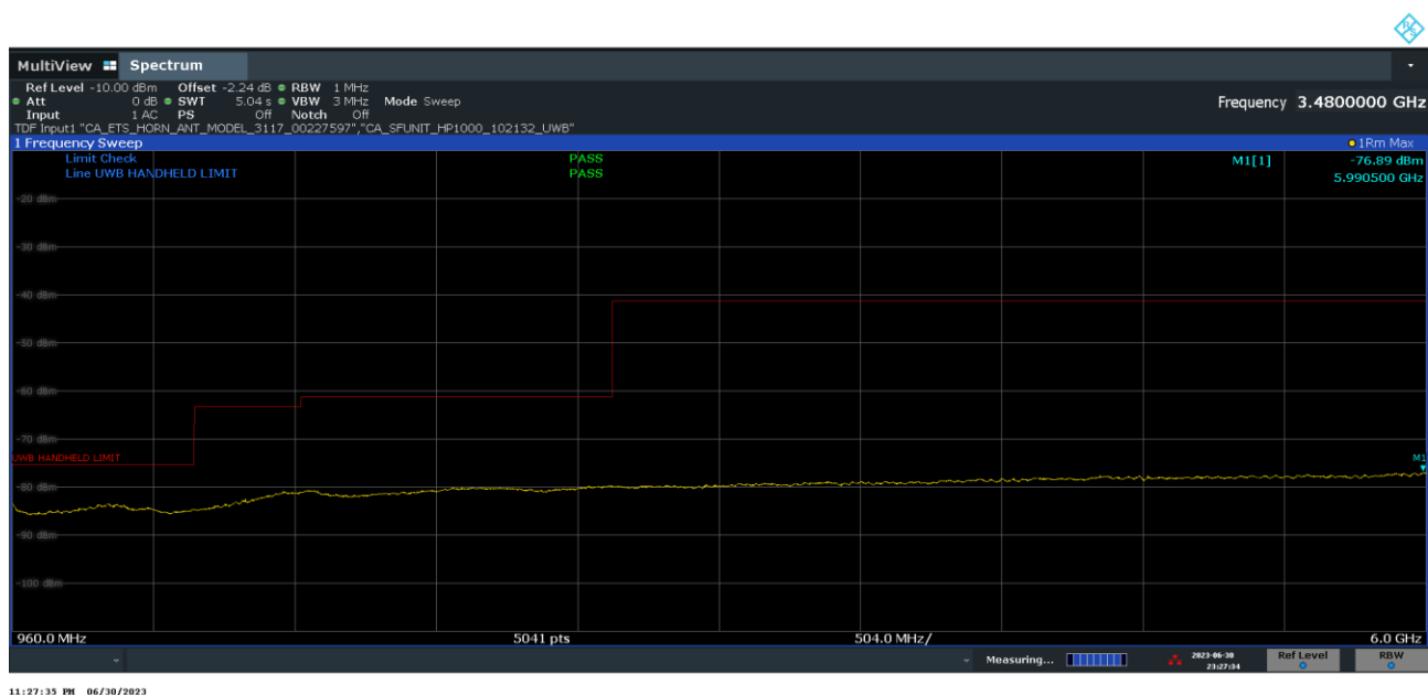
Plot 7-25. FCC Radiated Spurious Emission 960-6000MHz (Ch. 9, Config 409, Payload 4093 Ant. Pol. H)
