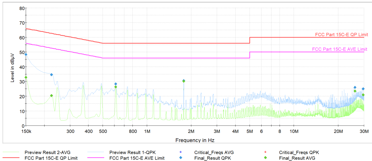
Plot 7-42. AC Line Conducted (Ch. 5, Config 409, Payload 4093 N, with PC via USB-C cable with magnetic charger)
