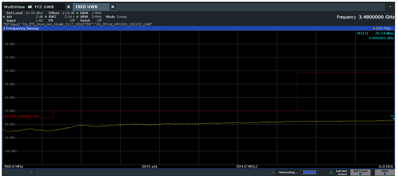
Plot 7-28. ISED Radiated Spurious Emission 960-6000MHz (Ch.9, Config 409, Payload 4093 Ant. Pol. V)
