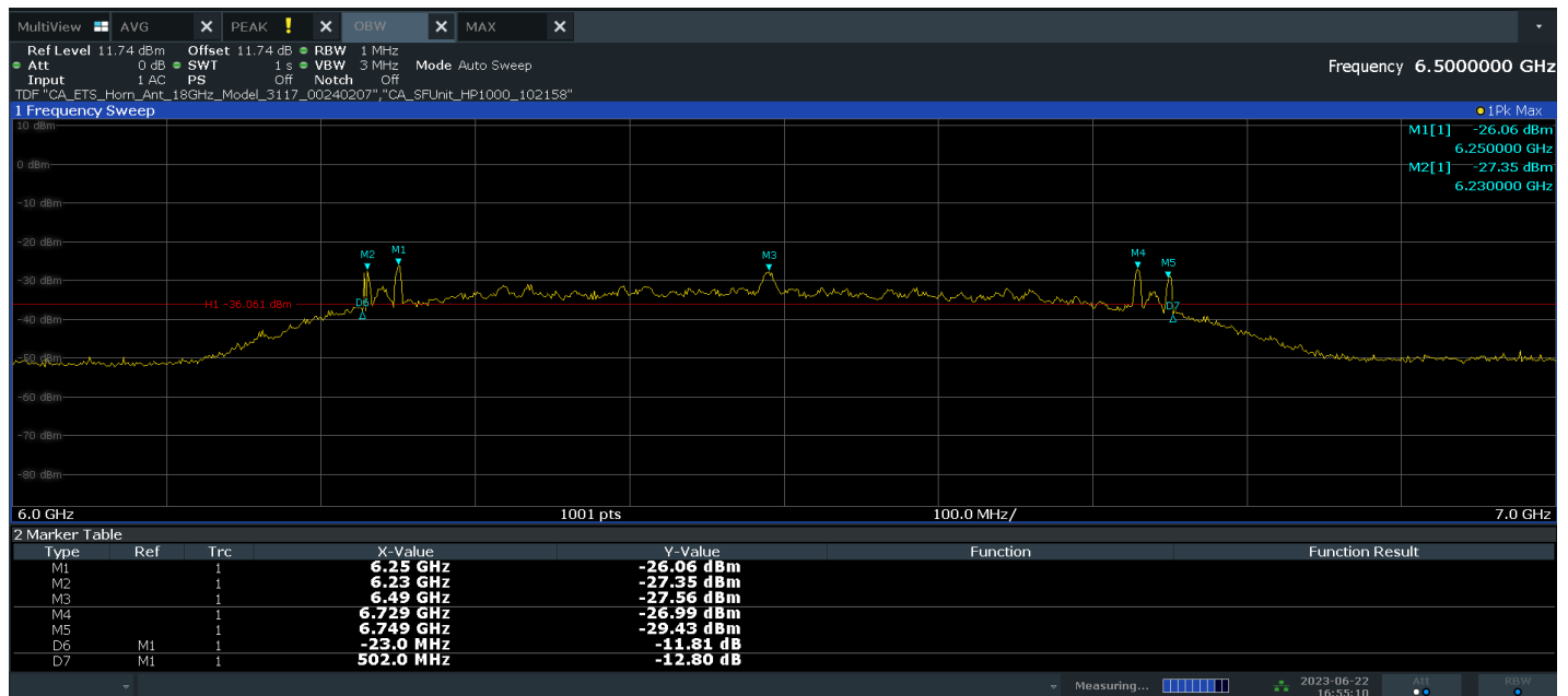
Plot 7-1. 10dBc Bandwidth (Ch. 5, Config 409/Payload 4093)
