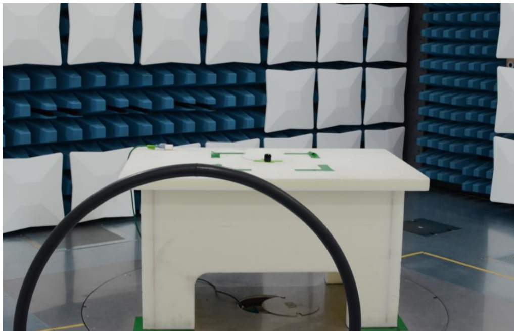
Figure 22: 9kHz-30MHz Test Setup (Front View)
