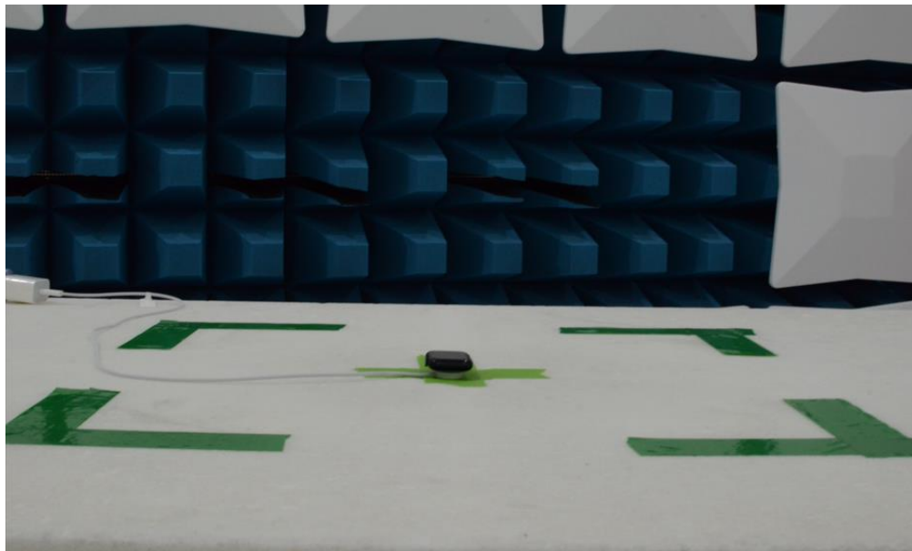
Figure 8: 30MHz-1GHz Test Setup (Front View)
