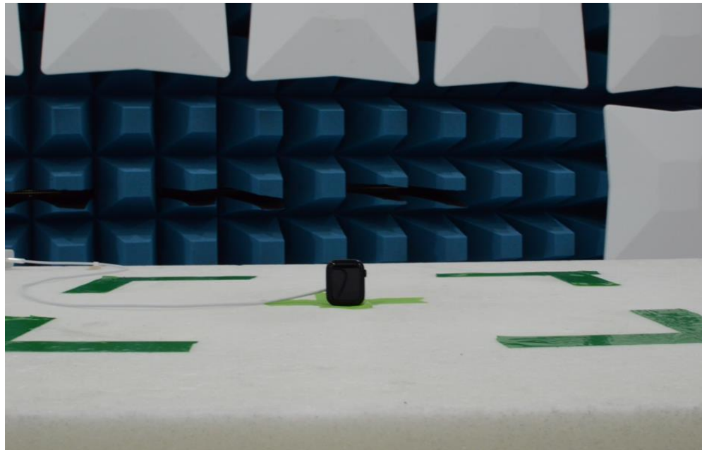
Figure 12: 30MHz-1GHz Test Setup (Front View)
