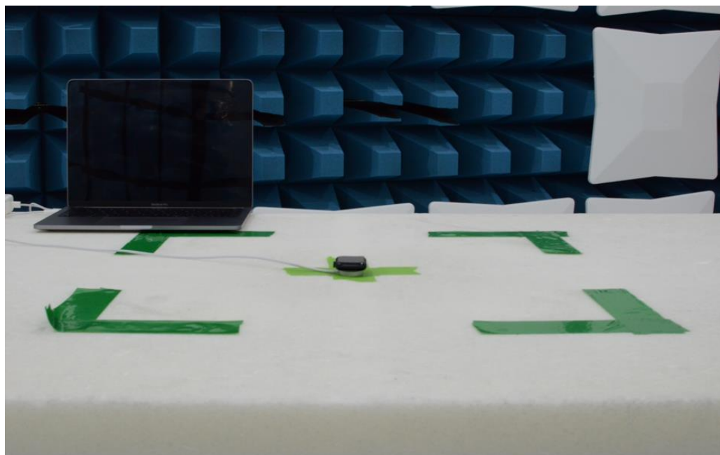
Figure 14: 30MHz-1GHz Test Setup (Front View)
