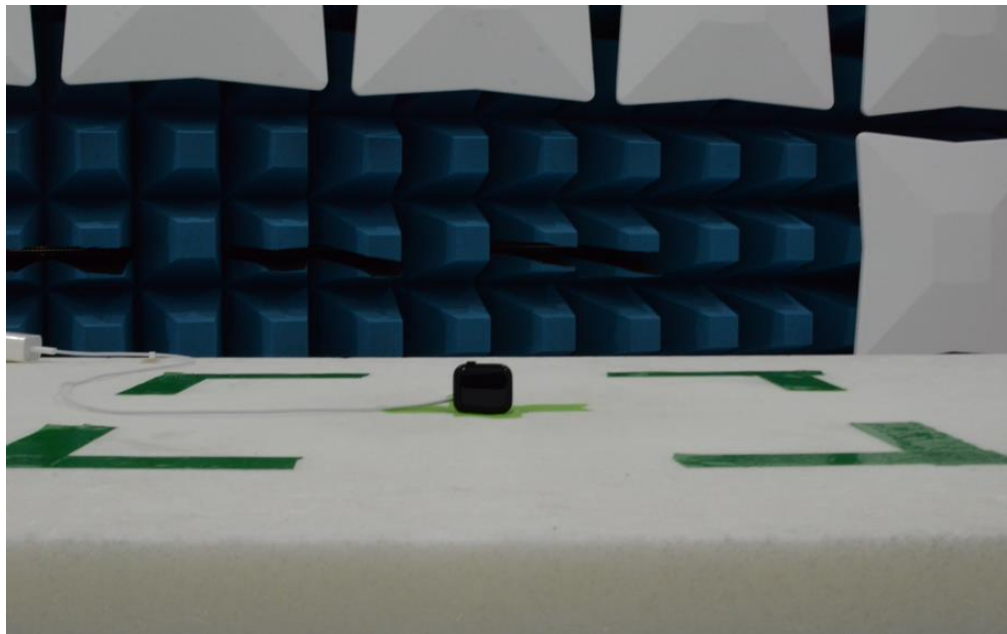
Figure 10: 30MHz-1GHz Test Setup (Front View)
