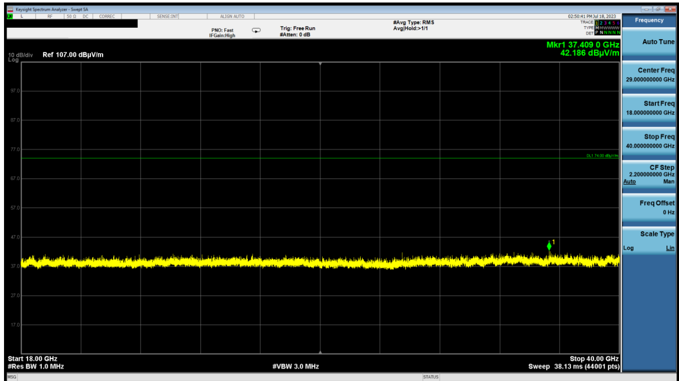
Plot 7-23. Radiated Spurious Emissions Above 18GHz (OQPSK – 5786.25MHz Pol V)
