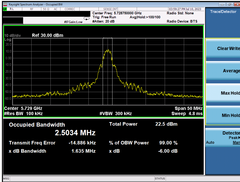
Plot 7-1. 6dB BW & 99% OBW (OQPSK, 5728.75MHz, 250kbps)
