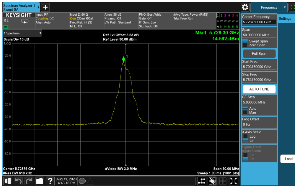
Plot 7-13. PSD (OQPSK, 5728.75MHz, 500kbps)
