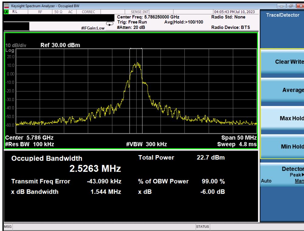
Plot 7-8. 6dB BW & 99% OBW (QPSK, 5786.25MHz, 1000kbps)
