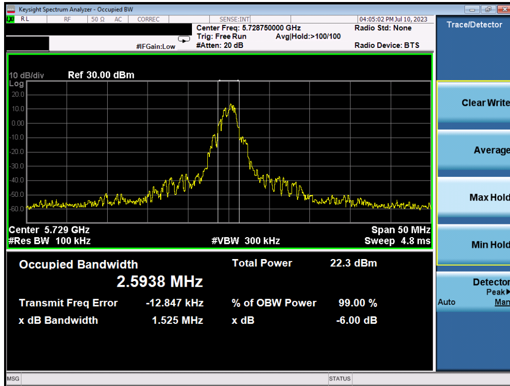
Plot 7-7. 6dB BW & 99% OBW (QPSK, 5728.75MHz, 1000kbps)
