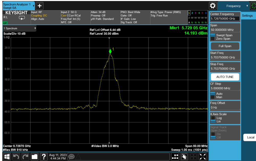
Plot 7-16. PSD (QPSK, 5728.75MHz, 1000kbps)
