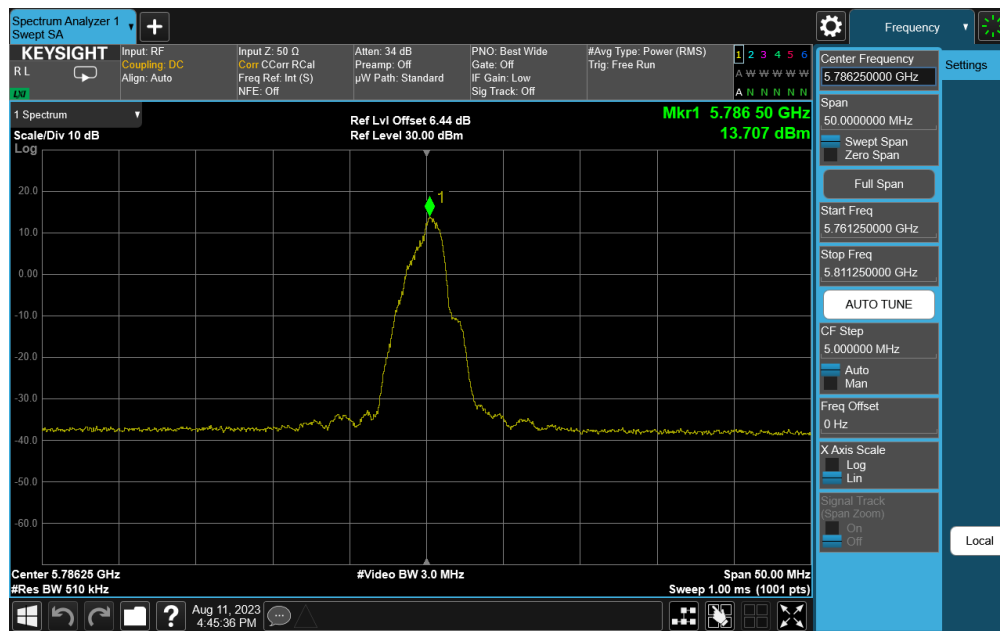
Plot 7-17. PSD (QPSK, 5786.25MHz, 1000kbps)
