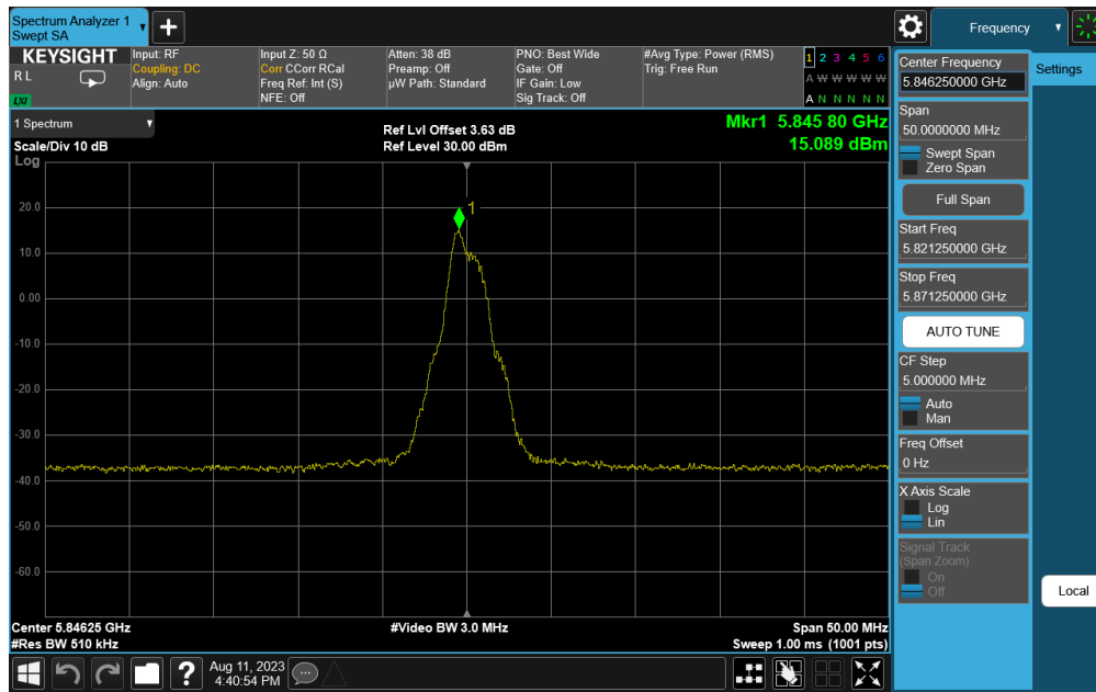
Plot 7-15. PSD (OQPSK, 5846.25MHz, 500kbps)
