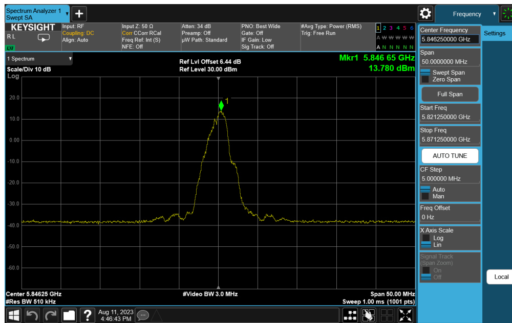
Plot 7-18. PSD (OQPSK, 5846.25MHz, 1000kbps)
