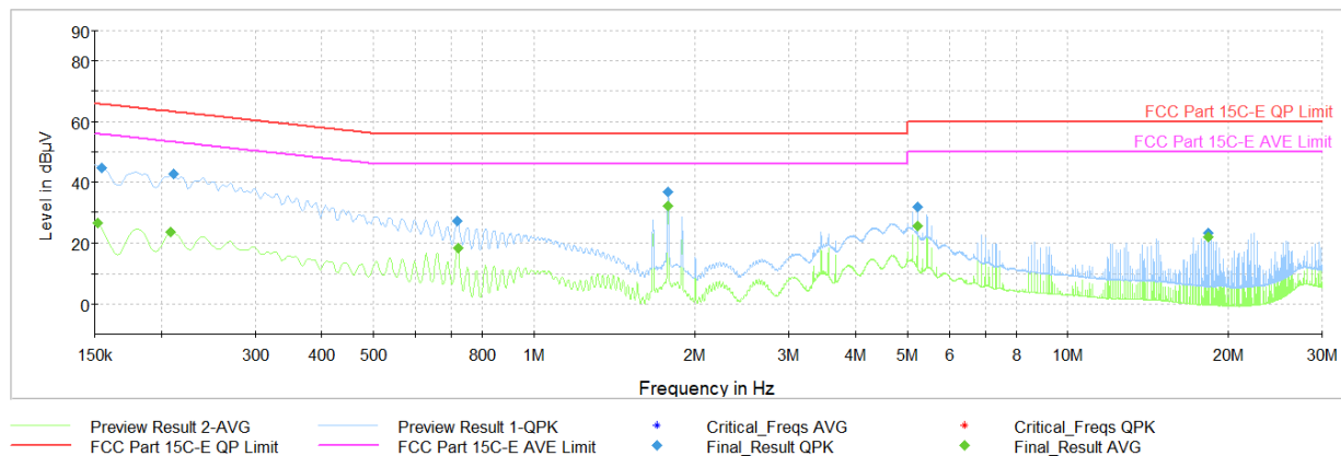
Plot 7-31. AC Line Conducted Plot (OQPSK – Ch. 24) (L1) with AC/DC Adapter & Magnetic charger
