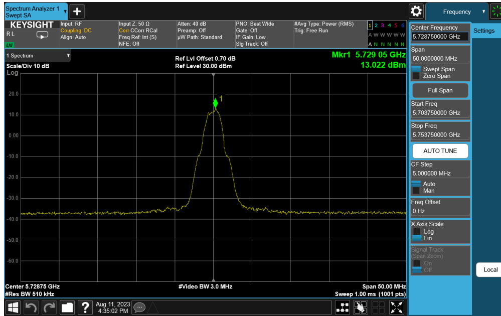
Plot 7-10. PSD (OQPSK, 5728.75MHz, 250kbps)
