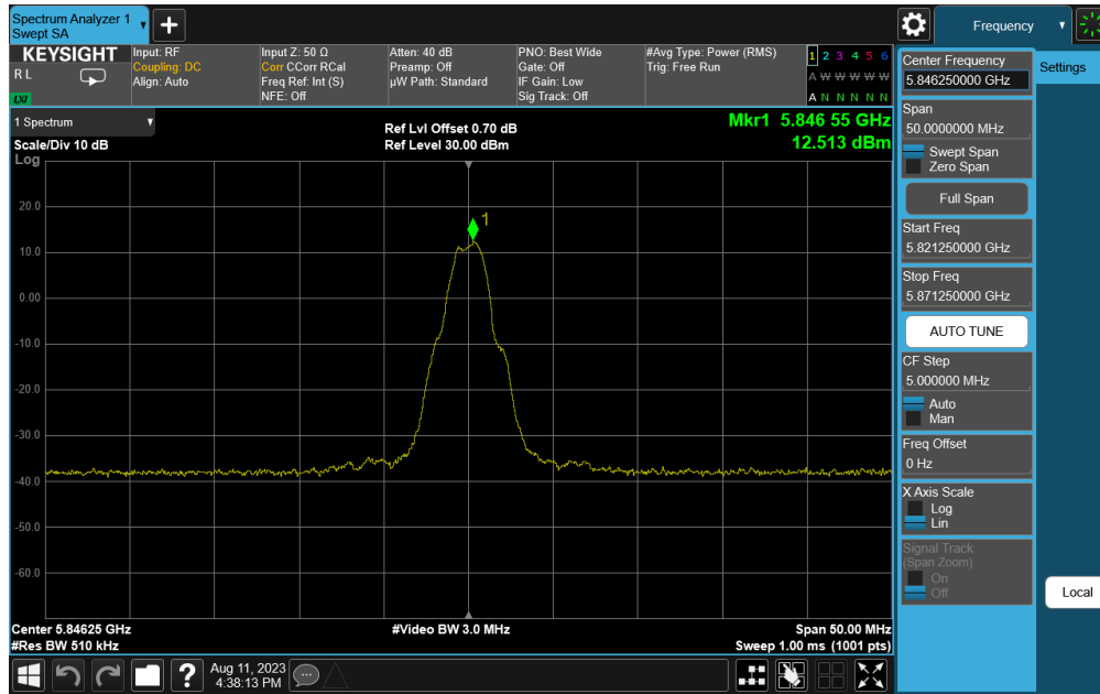
Plot 7-12. PSD (OQPSK, 5846.25MHz, 250kbps)
