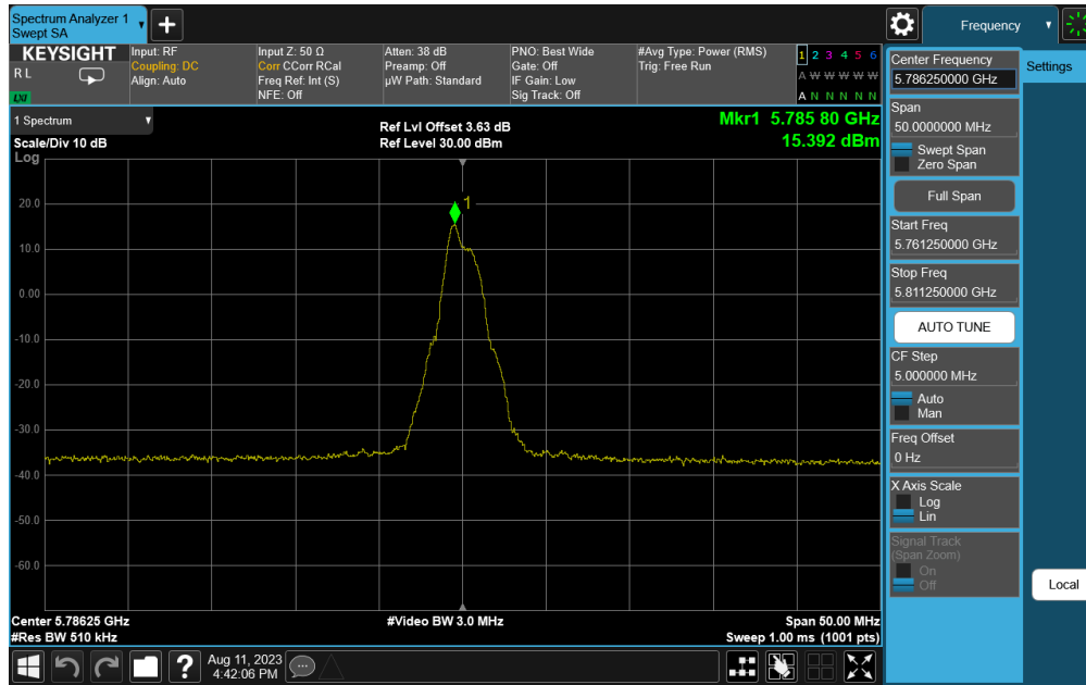
Plot 7-14. PSD (OQPSK, 5786.25MHz, 500kbps)
