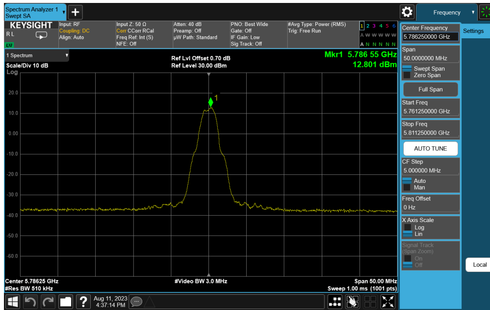
Plot 7-11. PSD (OQPSK, 5786.25MHz, 250kbps)
