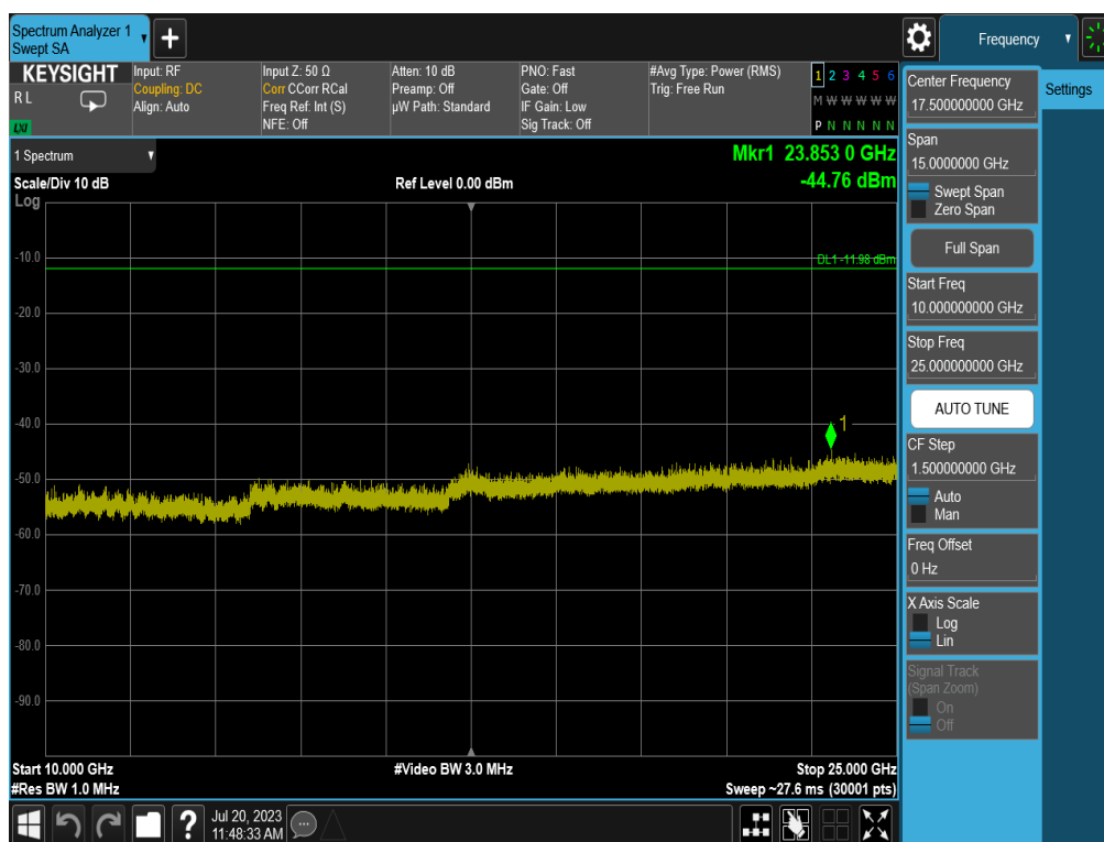
Plot 7-28. Conducted Spurious Plot (Bluetooth (HDR4), 4 Mbps, ePA – Ch. 73)
