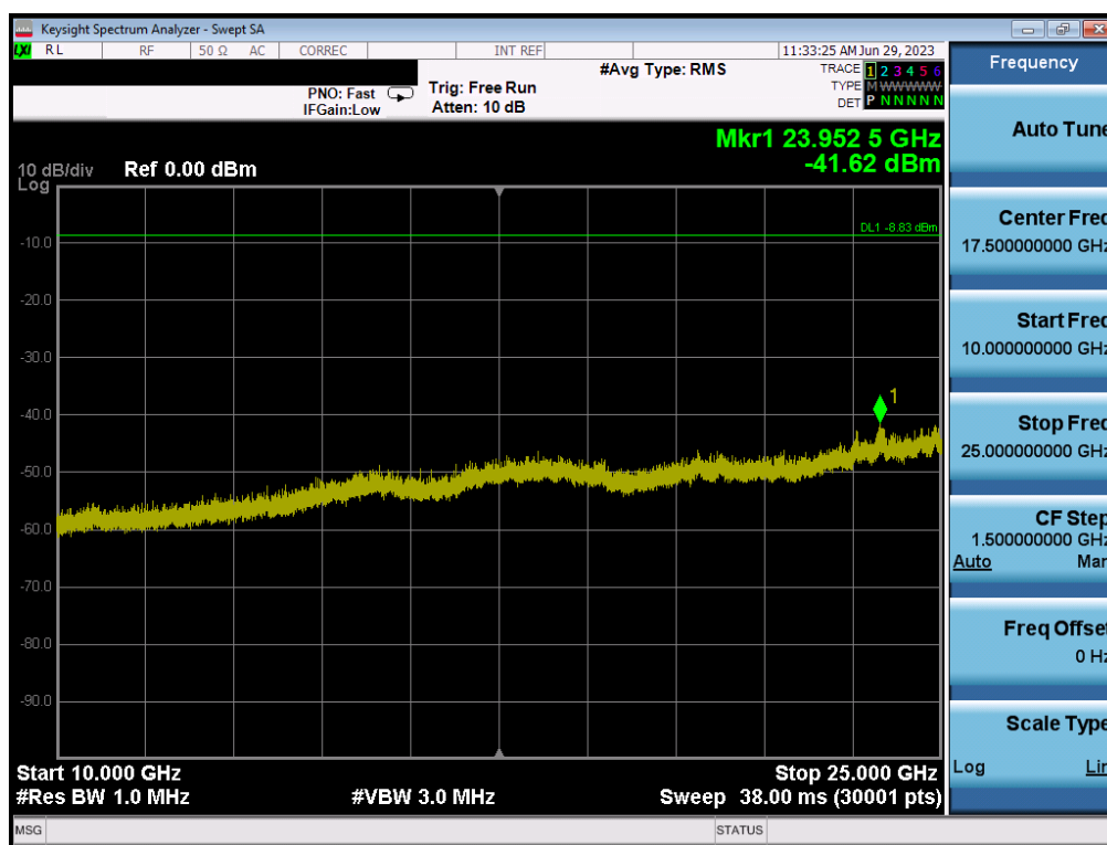
Plot 7-26. Conducted Spurious Plot (Bluetooth (HDR4), 4 Mbps, ePA – Ch. 38)
