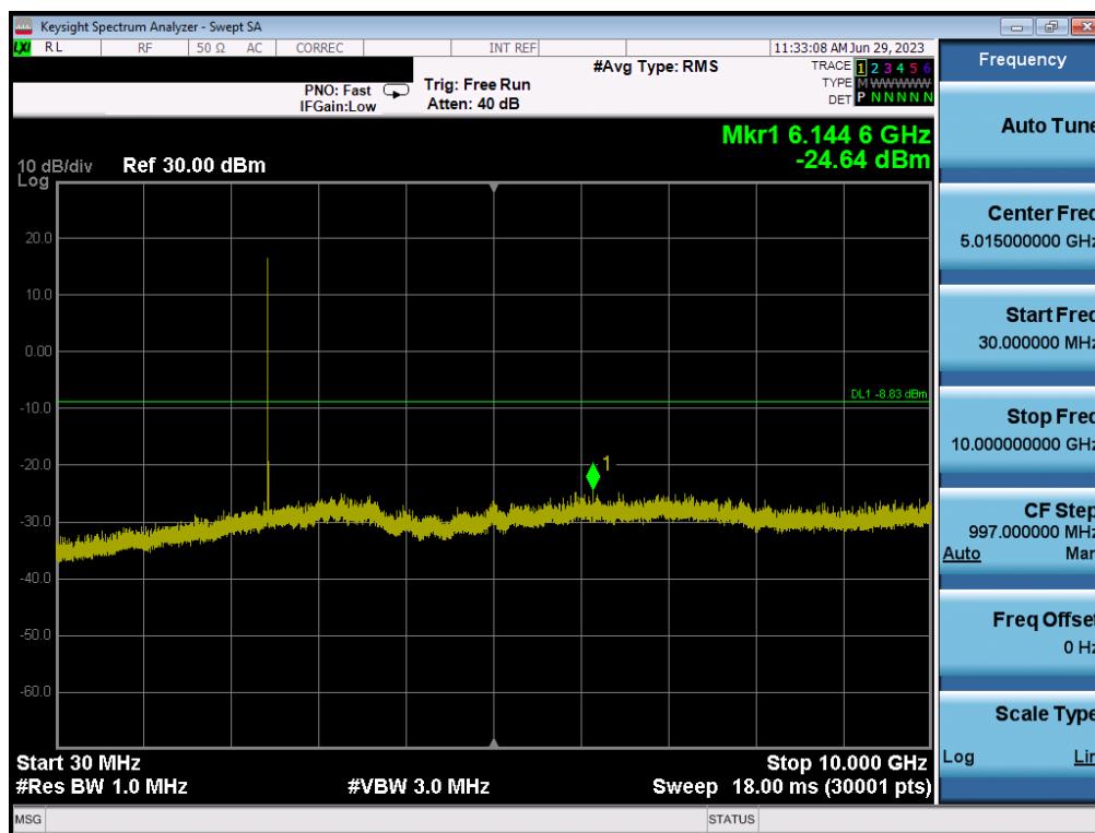
Plot 7-25. Conducted Spurious Plot (Bluetooth (HDR4), 4 Mbps, ePA – Ch. 38)
