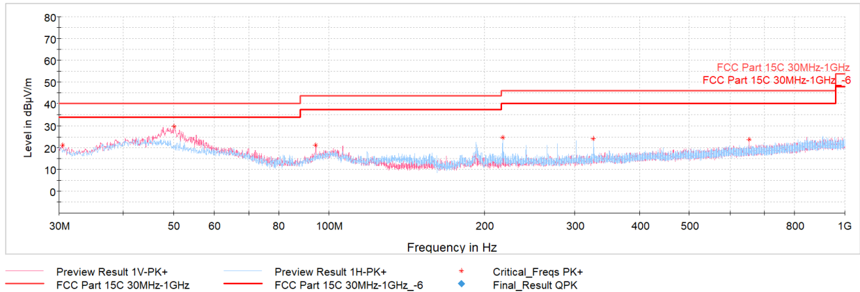
Plot 7-38. Radiated Spurious Emissions Below 1GHz (HDR4 ePA – Ch.38 with AC/DC Adapter + Magnetic Charger)
