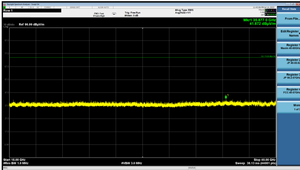
7-33. Radiated Spurious Plot Above 18GHz (4Mbps, HDR4, ePA – Ch.38, Ant. Pol. V)
