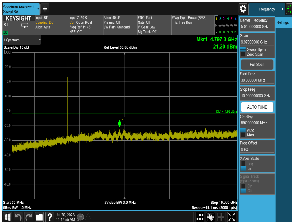
Plot 7-27. Conducted Spurious Plot (Bluetooth (HDR4), 4 Mbps, ePA – Ch. 73)
