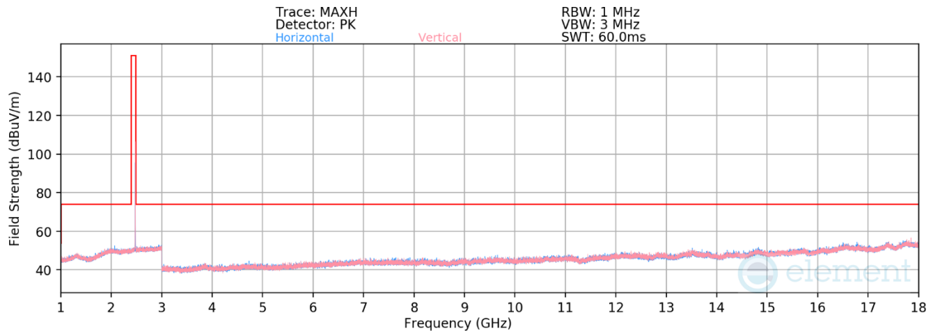
Plot 7-31. Radiated Spurious Emissions 1-18GHz (4Mbps, HDR4, ePA – Ch. 73)
