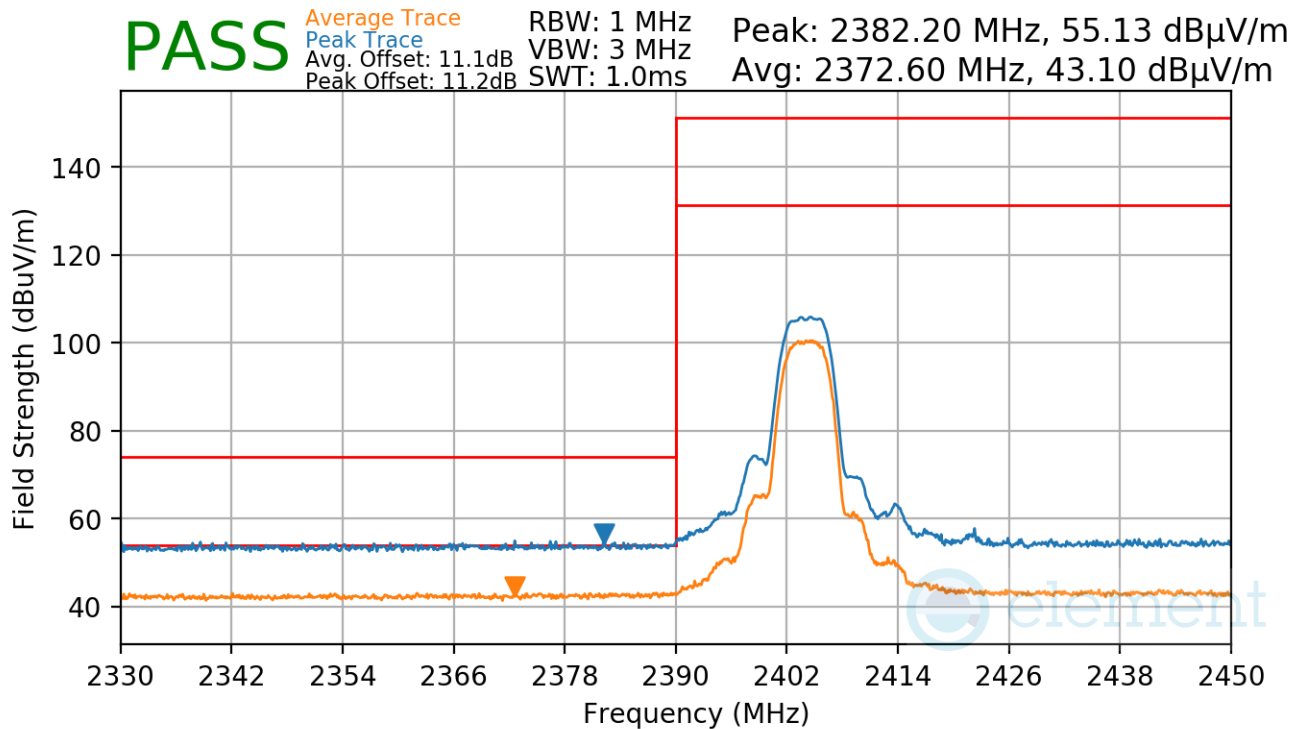
Plot 7-35. Radiated Restricted Lower Band Edge Measurement
