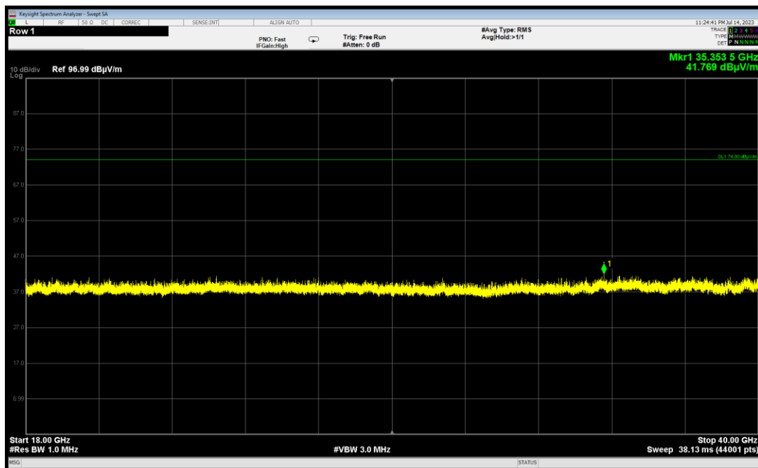
Plot 7-32. Radiated Spurious Emissions above 18GHz (1Mbps, ePA – Ch.39, Pol.H)
