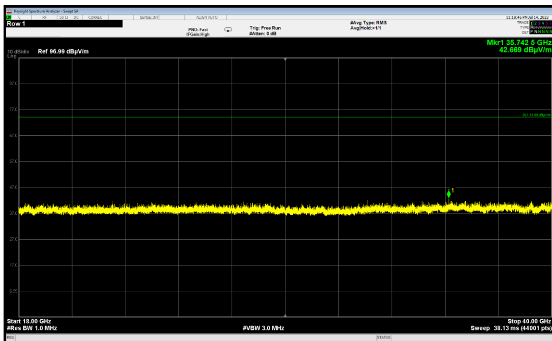
Plot 7-33. Radiated Spurious Emissions above 18GHz (1Mbps, ePA – Ch.39, Pol V)
