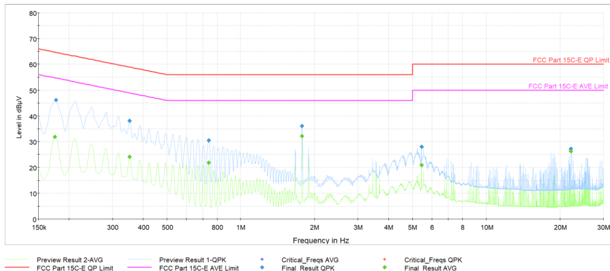
Plot 7-40. AC Line Conducted Plot with Bluetooth LE (N, 1Mbps ePA – Ch.39 with AC/DC Adapter + Magnetic Charger)
