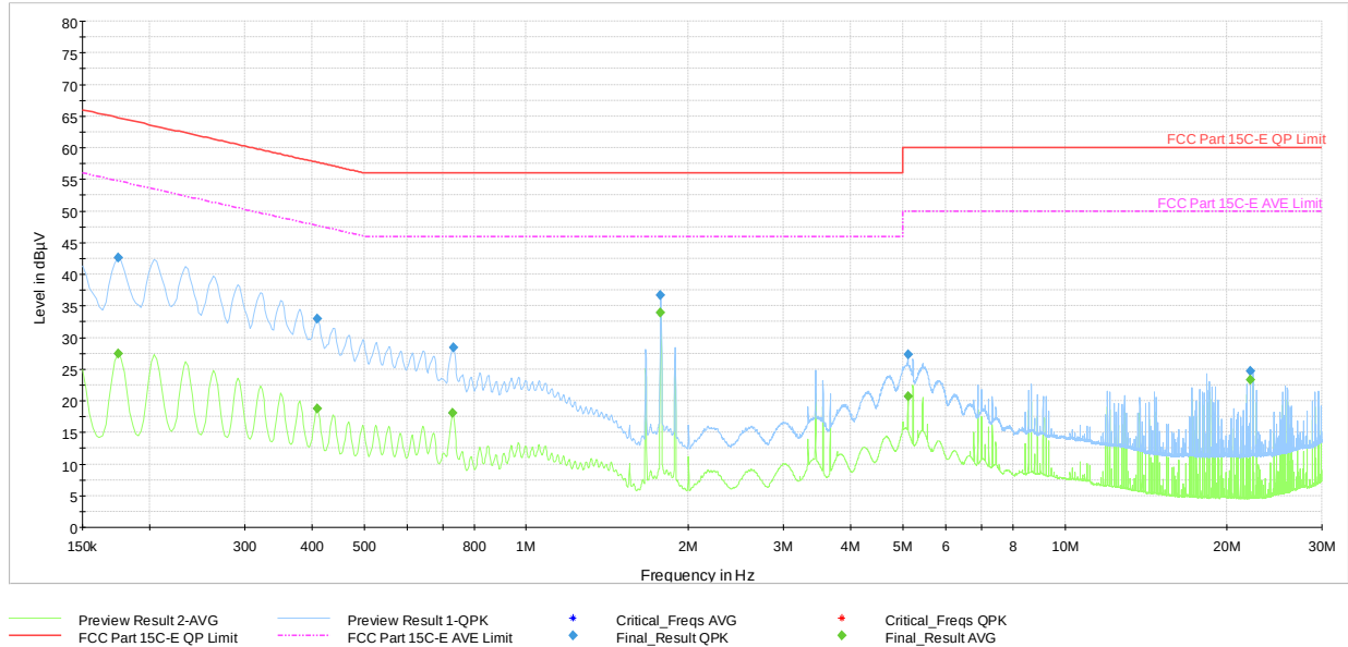
Plot 7-43. AC Line-Conducted Test Plot (L1, GFSK ePA – Ch.39, with AC/DC Adapter + Magnetic Charger)
