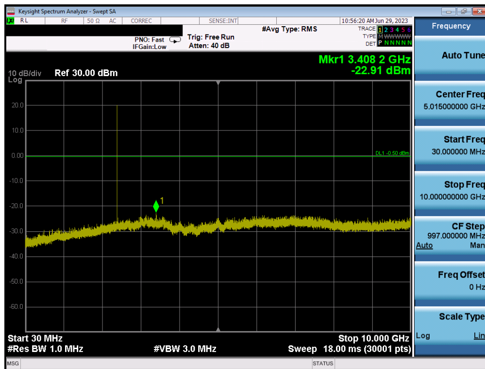
Plot 7-23. Conducted Spurious Plot (Bluetooth, GFSK, ePA – Ch. 0)
