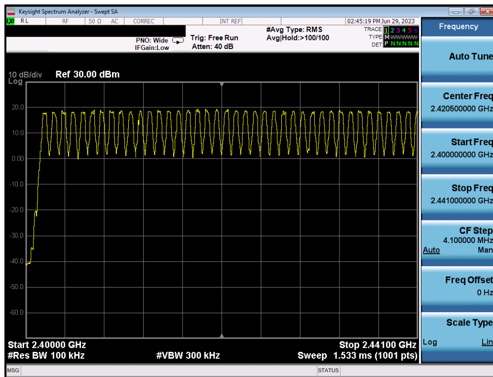
Plot 7-19. Low End Spectrum Channel Hopping Plot (Bluetooth, GFSK, ePA)
