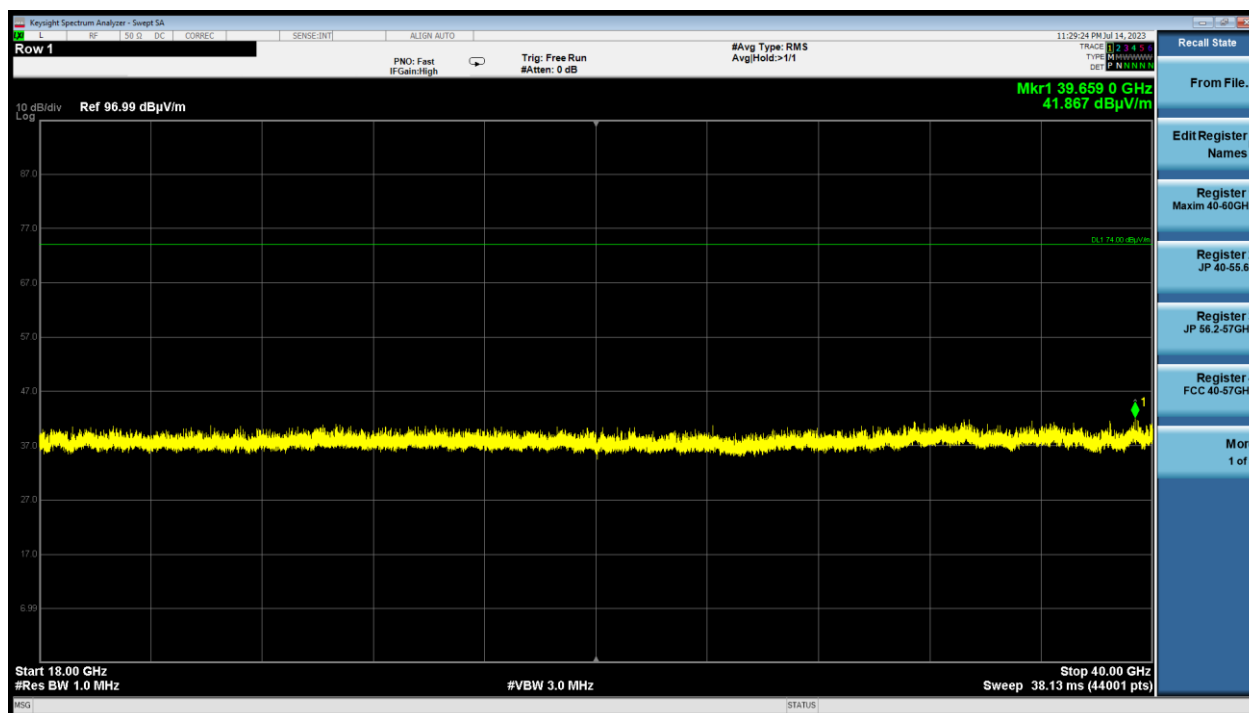
Plot 7-32. Radiated Spurious Emissions above 18GHz (GFSK ePA – Ch.39, Pol. H)
