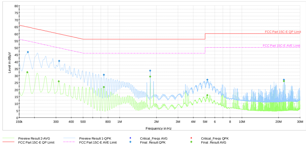
Plot 7-44. AC Line-Conducted Test Plot (N, GFSK ePA – Ch.39, with AC/DC Adapter + Magnetic Charger)
