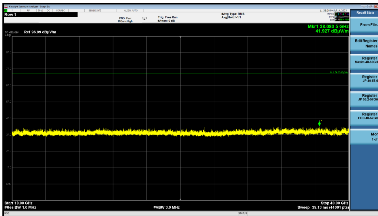
Plot 7-33. Radiated Spurious Emissions above 18GHz (GFSK ePA – Ch.39, Pol. V)
