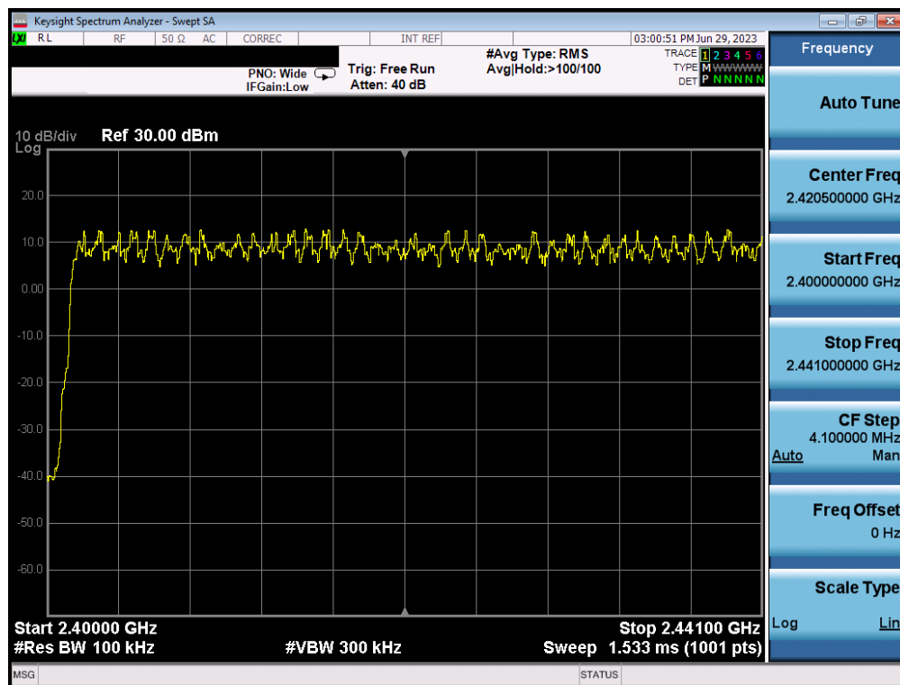
Plot 7-21. Low End Spectrum Channel Hopping Plot (Bluetooth, 8DPSK, ePA)
