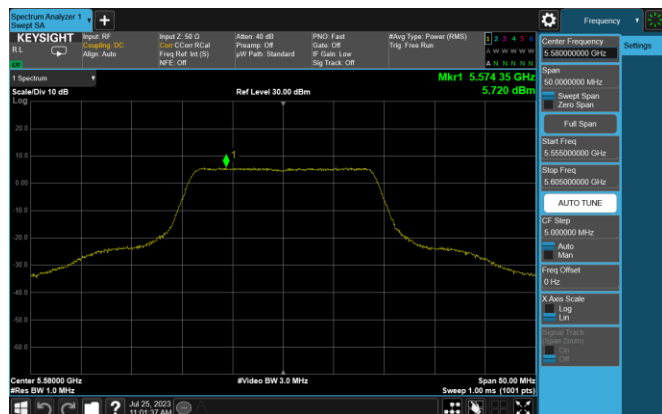
Plot 7-20. PSD (20MHz BW 802.11n – Ch. 116, MCS0)
