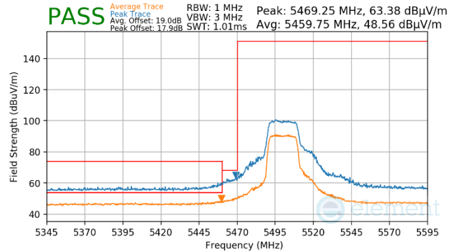
Plot 7-50. (Pk & Avg, Ch.100, 802.11n, MCS7)
