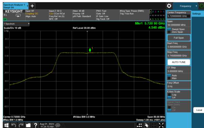
Plot 7-21. PSD (20MHz BW 802.11n – Ch. 144, MCS0)
