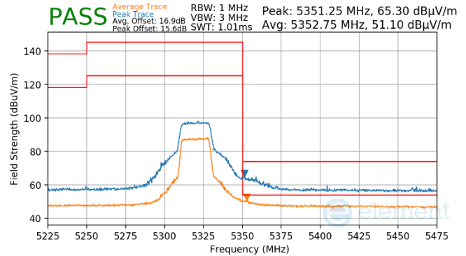
Plot 7-48. (Pk & Avg, Ch.64, 802.11n, MCS7)
