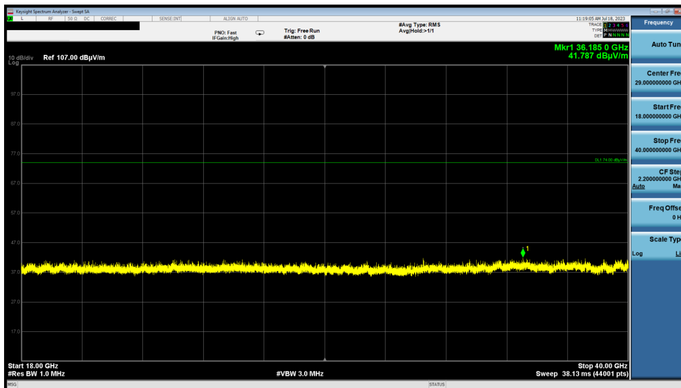
Plot 7-40. Radiated Spurious Emissions 18GHz-40GHz H Polarity (802.11n – Ch. 165)
