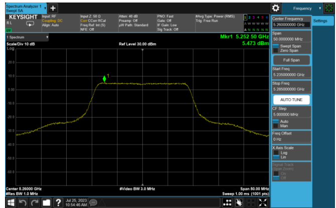
Plot 7-16. PSD (20MHz BW 802.11n - Ch. 52, MCS0)
