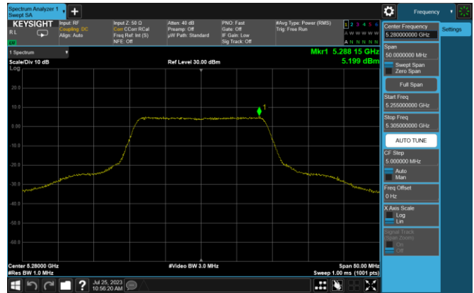
Plot 7-17. PSD (20MHz BW 802.11n - Ch. 56, MCS0)
