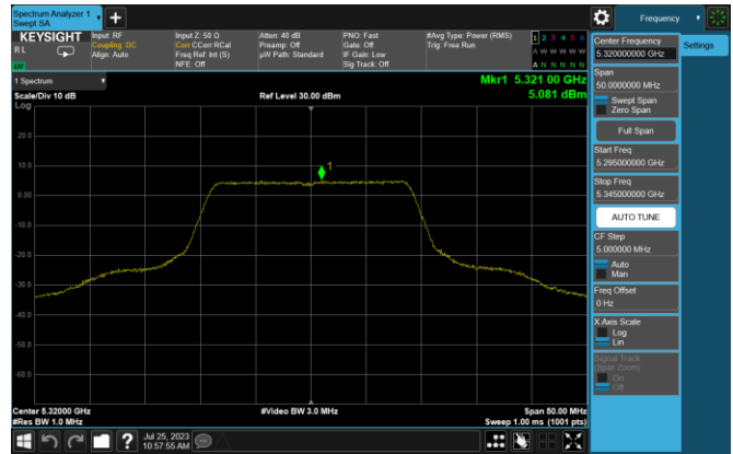
Plot 7-18. PSD (20MHz BW 802.11n - Ch. 64, MCS0)
