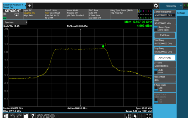
Plot 7-19. PSD (20MHz BW 802.11n – Ch. 100, MCS0)
