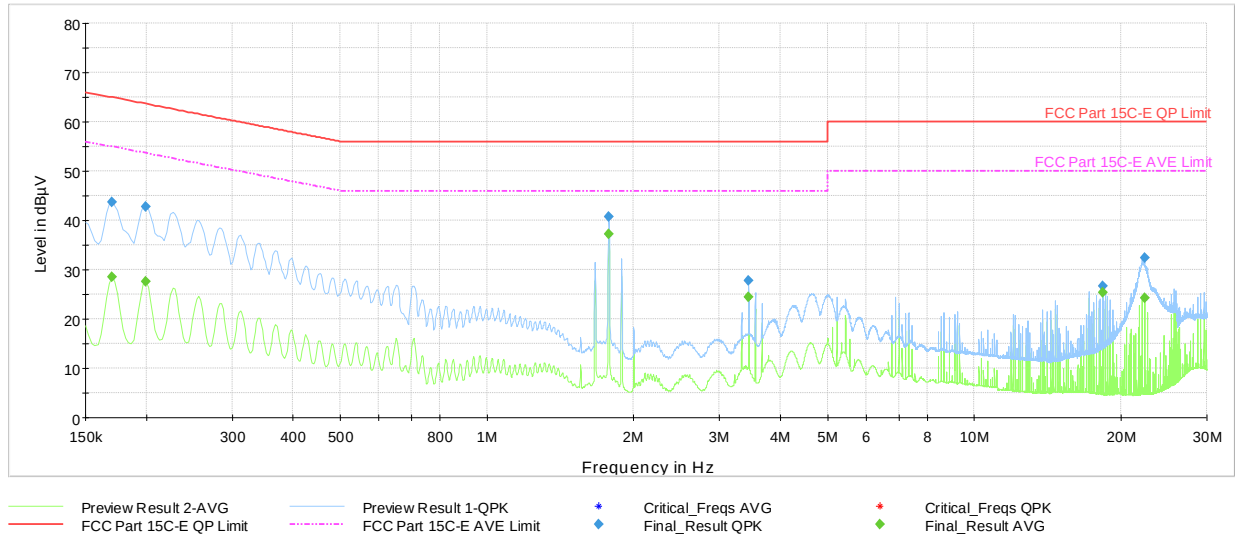
Plot 7-61. AC Line Conducted Plot with 802.11n – Ch.165 (L1), with host PC & magnetic charger
