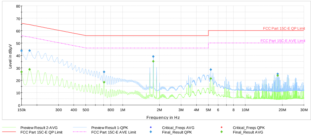
Plot 7-62. AC Line Conducted Plot with 802.11n– Ch.165 (N) with host PC & magnetic charger
