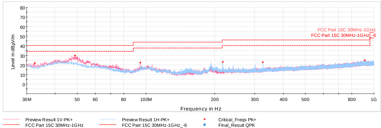
Plot 7-59. Radiated Spurious Emissions below 1GHz, 802.11n, Ch.165 with AC/DC Adapter & magnetic charger
