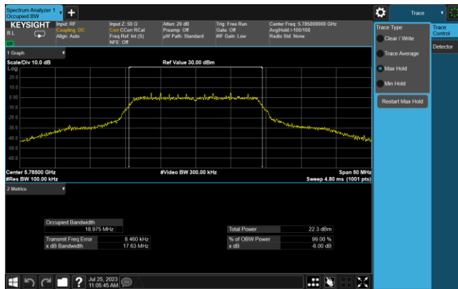
Plot 7-11. 6dB BW & 99% OBW (20MHz BW 802.11n – Ch. 157, MCS0)
