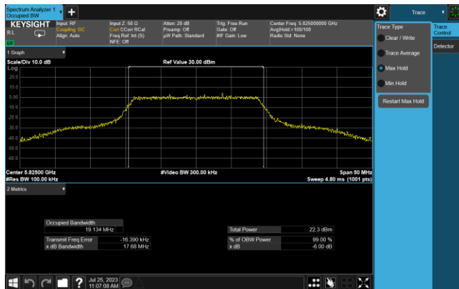
Plot 7-12. 6dB BW & 99% OBW (20MHz BW 802.11n – Ch. 165, MCS0)
