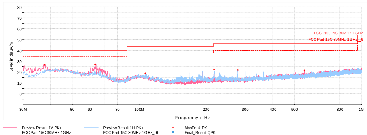
Plot 7-60. Radiated Spurious Emissions – Simultaneous Transmission 30MHz – 1GHz, with AC/DC Adapter & magnetic charger
