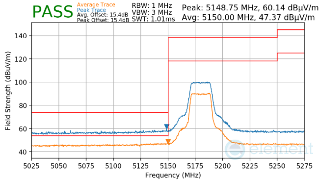
Plot 7-45. (Pk & Avg, Ch.36, 802.11n, MCS0)
