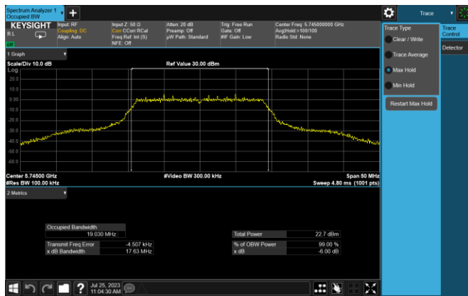
Plot 7-10. 6dB BW & 99% OBW (20MHz BW 802.11n – Ch. 149, MCS0)
