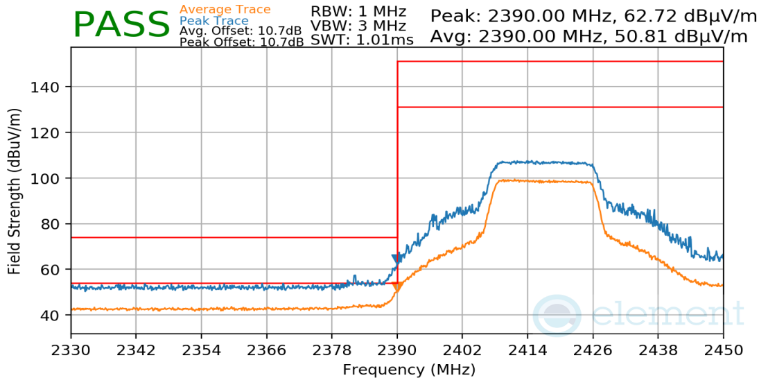
Plot 7-69. Radiated Restricted Lower Band Edge Measurement
