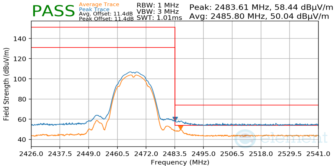
Plot 7-65. Radiated Restricted Upper Band Edge Measurement
