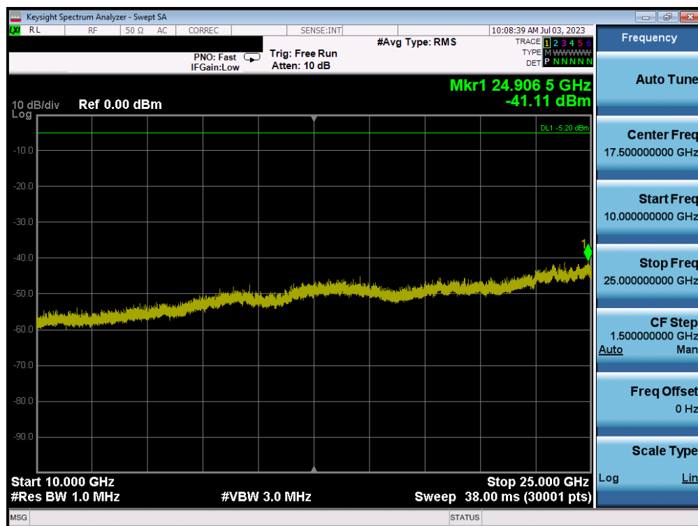
Plot 7-55. Conducted Spurious Plot (802.11b – Ch. 6)
