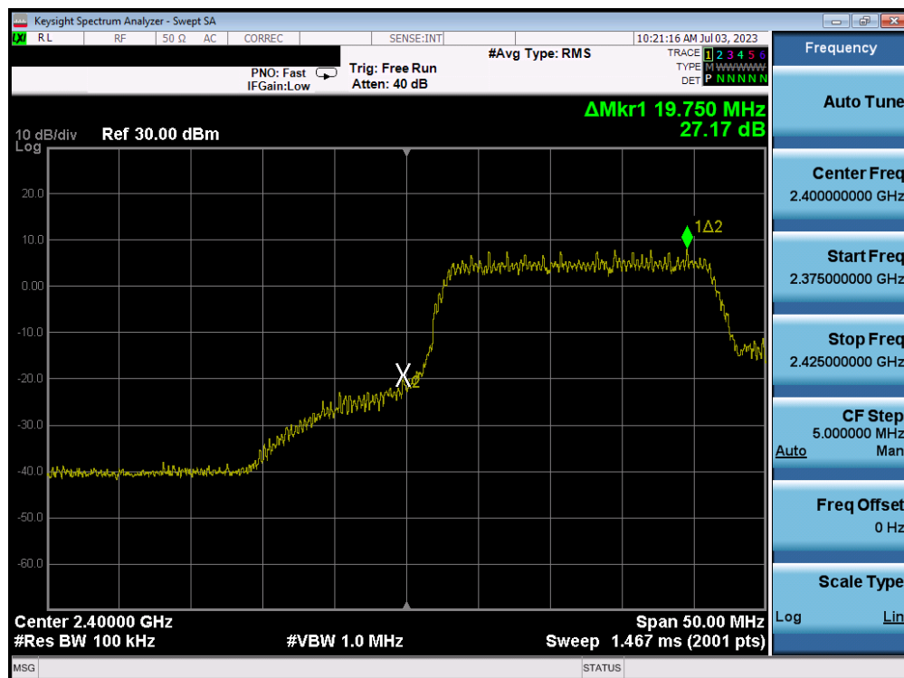
Plot 7-47. Band Edge Plot (802.11n (2.4GHz) – Ch. 1) – MCS7
