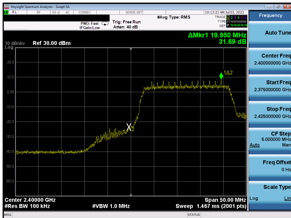
Plot 7-39. Band Edge Plot (802.11n (2.4GHz) – Ch. 2) – MCS0
