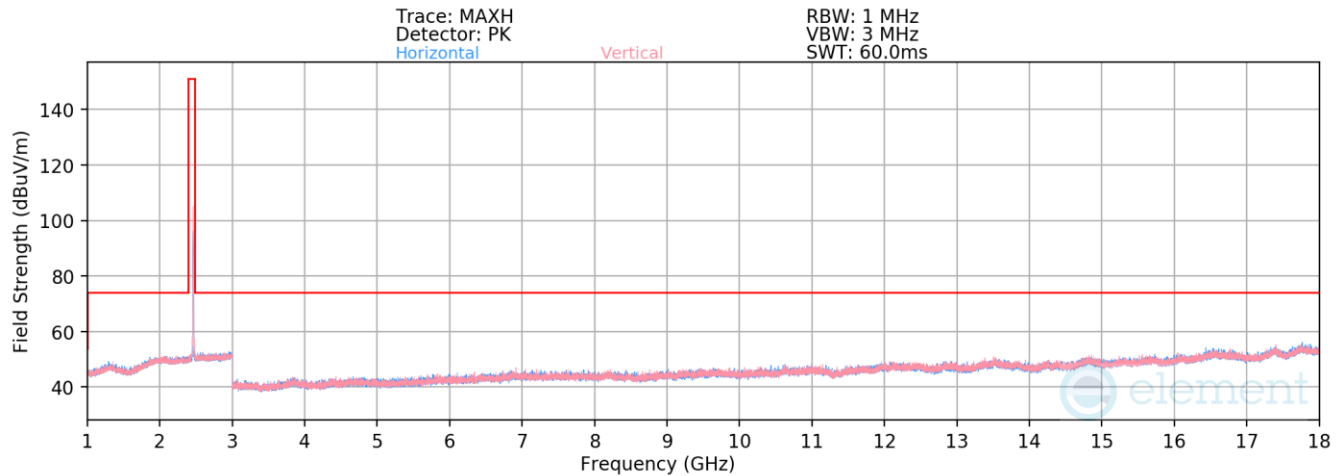
Plot 7-62. Radiated Spurious Emissions above 1GHz (802.11b – Ch. 11)
