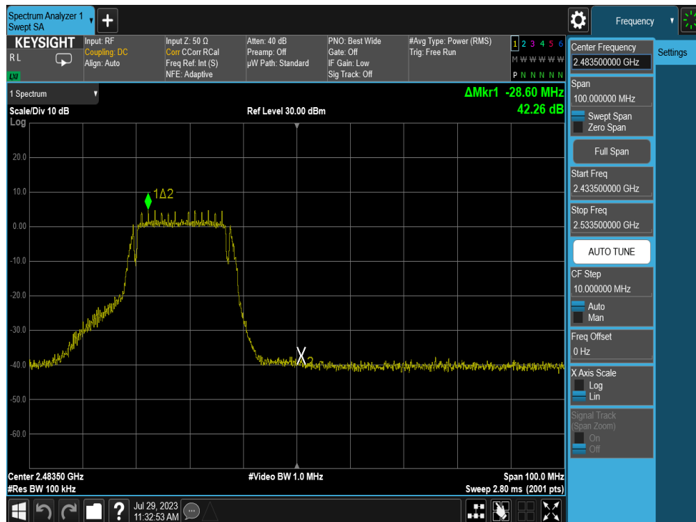
Plot 7-35. Band Edge Plot (802.11g – Ch. 11) – 6Mbps
