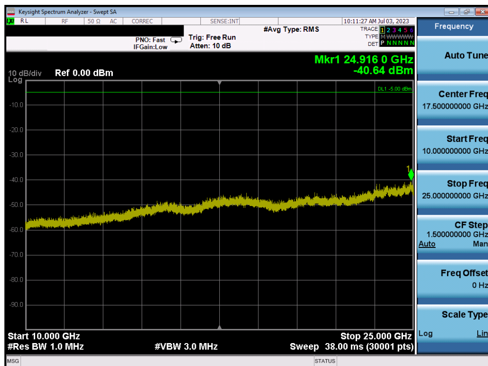
Plot 7-57. Conducted Spurious Plot (802.11b – Ch. 11)
