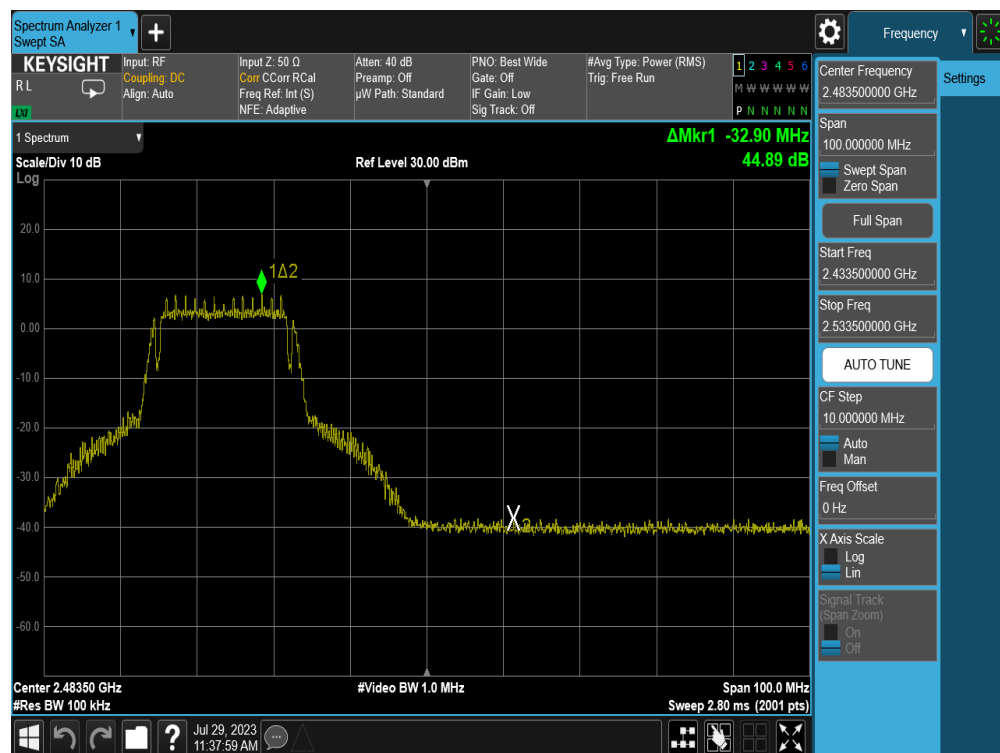
Plot 7-34. Band Edge Plot (802.11g – Ch. 10) – 6Mbps
