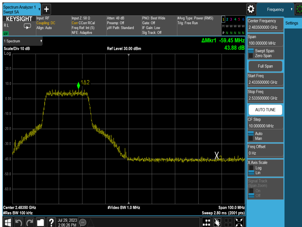
Plot 7-48. Band Edge Plot (802.11n (2.4GHz) – Ch. 10) – MCS7
