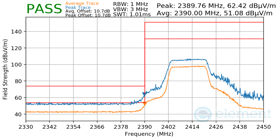
Plot 7-67. Radiated Restricted Lower Band Edge Measurement
