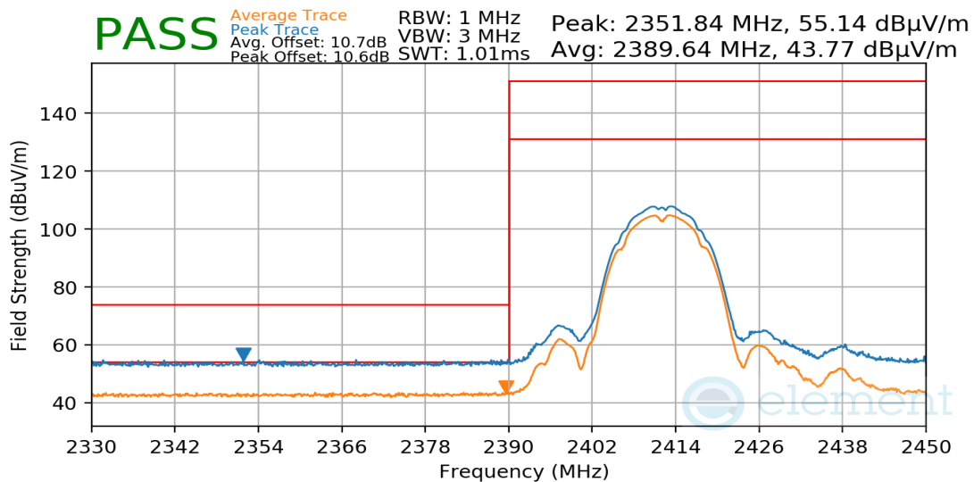
Plot 7-63. Radiated Restricted Lower Band Edge Measurement
