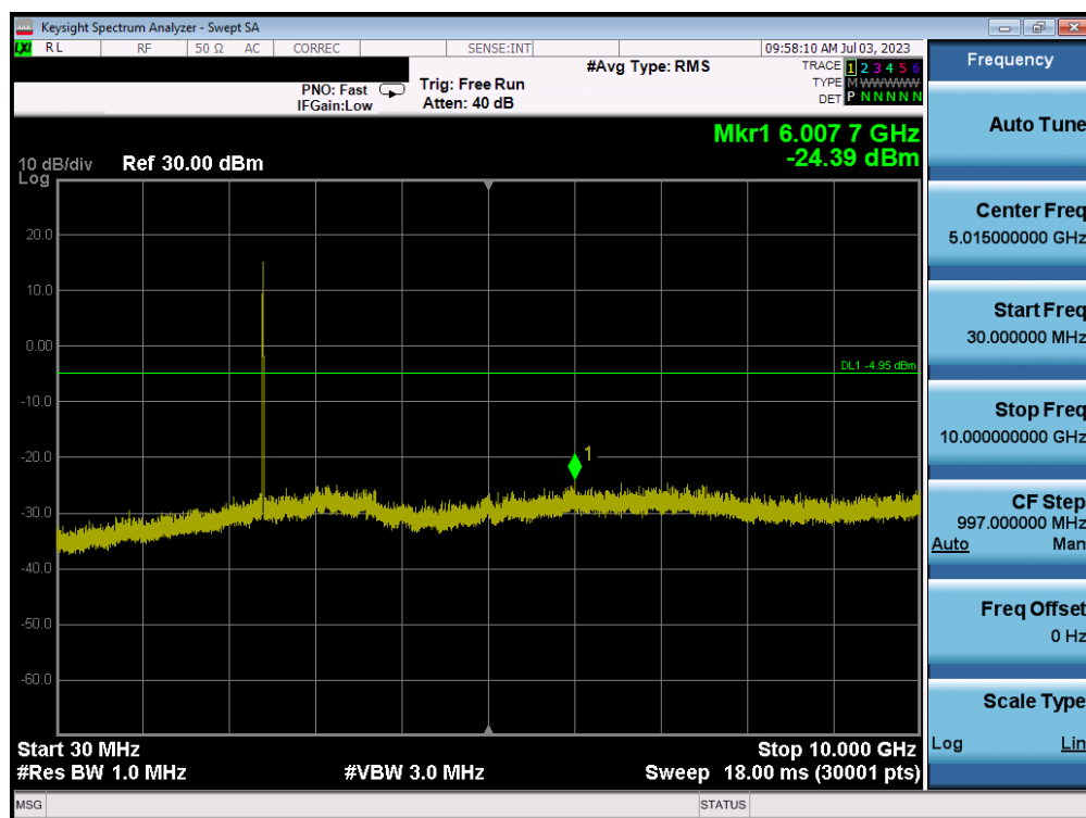
Plot 7-52. Conducted Spurious Plot (802.11b – Ch. 1)
