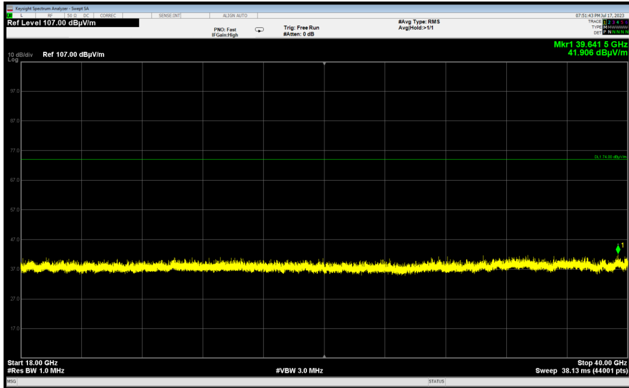
Plot 7-60. Radiated Spurious Emissions Above 18GHz (802.11b – Ch. 6 Pol H)
