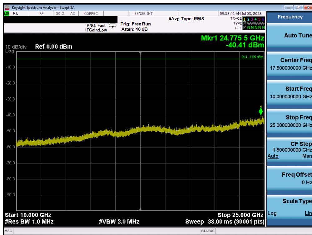
Plot 7-53. Conducted Spurious Plot (802.11b – Ch. 1)
