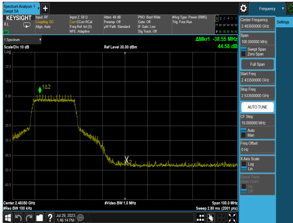
Plot 7-42. Band Edge Plot (802.11n (2.4GHz) – Ch. 9) – MCS0
