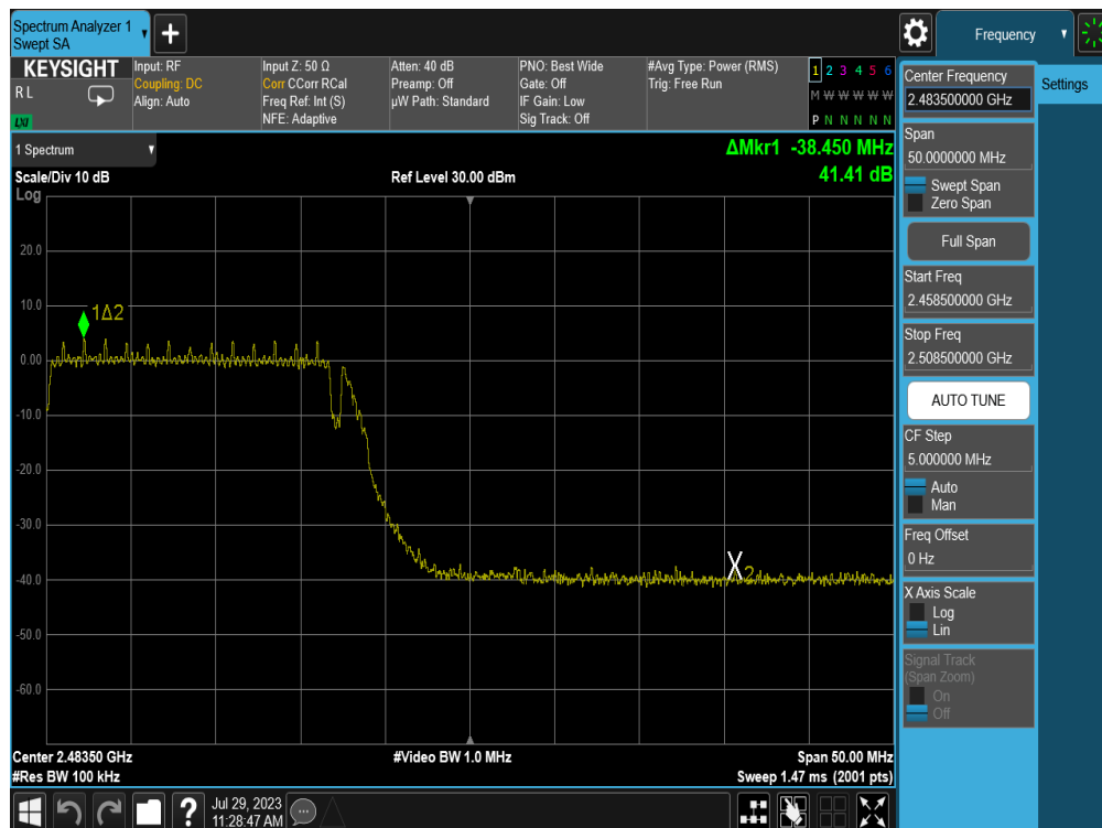
Plot 7-36. Band Edge Plot (802.11g – Ch. 12) – 6Mbps
