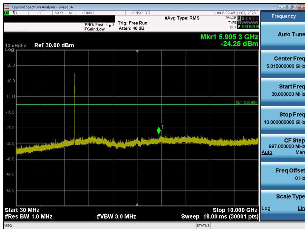
Plot 7-54. Conducted Spurious Plot (802.11b – Ch. 6)
