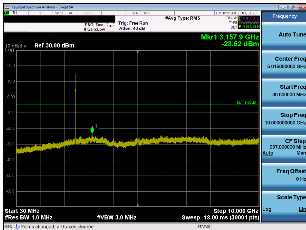
Plot 7-56. Conducted Spurious Plot (802.11b – Ch. 11)
