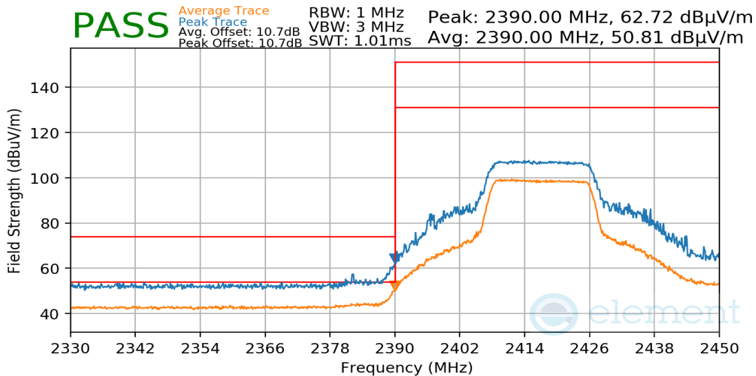
Plot 7-68. Radiated Restricted Lower Band Edge Measurement
