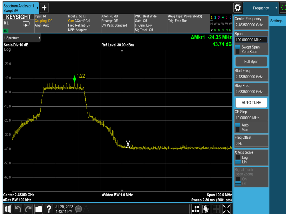
Plot 7-43. Band Edge Plot (802.11n (2.4GHz) – Ch. 10) – MCS0
