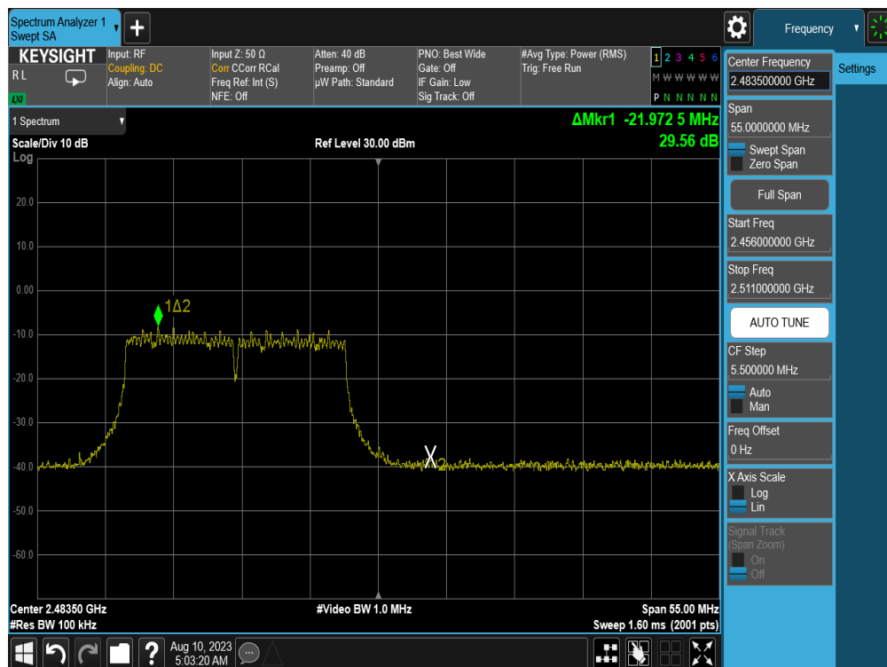
Plot 7-51. Band Edge Plot (802.11n (2.4GHz) – Ch. 13) – MCS7
