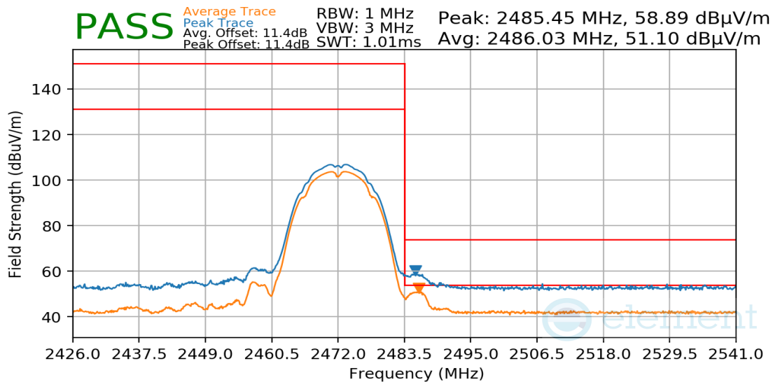
Plot 7-66. Radiated Restricted Upper Band Edge Measurement
