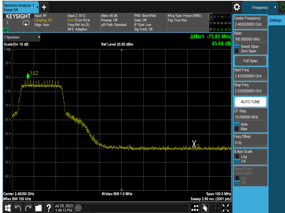
Plot 7-41. Band Edge Plot (802.11n (2.4GHz) – Ch. 8) – MCS0
