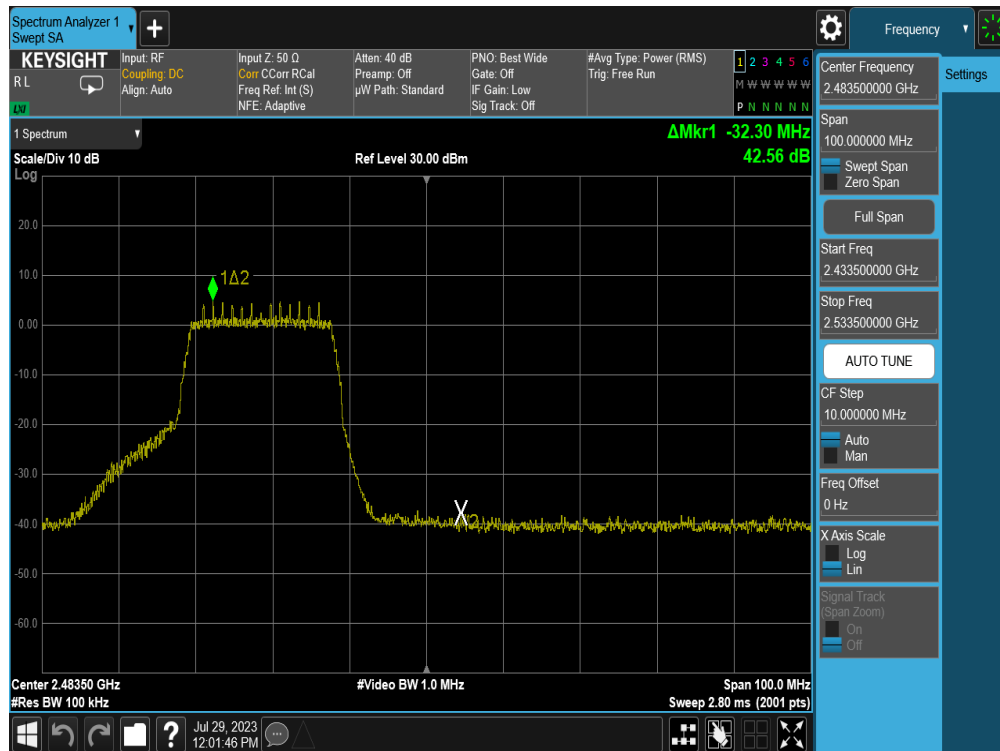
Plot 7-44. Band Edge Plot (802.11n (2.4GHz) – Ch. 11) – MCS0
