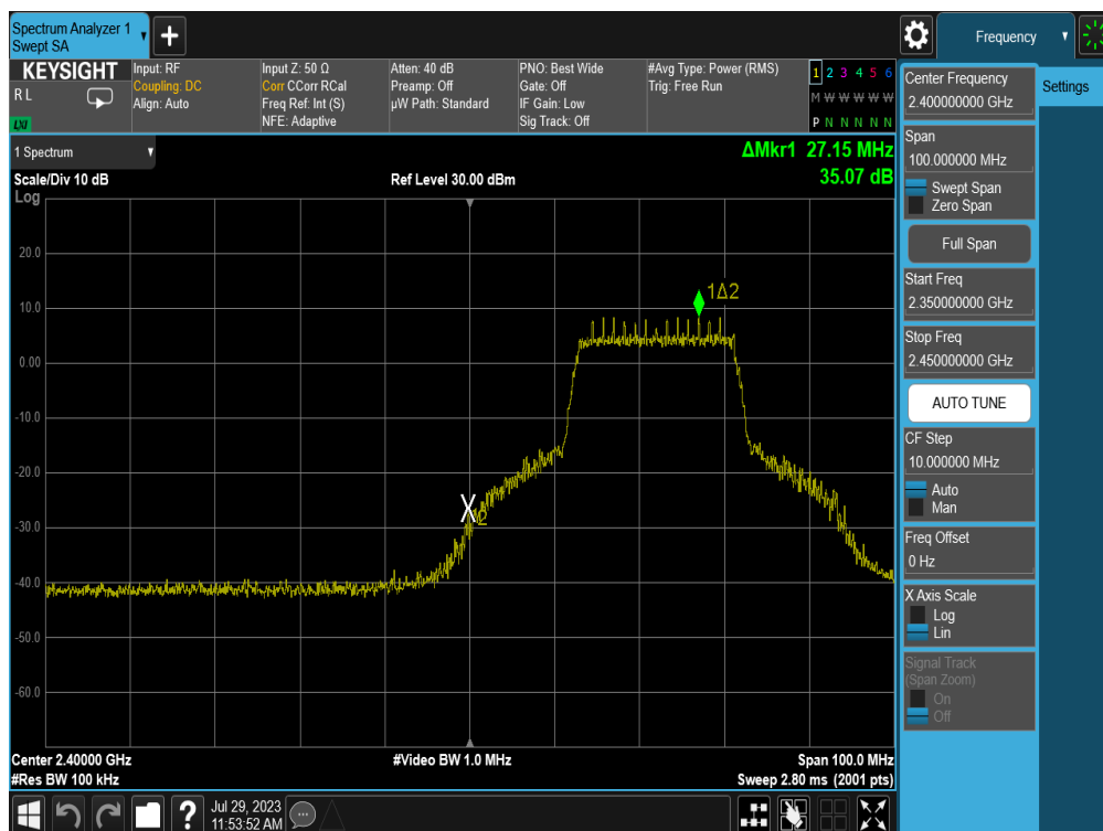
Plot 7-40. Band Edge Plot (802.11n (2.4GHz) – Ch. 3) – MCS0
